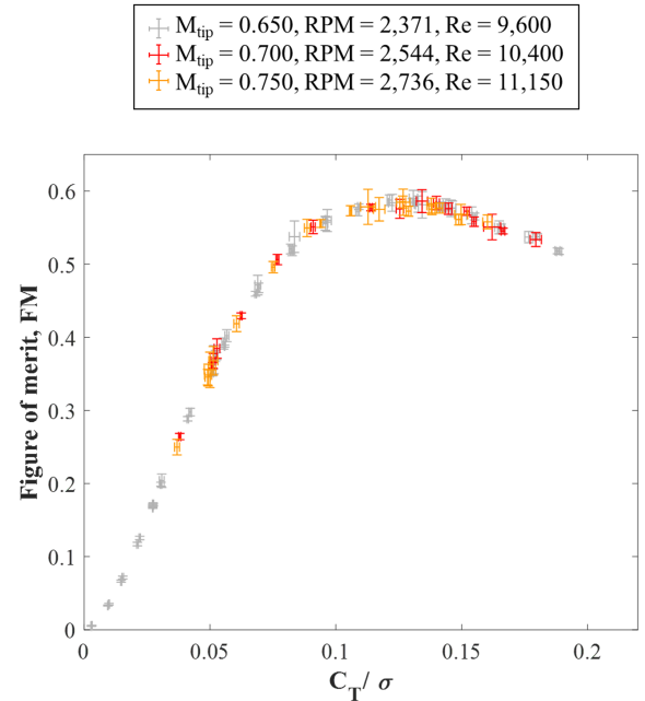
Figure 16. Figure of merit versus blade loading for DRT coaxial rotor configuration with uncertainty at \rho = 0.0185 kg/m 3 .
