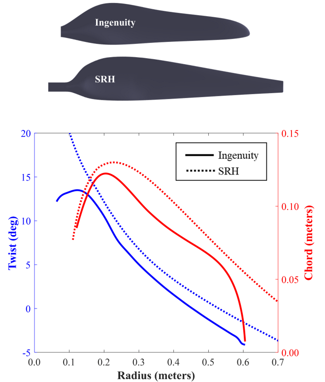
Figure 2. Ingenuity and SRH blade geometry specifications.
