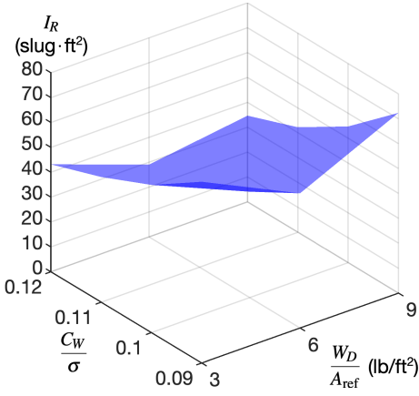
Figure 7. Hexacopter rotor moment of inertia.
