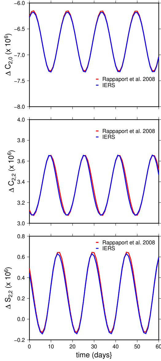
Supplementary Figure 8: Time-varying changes due to tides in the un-normalized degree 2 coefficients C_{2,0} (top), C_{2,2} (middle), and S_{2,2} (bottom) using either a simplified potential 12 or the full expression 30 , for 60 days in 2006.
