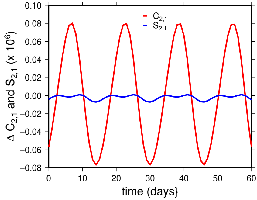
Supplementary Figure 9: Time-varying changes due to tides in the un-normalized degree 2 coefficients C_{2,1} and S_{2,1} , from the full potential 30 . The variations are much smaller than those in the other degree 2 coefficients.
