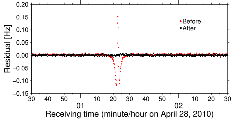
Supplementary Figure 6: Doppler residuals from Deep Space Network station DSS-55 for Enceladus flyby 009, before and after gravity field estimation. The closest approach signal is clearly visible in the pre-gravity determination residuals. The residuals after gravity estimation resemble measurement noise.
