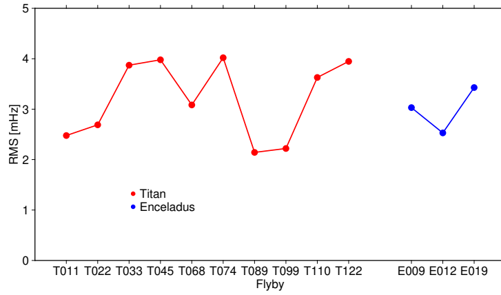
Supplementary Figure 7: Root-mean-square of Doppler data fit after gravity field determination for flybys for Titan (left/red) and Enceladus (right/blue).
