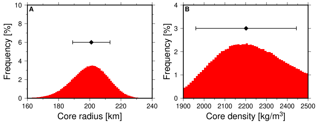
Supplementary Figure 13: A posteriori distributions (including the central value \pm 1 standard deviation) of the core radius (left) and core density (right) for Enceladus as results from our Monte Carlo analysis to match the moment of inertia and bulk density. We evaluated 100,000 models using 40 chains.
