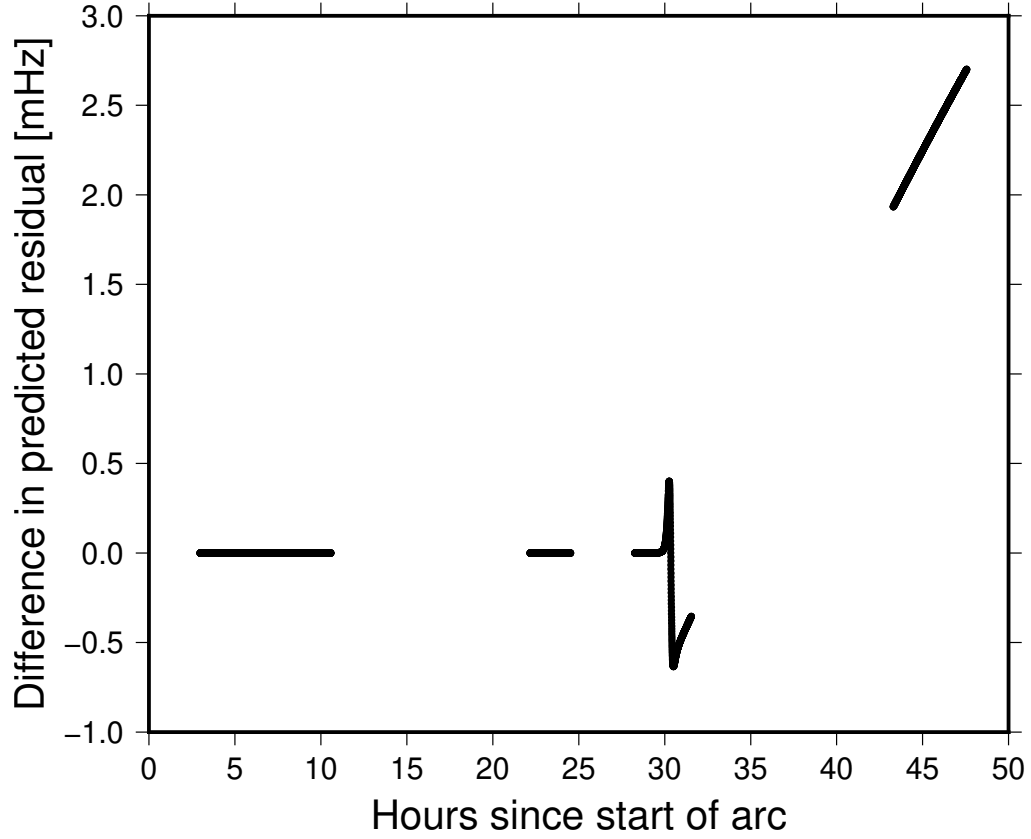
Supplementary Figure 12: Differences in residuals between those predicted by the variational partials (eq. 17) and those predicted by the non-variational partials (eq. 12) for Cassini flyby T022, using a \Delta k_2 of 0.25. These are constructed using the partials shown in Supplementary Figure 10.
