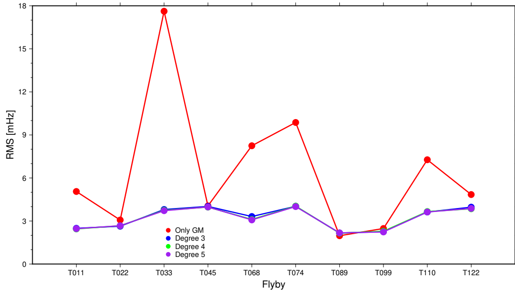
Supplementary Figure 3: Root-mean-square of Doppler data fit after gravity field determination for flybys for Titan for various expansions of the estimated gravity field. The entry labeled "Only GM" used the start value for GM with all other gravity terms set to zero. This shows that the fit did not change much when expanding from degree and order 3 up to 5.
