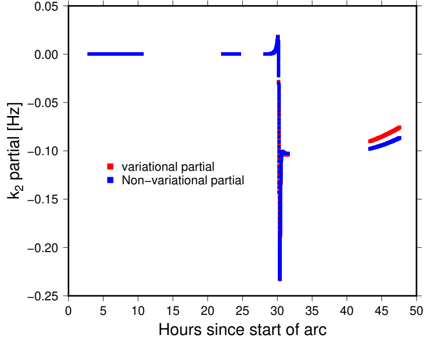
Supplementary Figure 10: Partials of Doppler data for Cassini flyby T022 with respect to k_2 , directly computed using the full variational approach, or using the non-variational approach from eq. (12). We used the full IERS expressions, not the simplified potential 12 , in order to have the exact same partials \partial\nu_{2,m}/\partial k_2 .
