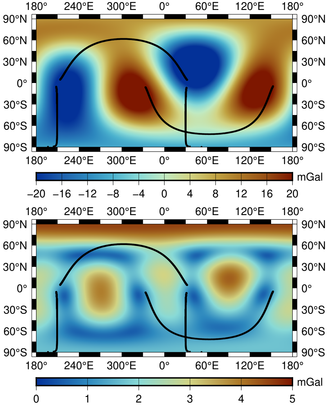
Supplementary Figure 2: Gravity expressed as radial accelerations for Enceladus (top) and formal errors from the full covariance matrix of our solution (bottom), both for the degree and order 2 field including the zonal term \bar{C}_{3,0} . The ground tracks of the flybys are indicated in black for altitudes less than 3,000 km. We set the coefficients C_{2,0} and C_{2,2} to zero for the gravity map.
