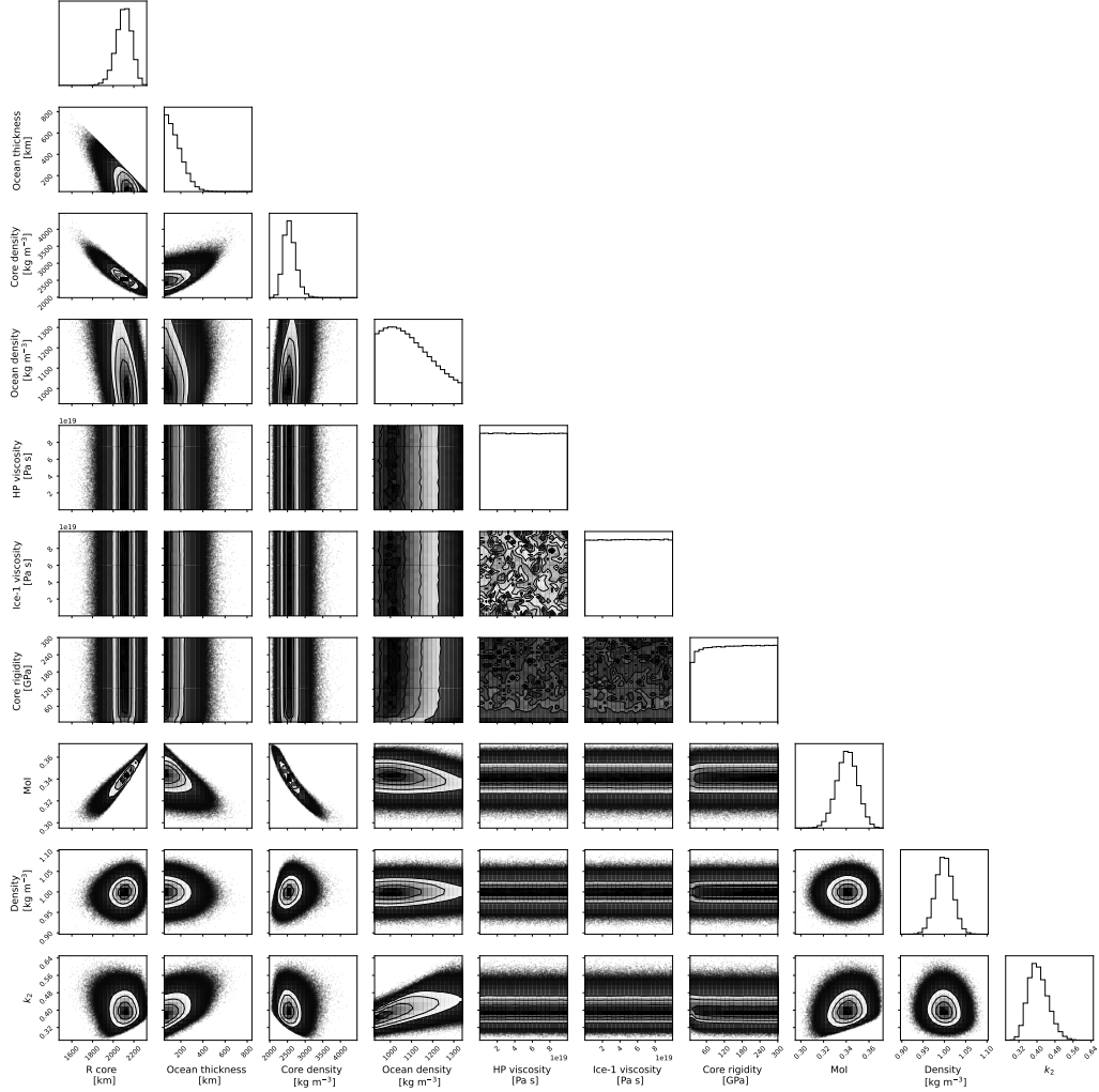
Supplementary Figure 5: Triangle plot of the distributions of the parameters and measurements for our Titan analysis using MCMC. Only a few parameters are well-determined as indicated by the distributions. The measurements are mapped well. This Figure is also available as a separate file. This figure was made with the Python package “corner” 45 .
