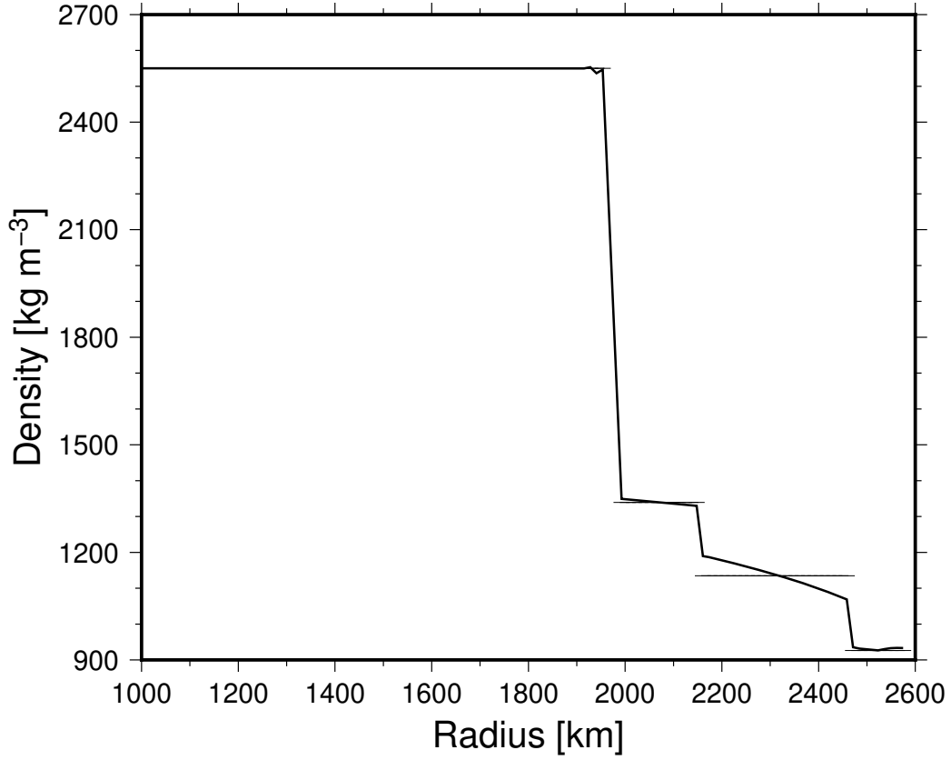
Supplementary Figure 4: Example of a density profile for the hydrosphere, using a pure water ocean with a temperature of 257 K at the base of the icy crust 31 . The core density is kept constant. We compared the tidal response of this density profile to that of a profile with constant densities, where the constant densities are the average densities in each layer of the hydrosphere. These constant densities are also indicated in the Figure.
