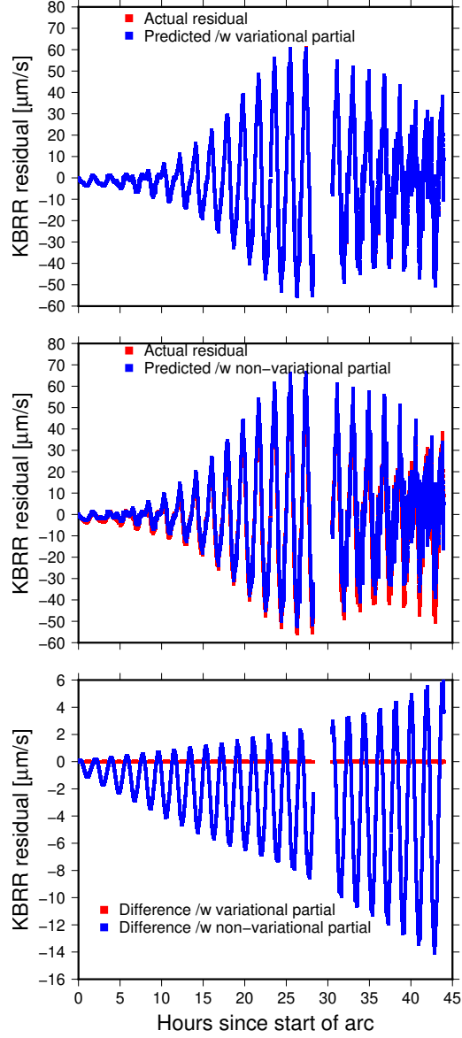
Supplementary Figure 11: Comparison of residual changes and those predicted from the partials, following eq. (11), for an arc for GRAIL Ka-Band Range-Rate (KBRR) data in April, 2012. We compare actual differenced residuals with the change in measurements as predicted by the partials for the case using the full variational approach (top) and for the case with the non-variational approach (middle). The difference between predicted and actual residual changes for both cases are shown in the bottom plot.
