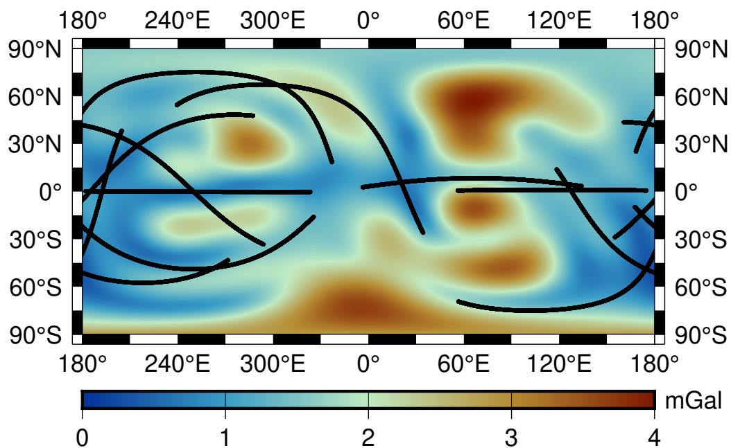
Supplementary Figure 1: Gravity formal errors for Titan from the full covariance matrix up to and including degree 5 of our solution. The ground tracks of the flybys are indicated in the same way as in Figure 1 of the main text.
