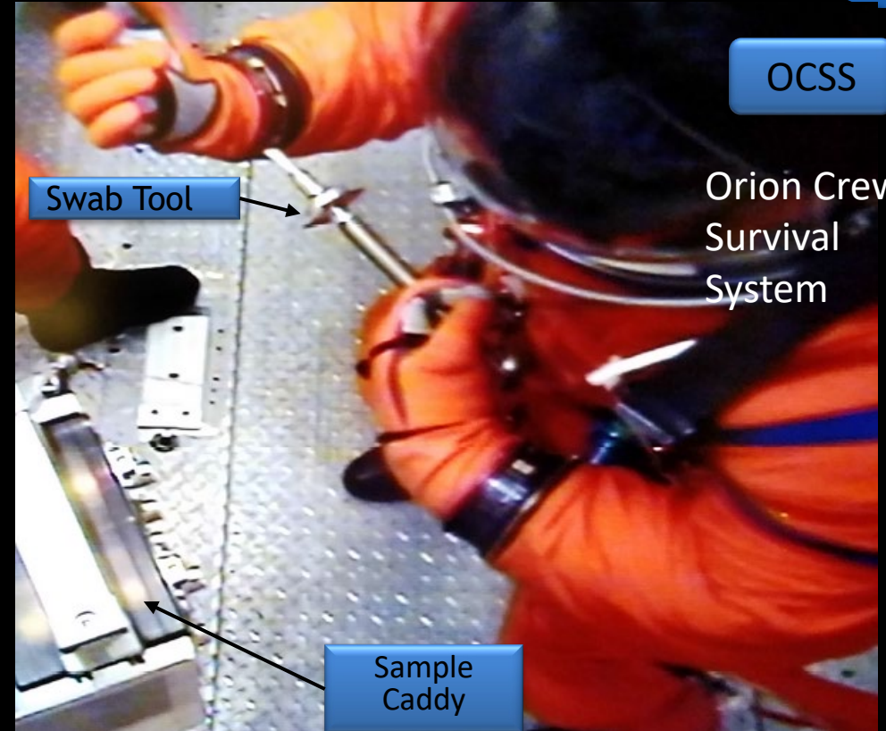
Sampling suit at vacuum in the 11 ft. chamber at Johnson Space Center Internal suit pressure is 4.2 psia 29.6 Kpa)
