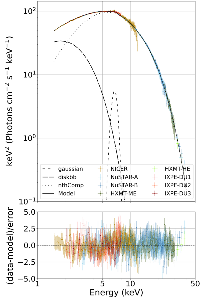
Figure 7. Spectral energy distribution of Sco X-1 in E_F representation. The points show the data from NICER (brown), NuSTAR (blue), Insight-HXMT (green), and IXPE (red). The different spectral model components are reported with black lines for diskbb (long-dashed), nthcomp (dotted), and gauss (short-dashed). The bottom panel shows the residuals between the data and the best-fit model A.
