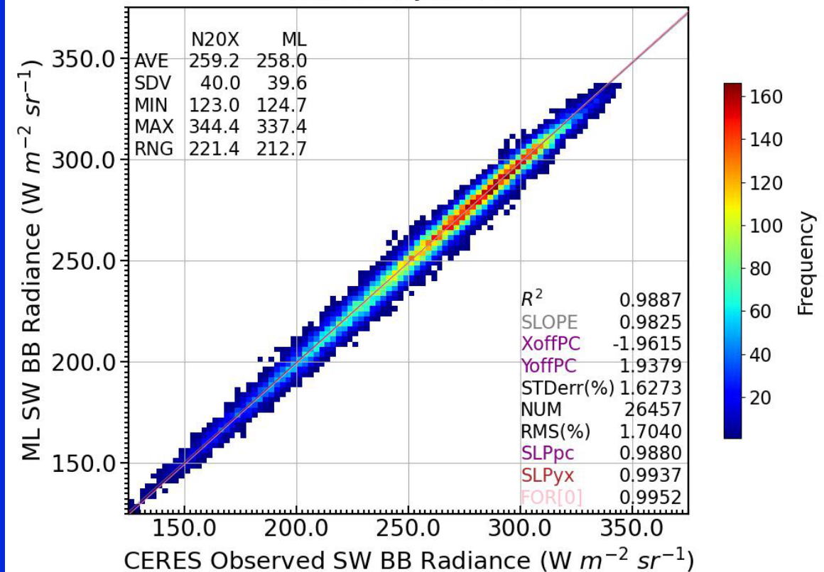
CERES N20X vs ML Predictions noIR DCC Jan 2019
