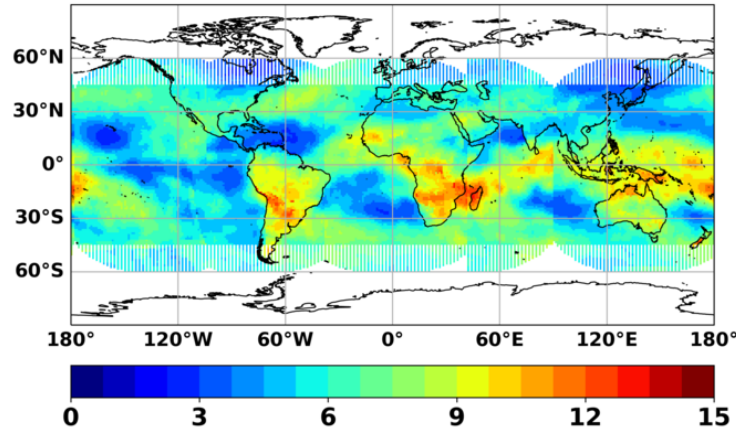
GEO vs. Terra-Aqua-MODIS 201901 LW RMS before Normalization
