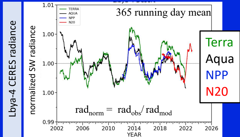
Terra/Aqua/NPP/N20 relative ratios
