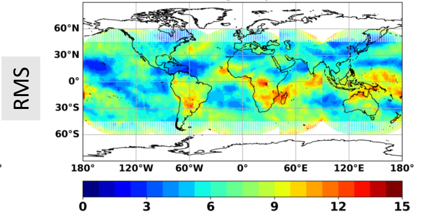
GEO vs. Terra-Aqua-MODIS 201901 LW RMS before Normalization Night Only
