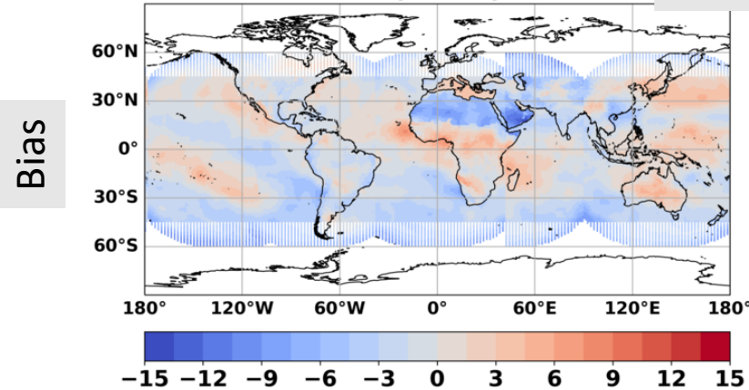
GEO vs. Terra-Aqua-MODIS 201901 LW BIAS before Normalization Daytime Only
