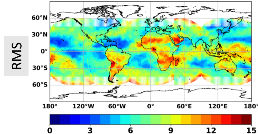
GEO vs. Terra-Aqua-MODIS 201901 LW RMS before Normalization Daytime Only
