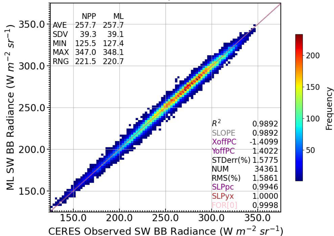
CERES NPP vs ML Predictions noIR DCC Jan 2019
