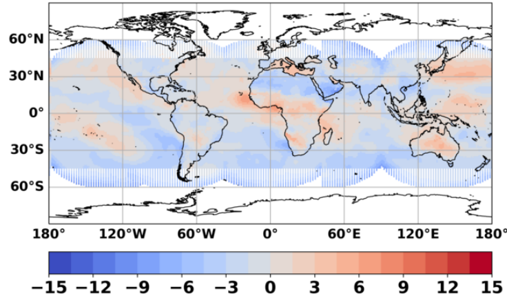
GEO vs. Terra-Aqua-MODIS 201901 LW BIAS before Normalization
