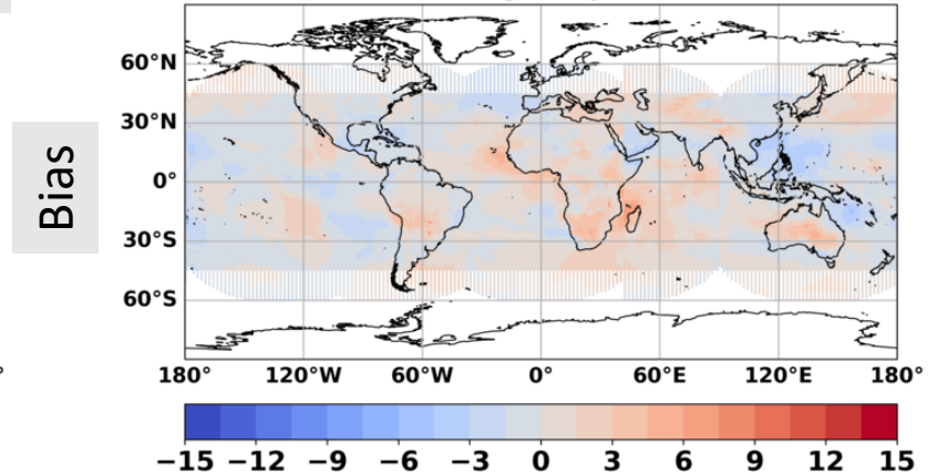
GEO vs. Terra-Aqua-MODIS 201901 LW BIAS before Normalization Night Only
