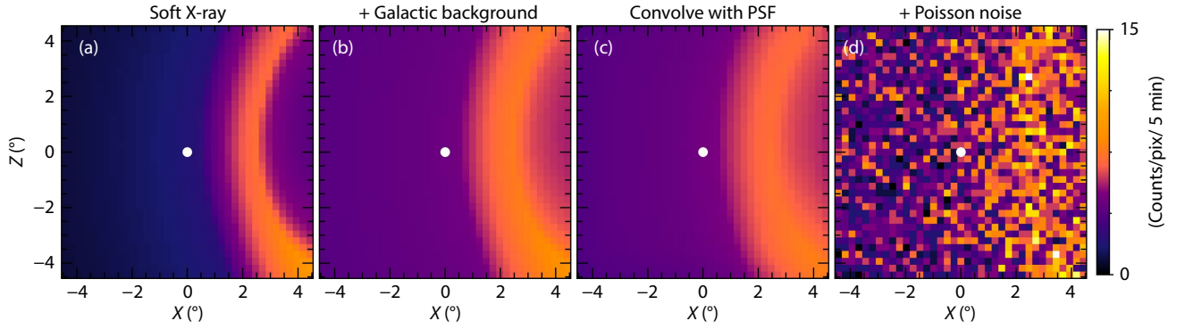
Figure 3. Imaging process used to construct a synthetic LEXI soft X-ray image.
