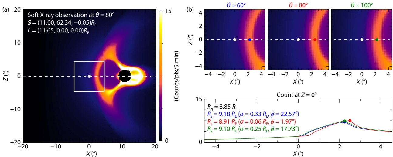
Figure 2. Ideal soft X-ray images from LEXI created with the OpenGGCM MHD model. Images are made with a pixel size of 0.25^\circ \times 0.25^\circ and a exposure time of 5 min. (a) Global image in a large FOV. The white dot and square indicate the LEXI look direction \mathbf{L} and FOV, respectively. (b) Top: Soft X-ray images in the LEXI FOV ( 9.1^\circ \times 9.1^\circ ) at different locations ( \theta and \mathbf{S} ). The white dashed line is the Sun–Earth line, where Z = 0^\circ , and the colored dots indicate the angle of the soft X-ray peak emission ( \alpha ). Bottom: Soft X-ray count rate along the white dashed Sun–Earth lines labeled with the subsolar magnetopause position ( R_g ), the accuracy ( \sigma ), and the angle of the LEXI– R_s line estimated from a line perpendicular to the Sun–Earth line ( \phi ).
