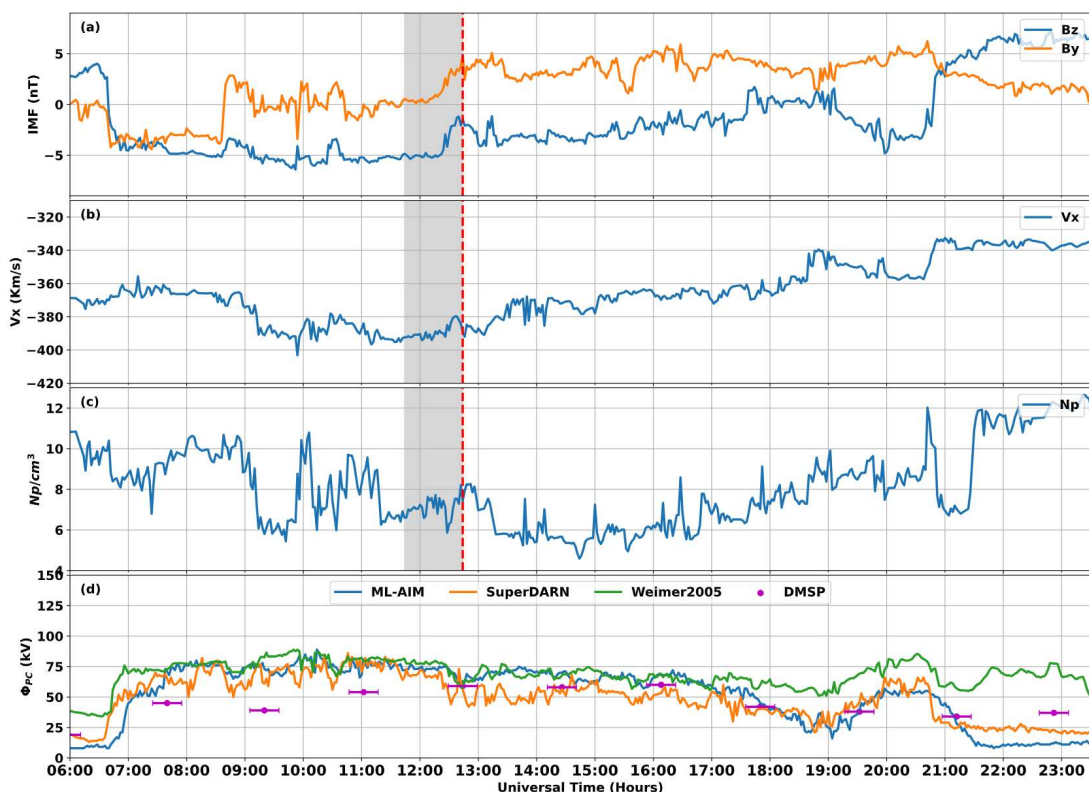
Figure 3. (a) IMF B_z and B_y , (b) solar wind velocity V_x in the Geocentric Solar Magnetospheric coordinates, and (c) number density obtained from the NASA OMNI data during 14 May 2013. The bottom panel shows the cross polar cap potential drop ( \Phi_{PC} ) of the northern hemisphere predicted by the ML-AIM (blue), Weimer (2005) (green), and SuperDARN potential models (orange). Magenta circles indicate the \Phi_{PC} calculated from each polar crossing of Defense Meteorological Satellite Program (DMSP) F17. Time taken for each polar crossing of DMSP is indicated using the horizontal magenta bars. A vertical dashed line and a shaded area indicate the prediction time used in Figure 2 (i.e., 12:44 UT) and the corresponding input period for the prediction (i.e., 11:44–12:44 UT), respectively.
