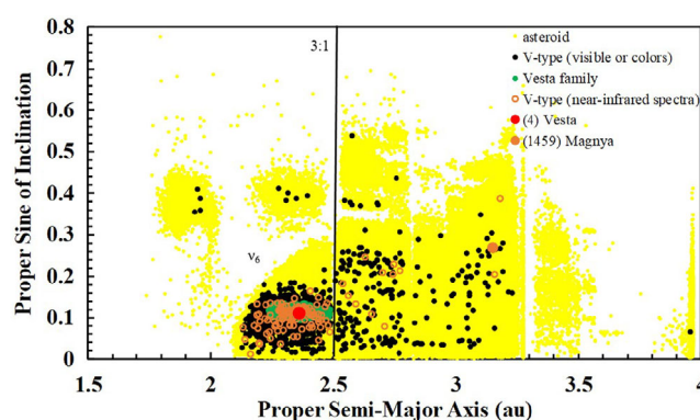
FIGURE 4. Plot of proper sine of inclination versus proper semi-major axis (au) for all asteroids (yellow dots; Novaković et al., 2022), V-types (black dots) that have been identified by various visible spectra surveys or visible or near-infrared color surveys with no near-infrared spectral data, Vesta family members (green dots) (Nesvorný, 2015), Vesta (red filled circle), V-types that have near-infrared spectra consistent with an HED-like mineralogy (orange open circles), and Magnya (orange filled circle). Our V-types include objects with HED-like visible spectra or colors that have been classified as either V-types, J-types, or V_p -types. The plotted Vesta family members have been identified just by dynamical criteria since most of the ~15,000 family members have not been classified since they have not been observed as part of spectral or color surveys. The v_6 secular resonance at the inner edge of the belt and the 3:1 mean-motion resonance are also identified.
