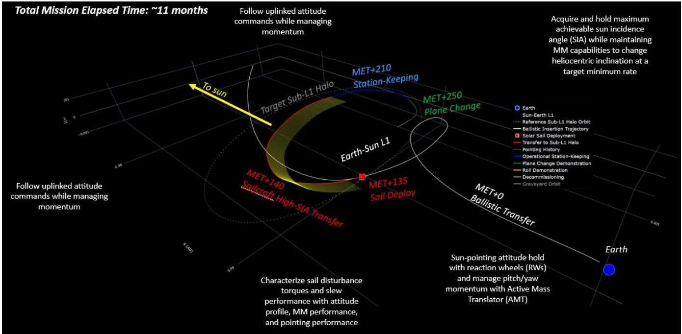
Figure 1. Solar Cruiser Planned Conops
