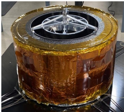
Figure 6. Sail Spool with Sail Restraint
