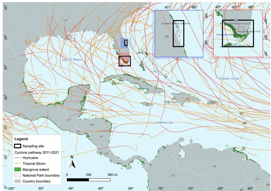
Figure 2. The Gulf of Mexico study region, showing mangrove extent (green) and the paths of tropical storms and hurricanes from 2011–2021 that drive the losses of mangroves through erosion and wind damage. Insets show the areas where the airborne component of BlueFlux will carry out eddy covariance measurements.
