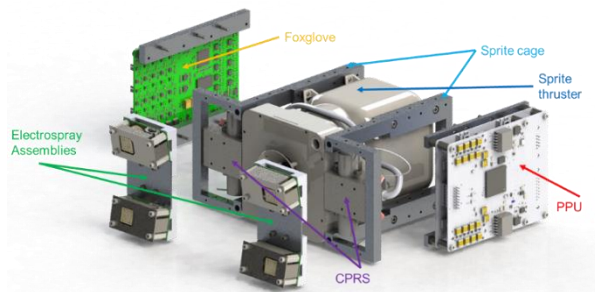
Figure 1. GPDM Propulsion System.
