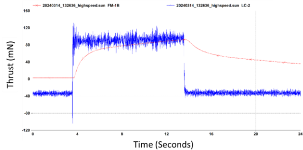
Figure 5. 10 second Single Pulse of the ASCENT 100 mN Chemical Thruster
