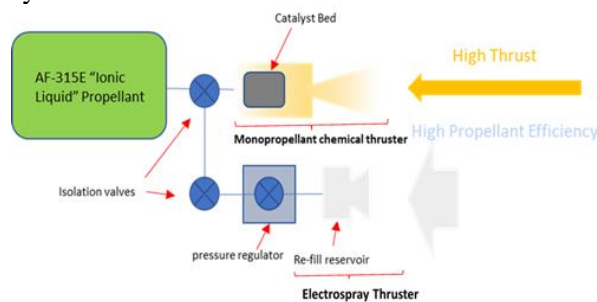
Figure 1 shows a schematic of an idealized ASCENT blowdown dual-mode propulsion system which includes a common propellant tank, a chemical monopropellant thruster, electro-spray thrusters and a compact pressure reduction mechanism which acts to reduce pressure from the propellant tank to the electro-spray thruster reservoirs.
