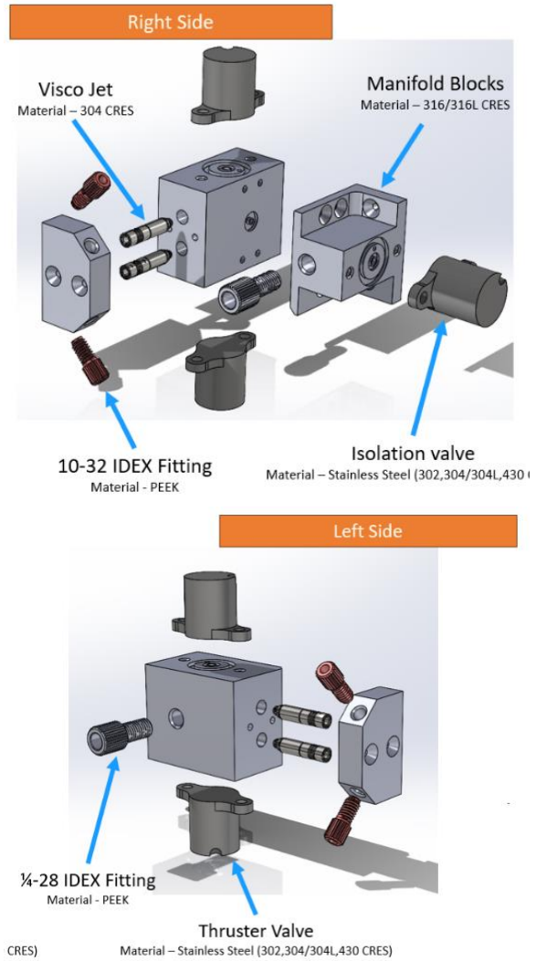
Figure 3. Detailed breakdown of updated CPRS design.
