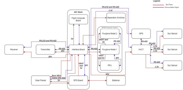
Figure 15: GPDM avionics integrated interface diagram.
