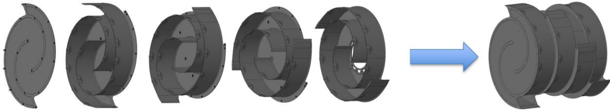
Fig. 23 IPEX TRL-5 bucket drum assembly CAD.
