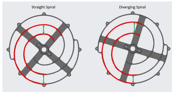
Fig. 24 Bucket drum straight spiral & diverging spiral geometries.
