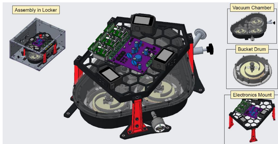
Fig. 25 IPEX bucket drum experimental payload overview.
