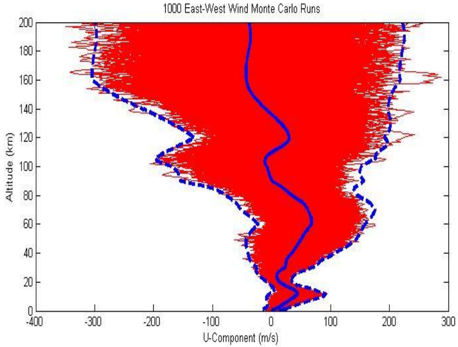
Figure 12. 1000 January East-West Wind Monte Carlo Dispersions with Mean and 3-sigma.
