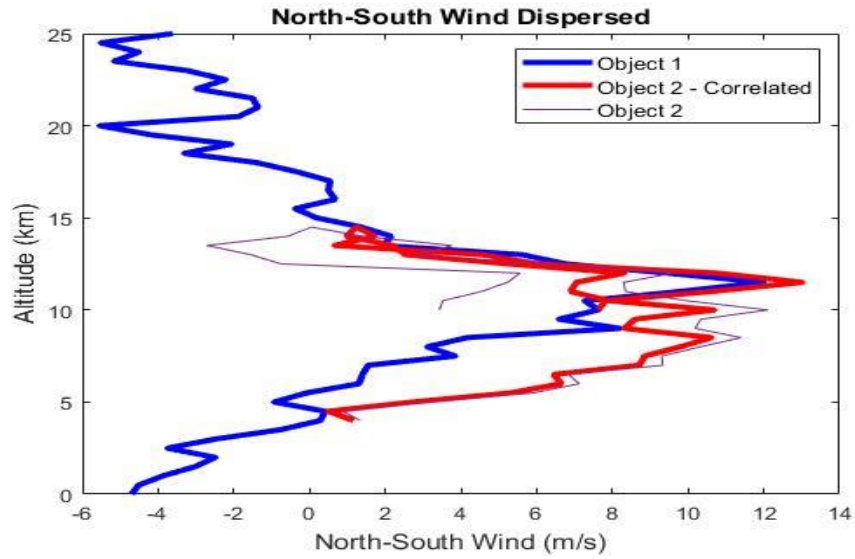
Figure 19. North-South Wind Dispersions Generated from Two Trajectory Objects Generated by Earth-GRAM.
