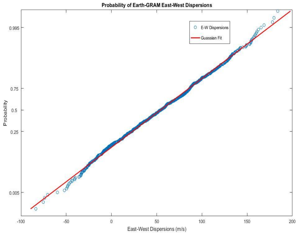
Figure 13. Cumulative Probability of East-West Wind Dispersion with a Gaussian distribution fit.
