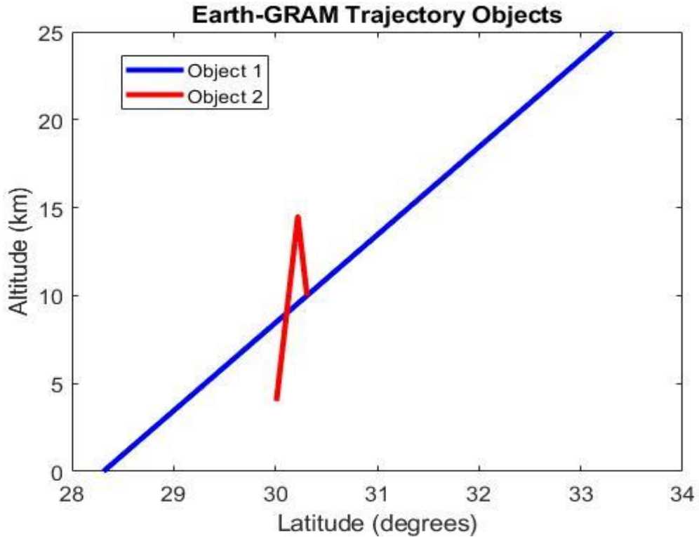
Figure 17. Positional Information Regarding Two Trajectory Objects Generated by Earth-GRAM.
