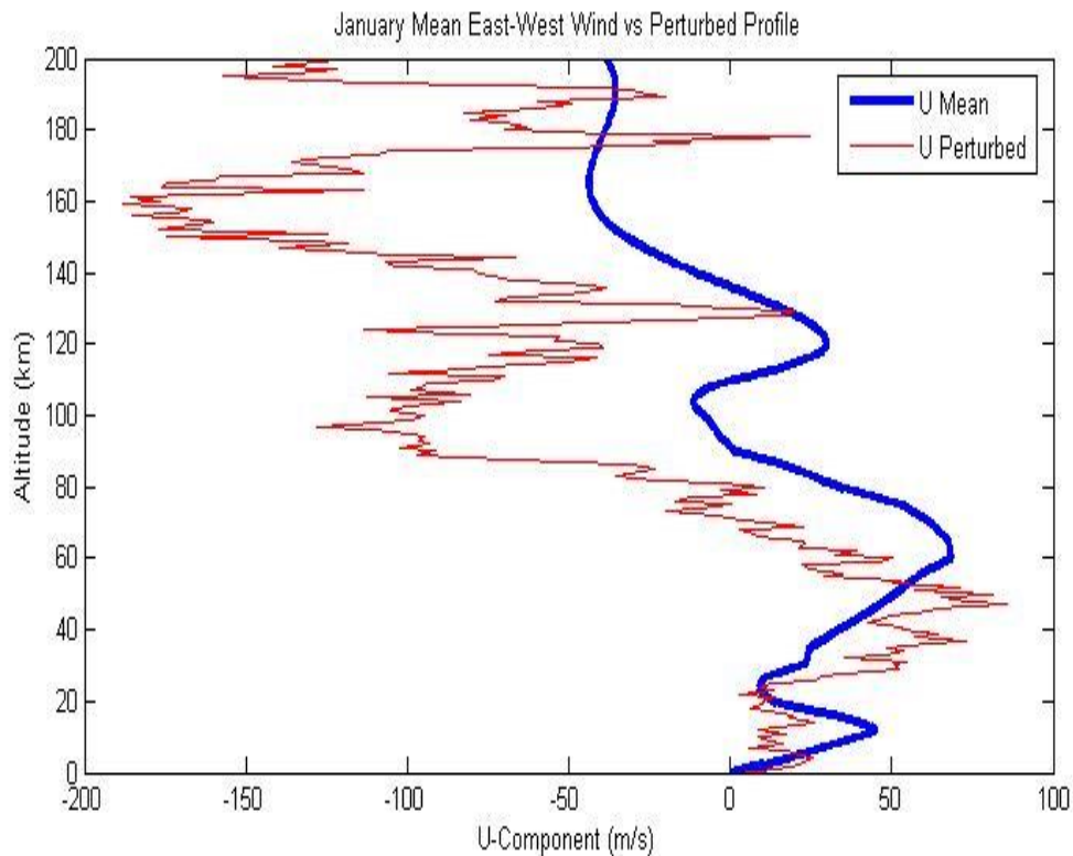
Figure 11. January Mean and Dispersed Profile of East-West Wind.
