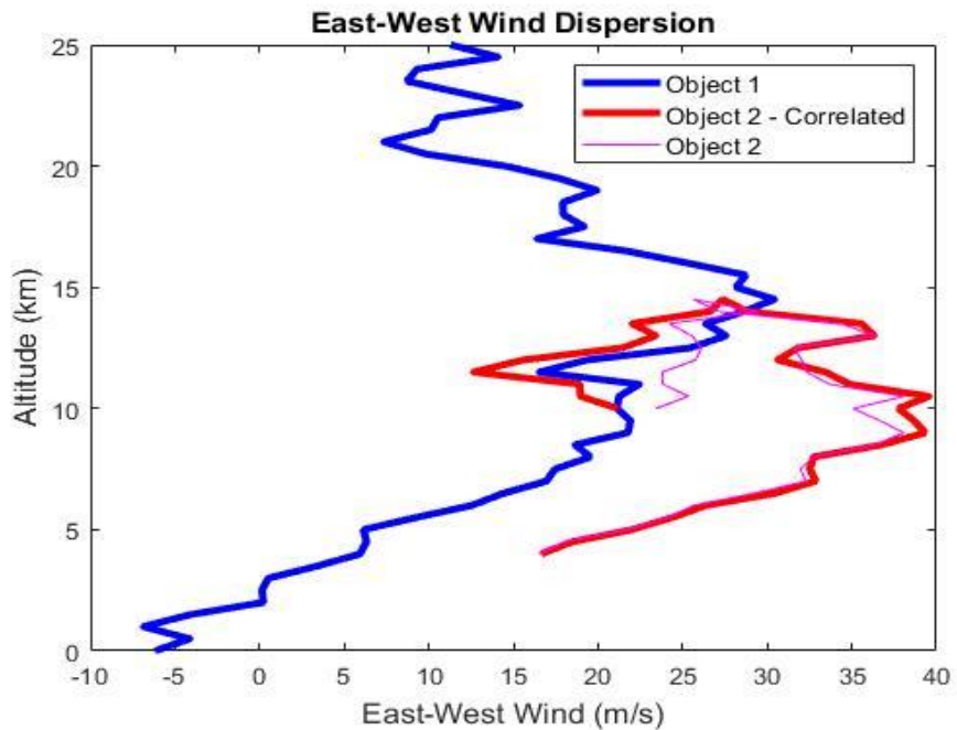
Figure 18. East-West Wind Dispersions Generated from Two Trajectory Objects Generated by Earth-GRAM.
