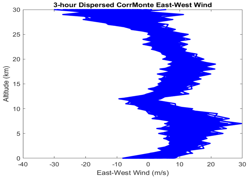
Figure 15. 1000 3-hour East-West Wind Dispersions about the Mean Generated by CorrMonte.
