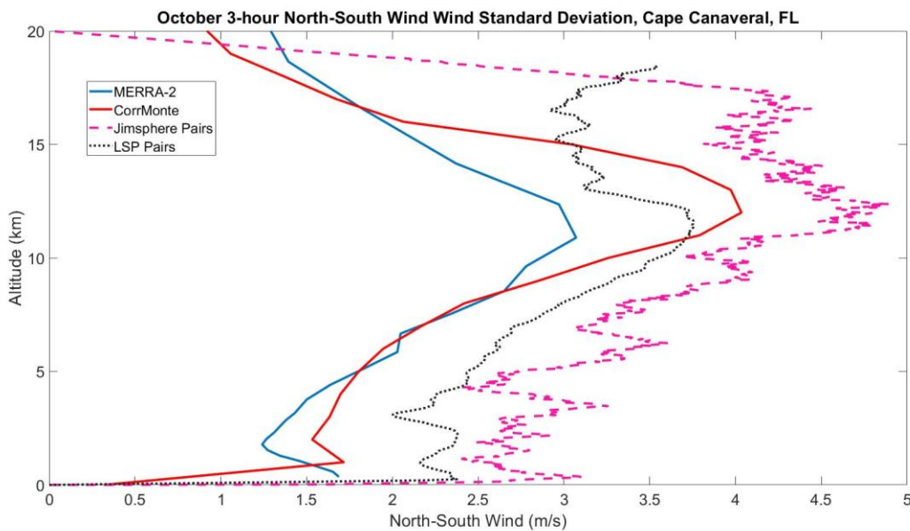
Figure 10. October 3-hour Comparison of North-South Wind Standard Deviation.
