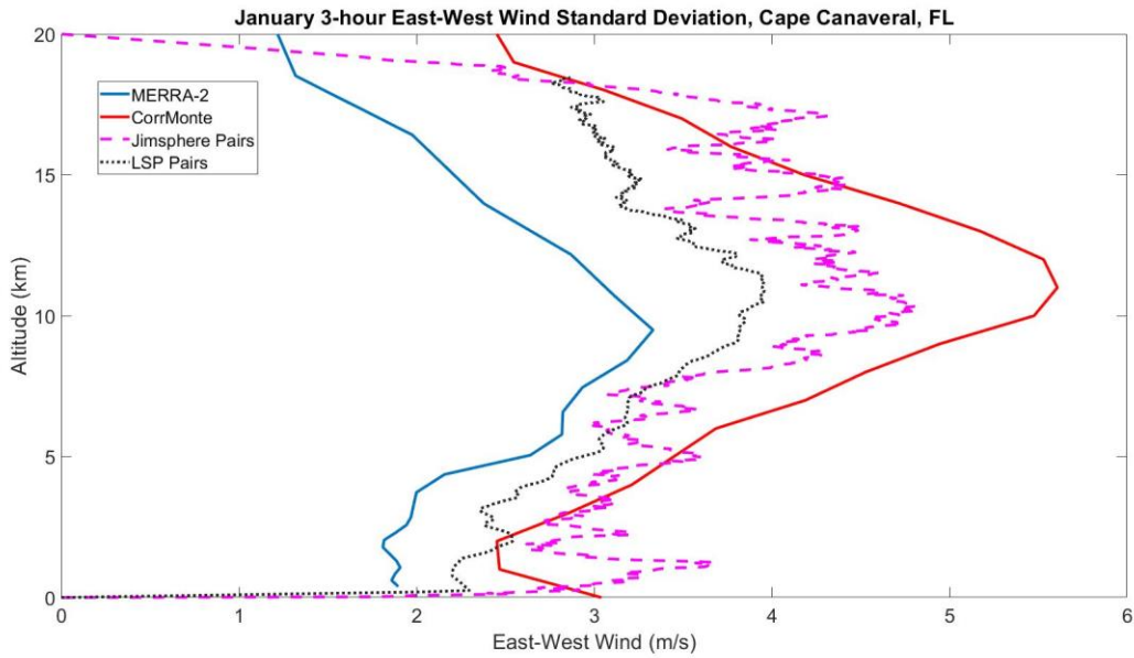
Figure 7. January 3-hour Comparison of East-West Wind Standard Deviation.
