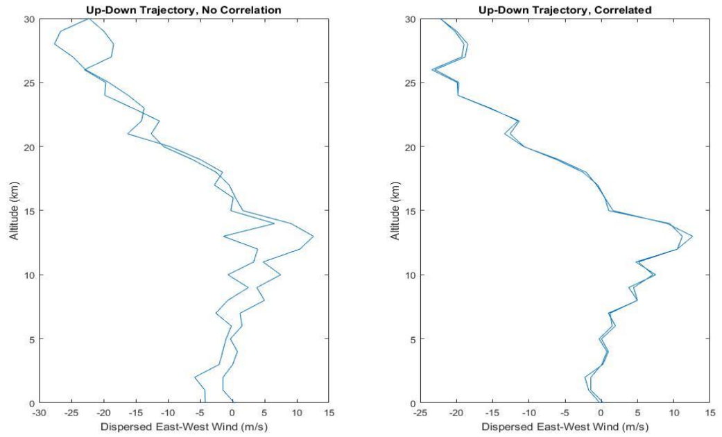
Figure 16. East-West Wind Dispersions Generated by Earth-GRAM (left) and the Ballistic Trajectory Feature (right).
