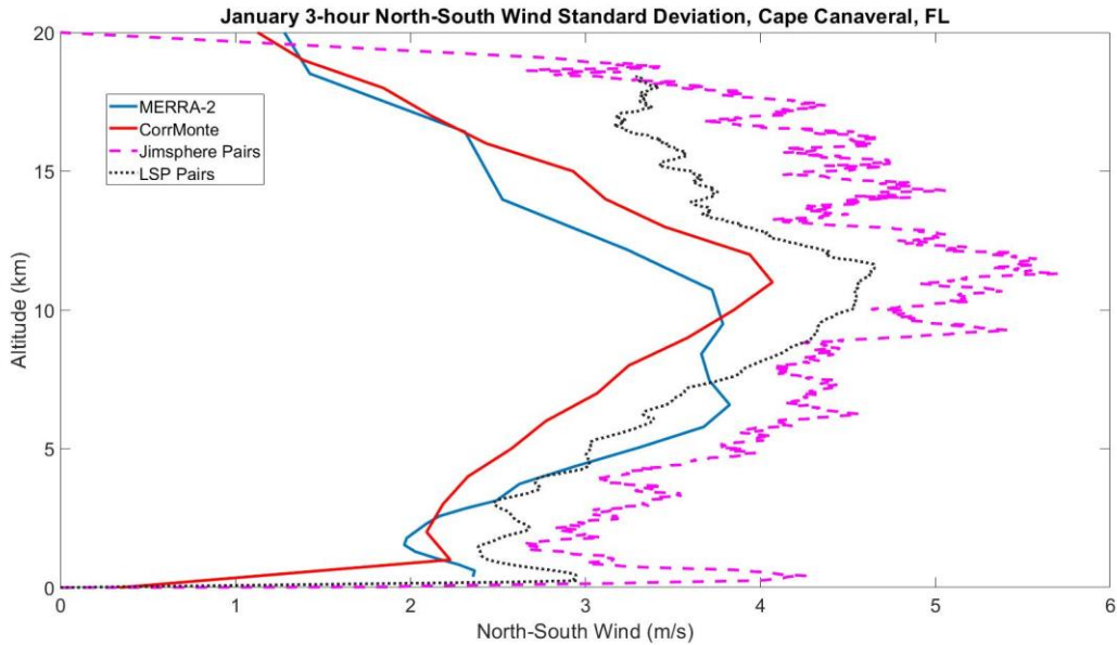
Figure 8. January 3-hour Comparison of North-South Wind Standard Deviation.
