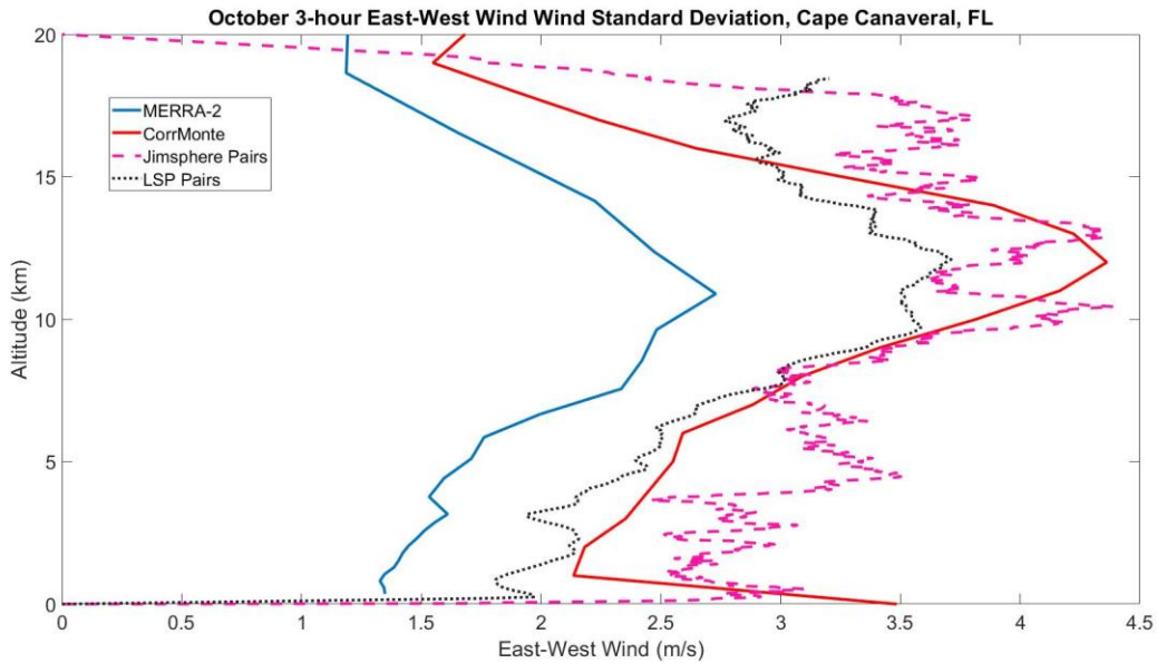
Figure 9. October 3-hour Comparison of Earth-West Wind Standard Deviation.
