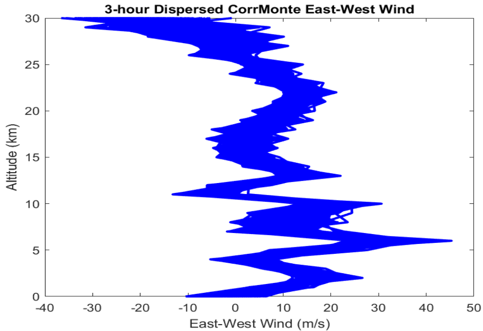
Figure 14. 1000 3-hour East-West Wind Dispersions about a Dispersed Profile Generated by CorrMonte.
