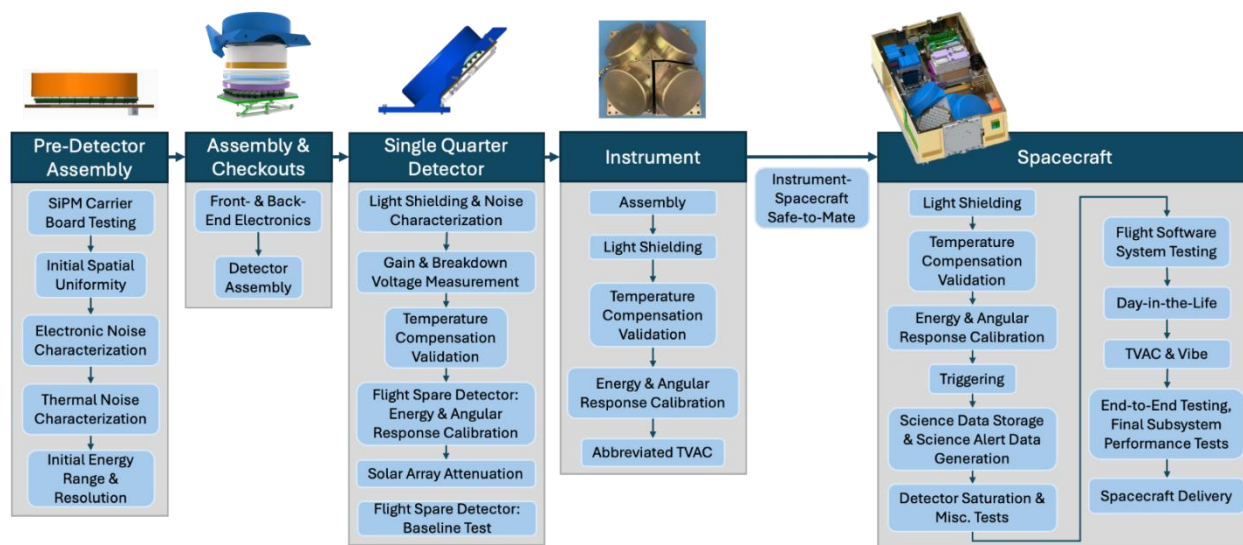
Figure 8: Instrument testing at each level of assembly and integration.
