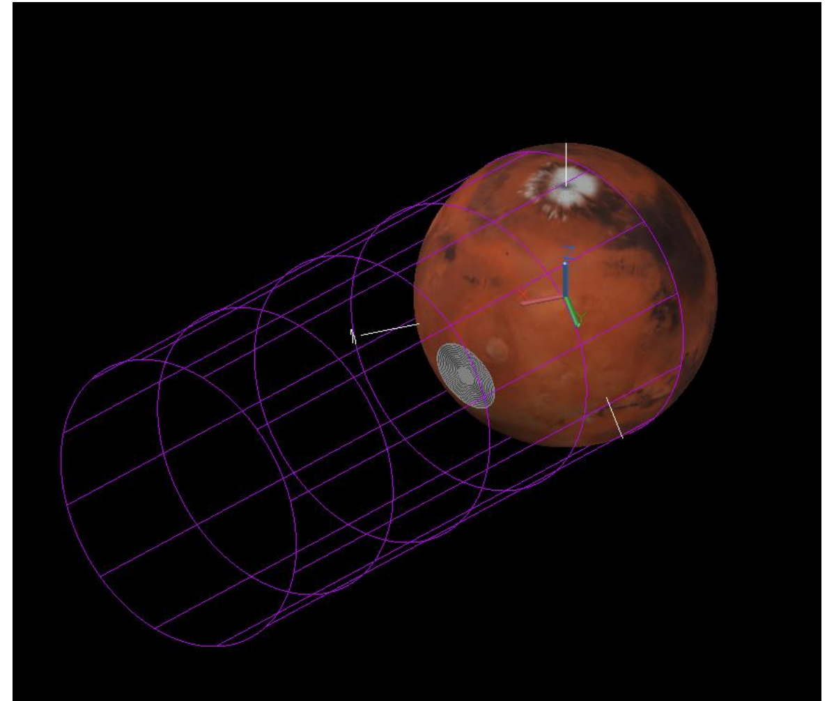
Orbit view showing the ground disk at 0° latitude at local midnight
