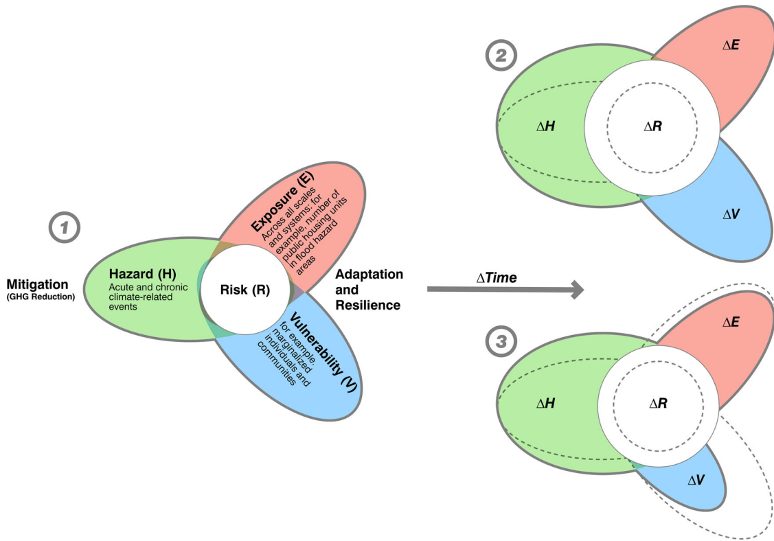
FIGURE 1 The impact of the dynamic components of climate risk ( R ) on its temporal evolution. Graphic 1 shows the baseline condition. Graphic 2 shows the impact of sluggish climate mitigation on the magnitude of the hazard ( H ) and the subsequent increase in climate risk. Graphic 3 shows that even with the implementation of climate adaptation and resilience strategies that reduce vulnerability ( V ) and exposure ( E ), climate risk may increase if the magnitude of the hazard continues to increase (adapted from Ref. 1).
