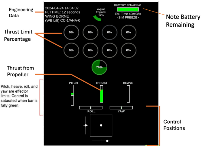
Fig. 10. System Health Display
