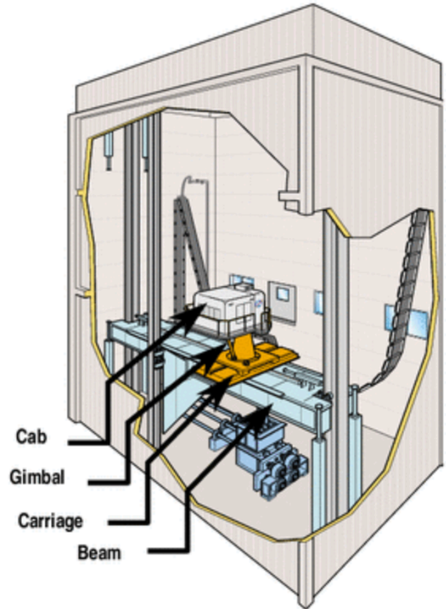
Fig. 20. NASA-Ames Vertical Motion Flight Simulator (World's largest Motion Base)
