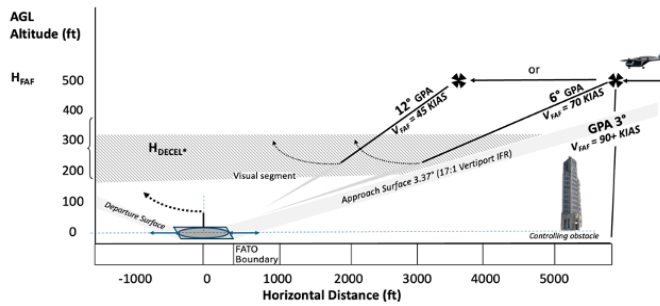
Fig. 16. Profile view of 6- and 12- degree approaches
