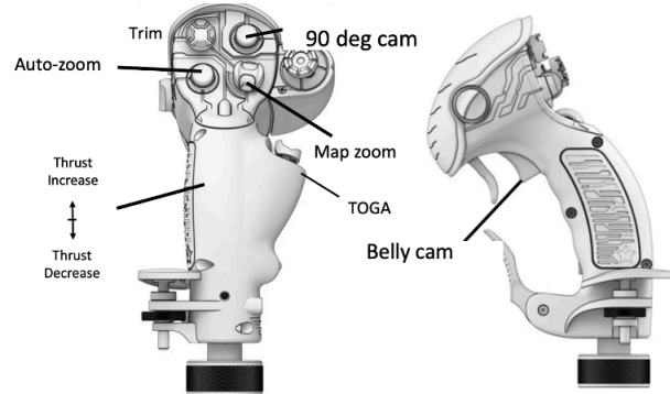
Fig. 11. Inceptors, grips, buttons and switches (Front and Side Views)
