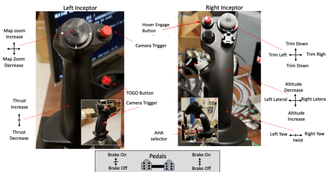
Fig. 19. VMS inceptor controls, grips, and mapping
