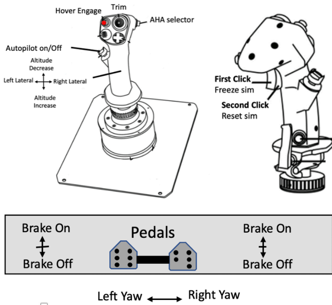
Fig. 12. Right Inceptor (front and back view) and Pedals
