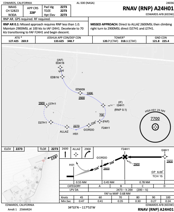
Fig. 15. Approach plate for the RNAV (RNP) 6 degree approach
