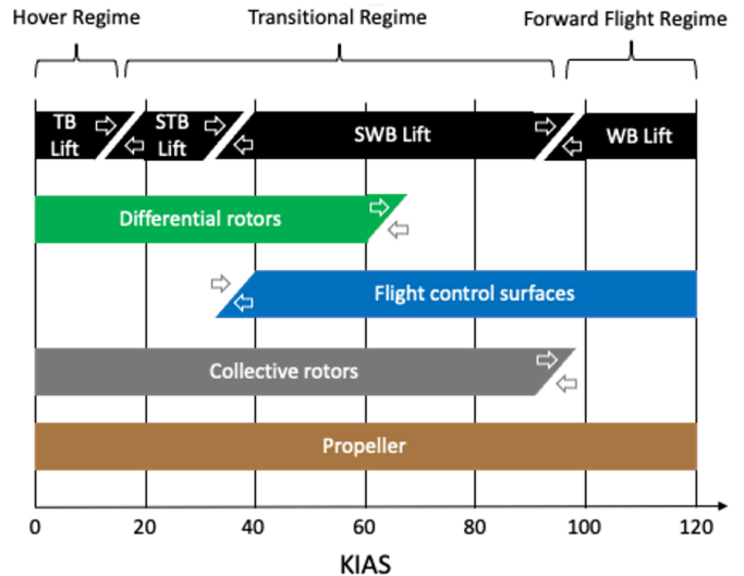
Fig 4. LPC Control Allocation Schedule (Lift Source, Control Surfaces, and Propeller Thrust)
