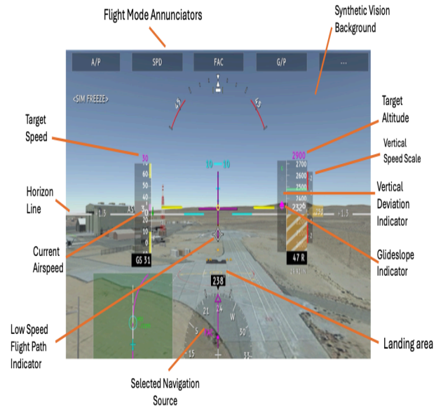
Fig. 7. Primary Flight Display with Synthetic Background
