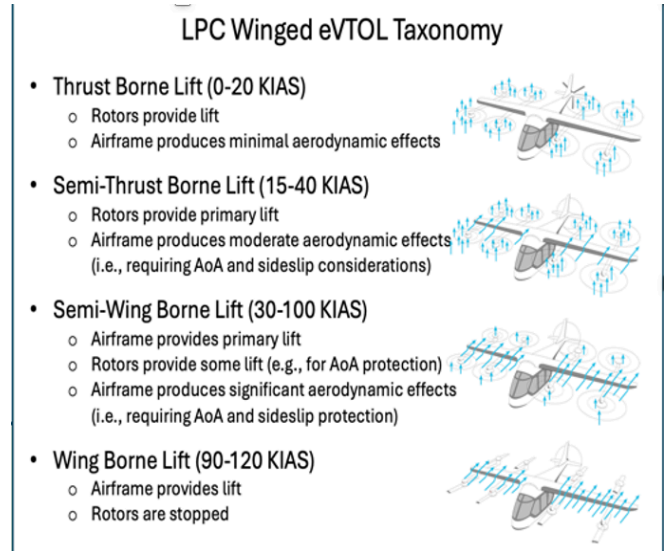
Fig 3. LPC Design Parameters and Lift Sources
