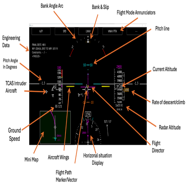
Fig. 8. Primary Flight Presenting Addition Information Elements (The black background is for illustration only)
