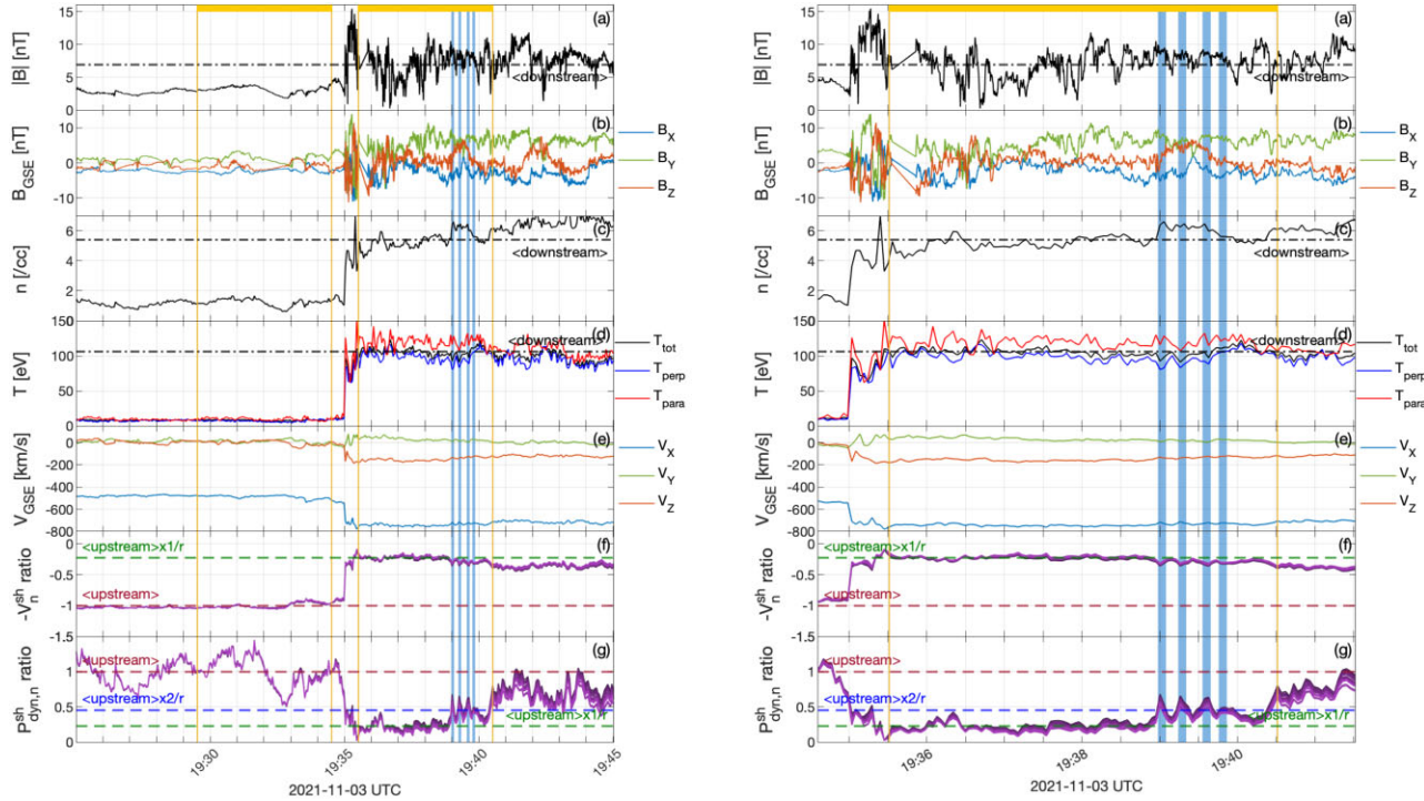
Figure 1. Event 1. From top to bottom: (a) magnetic field magnitude, (b) magnetic field components in GSE-coordinates, (c) ion density, (d) ion temperature, (e) ion velocity in GSE-coordinates, (f) -V_n^{\text{sh}} ratio, and (g) P_{\text{dyn},n}^{\text{sh}} ratio (20 purple curves corresponding to different shock parameter estimates). Yellow bars and vertical lines mark the 5 min upstream and downstream windows, where temporal averages are calculated, indicated with dashed and dash-dotted horizontal lines, respectively. The jet candidates where the dynamic pressure ratio threshold is exceeded for at least 11 of the 20 estimates, shock estimates, are highlighted in blue. The right-hand side shows a zoom-in of the downstream region.
