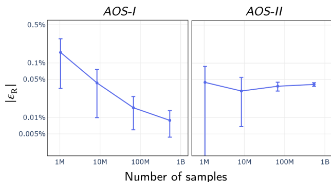
Fig. 6. (Absolute value of) Relative percent error in reflectance, |\varepsilon_{\text{R}}| , for AOS-I and AOS-II models at top of atmosphere, for \theta_\ell = 30^\circ , \theta_v = 30^\circ , \phi_v = 60^\circ . The mean of each set of 20 random trials is connected by dark purple line and the standard deviation of the trials is shown as error bars; both axes are a log scale. The AOS-I model shows a pattern of converging toward the reference result, while AOS-II shows a slight bias that approaches |\varepsilon_{\text{R}}| \sim 0.04\% .
