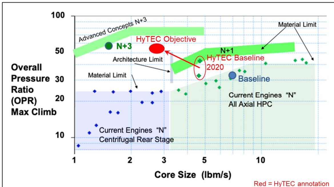
Figure 1: OPR versus core size for generation N, N+1, N+3 AIAA 2015-00071 [2]
