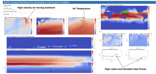
Figure 9: Increasing heat fluxes (two plots and images at the bottom right) and air temperature (image at top middle) create a high-velocity wind (image at top left) in the atmosphere moving eastward for the Kuroshio region.
