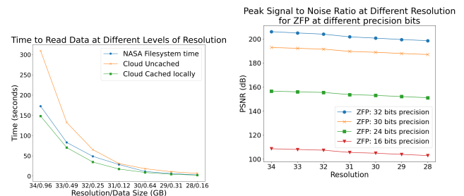
(a) Data retrieval time from different data locations at different levels of resolutions. (b) Peak signal-to-noise ratio for different bits of precision with ZFP compression algorithm.
