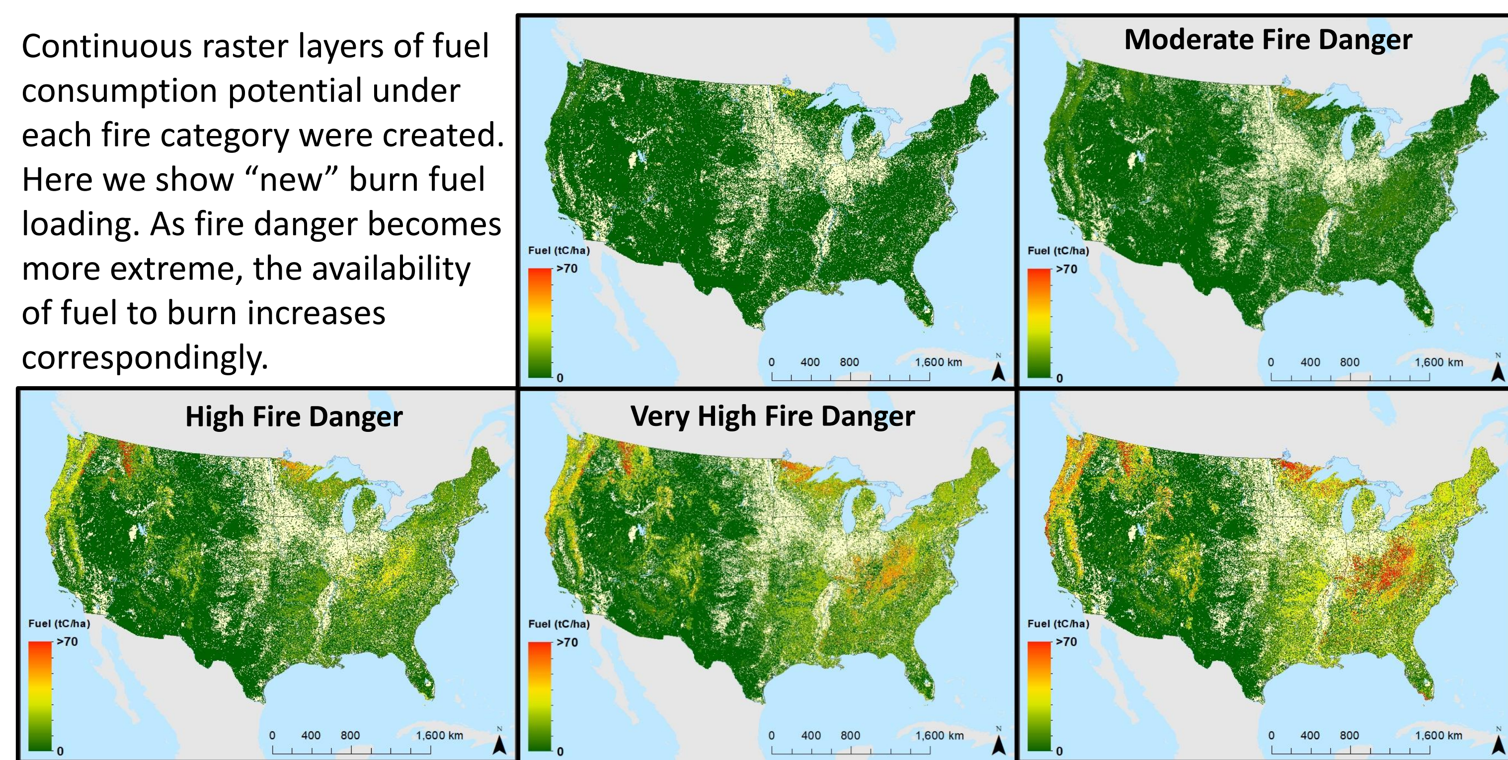
Figure 5: Resulting Fuel loading data layer for each fire danger category under 'new' burning conditions.
