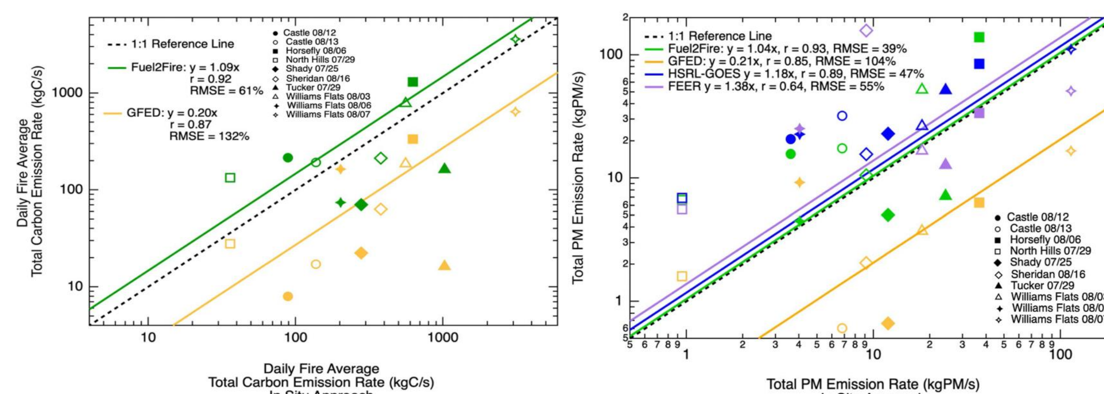
Figure 6: Total carbon emissions comparisons with in-situ aircraft data for FIREX-AQ
