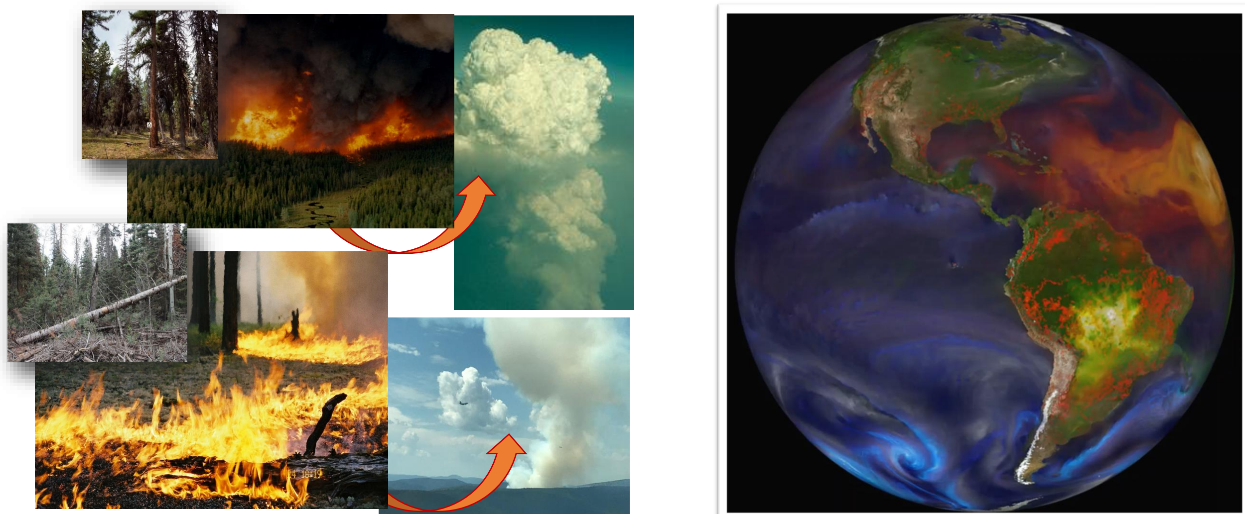
Figure 1: Fuel and fire weather are linked to fire carbon emissions and smoke plume injection height. Fire emissions are transported in the atmosphere, which is linked to global processes. Source: NASA Scientific Visualization Studio
