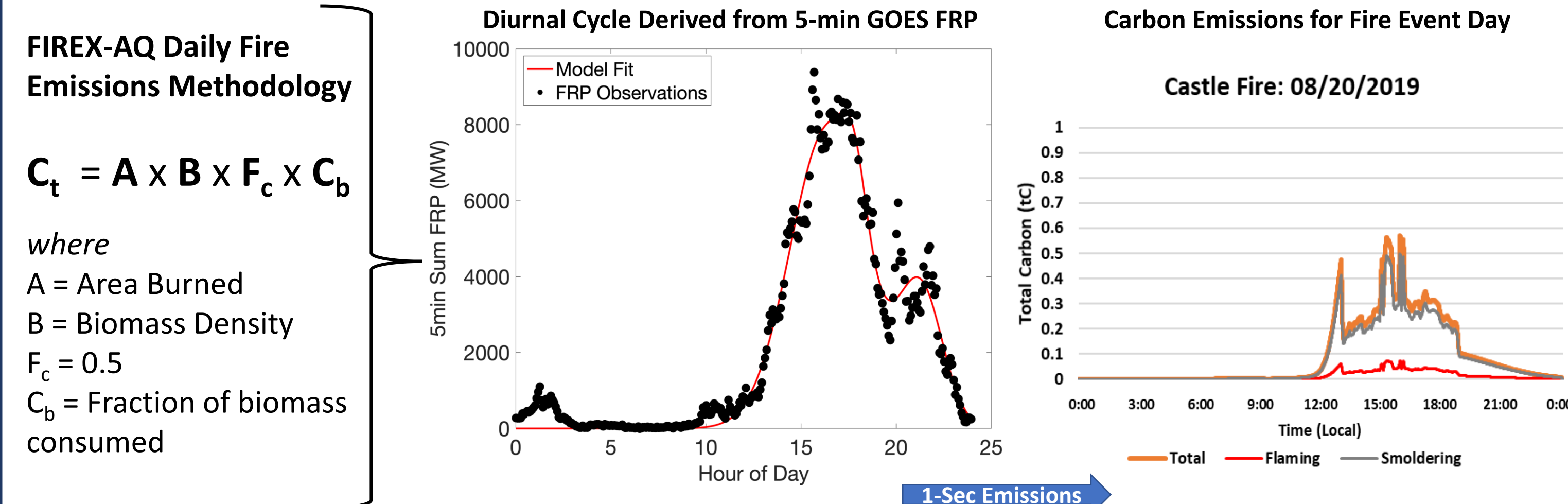
Figure 2: Emissions calculation showing the formula used (left), an example of a GOES satellite diurnal cycle used for distributing daily emissions (center), and the resulting daily carbon emissions for one day of a fire sampled (right).
