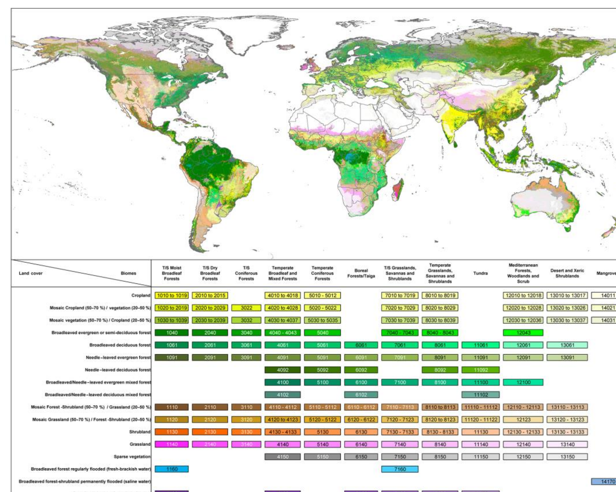
Figure 7: Pettinari & Chuvieco (2016) Global fuelbed map. The legend details the number of the fuelbeds, and the land cover biome that they represent.
