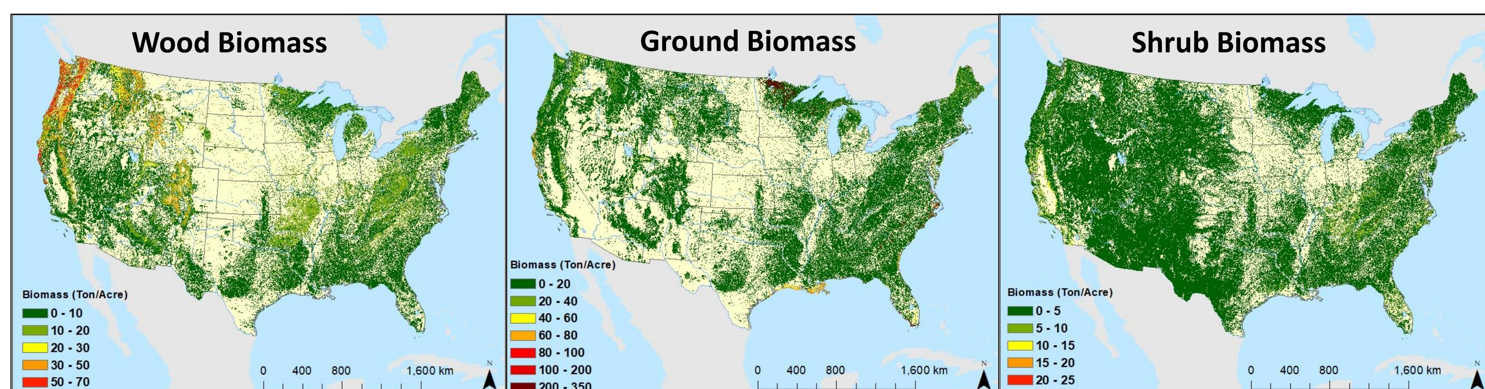
Figure 4: These maps show the carbon biomass loading (ton/acre) for some biomass variables
