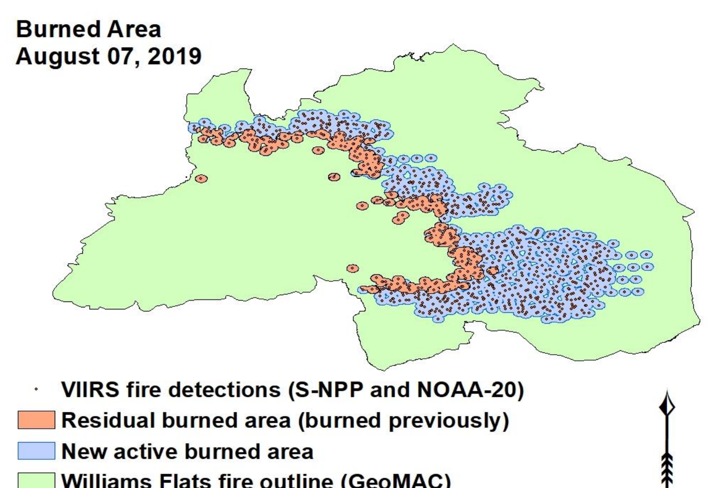
Figure 3: An example of burned area for one day of a fire
