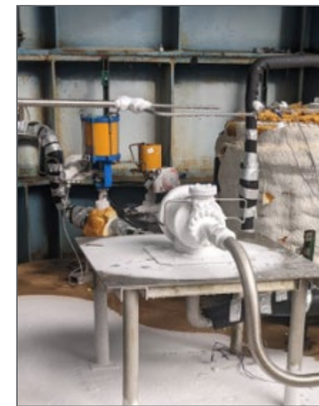
Low-leakage relief valve during LH2 testing
