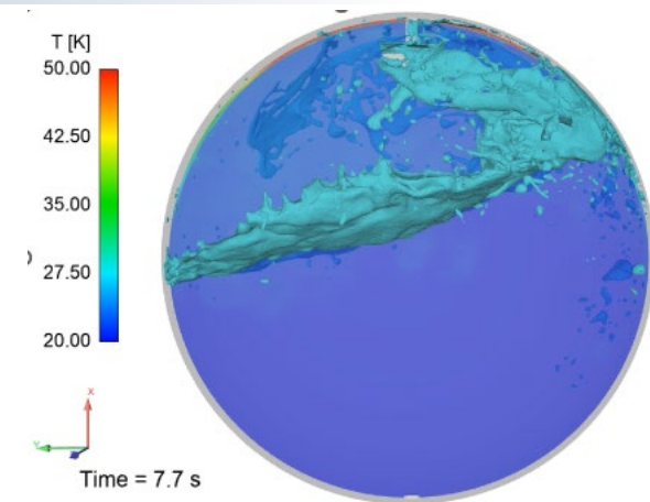
CFD Tank Propellant Slosh Analysis
