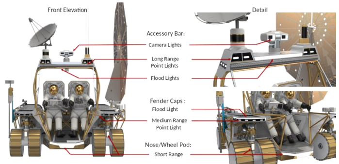
Figure 9. The LTV camera and lighting positions.
