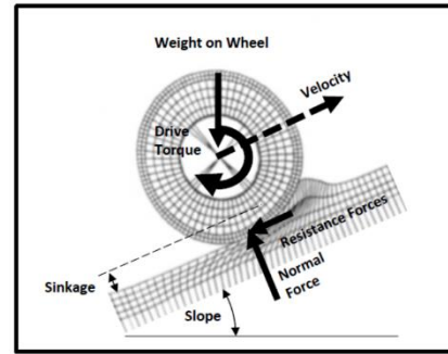
Modeling Soil Reaction as a Nonlinear Spring
