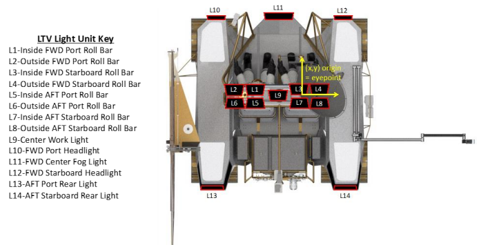
Figure 10. The LTV camera lighting unit locations.
