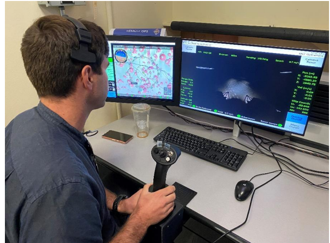
Figure 31. Remote operator in the teleoperation control center.
