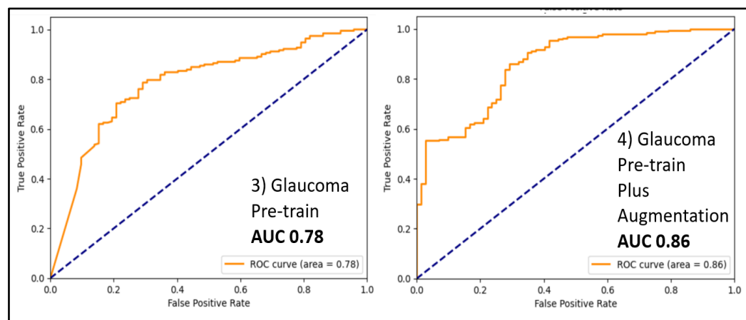
Overall model performance is 0.86, a perfect model would be 1.0
