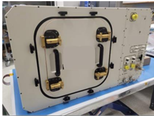
ODME Engineering Development Unit. Image Courtesy of Redwire.
