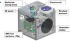
Portable on-Board 3D Printer (P3DP) – overall architecture
