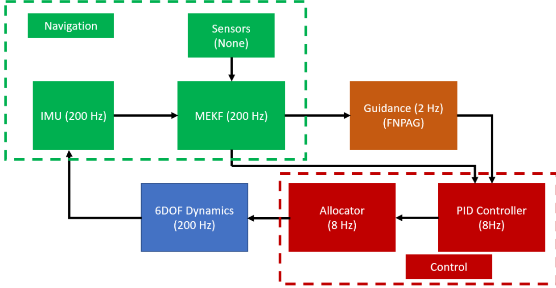
Fig. 2 Aerocapture simulation setup.
