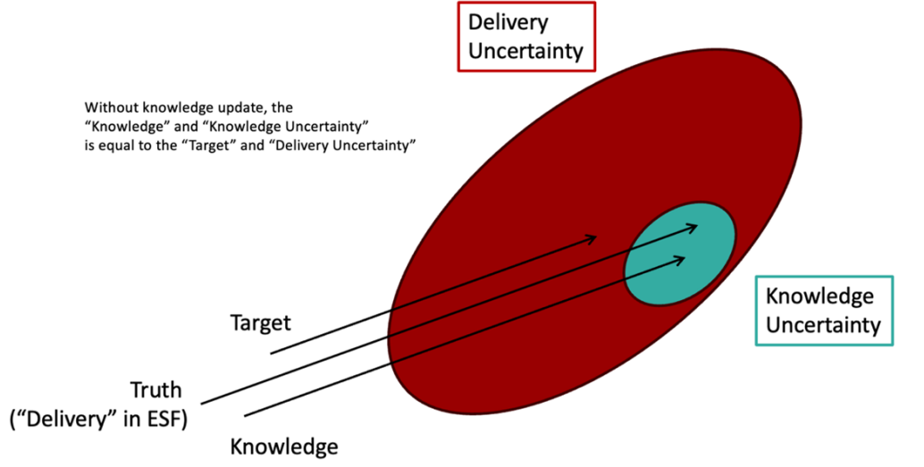
Fig. 1 Visualization of delivery and knowledge uncertainty at targeting entry interface point to start aerocapture
