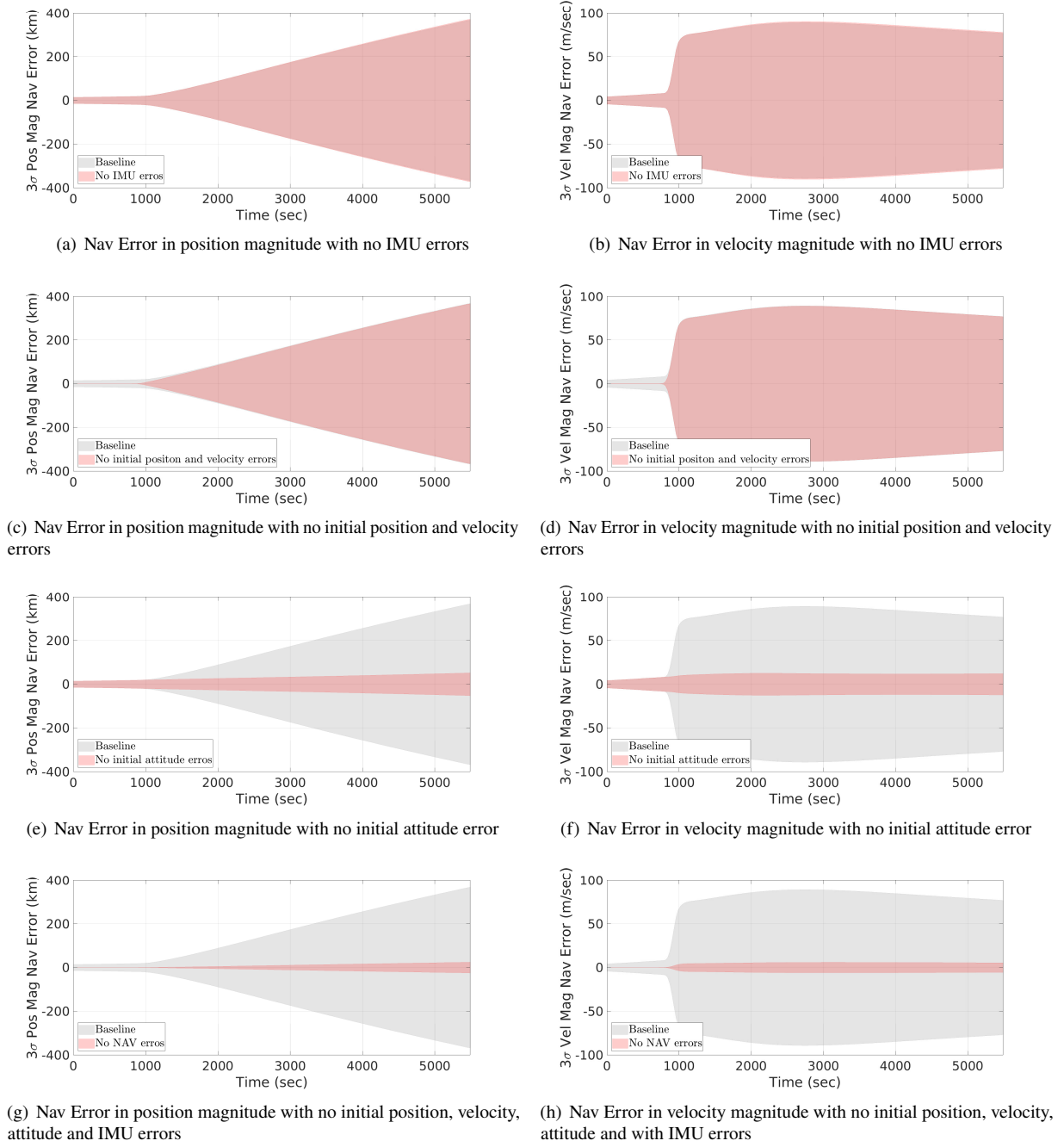
Fig. 6 Contribution of different sources to the onboard navigation errors during aerocapture
