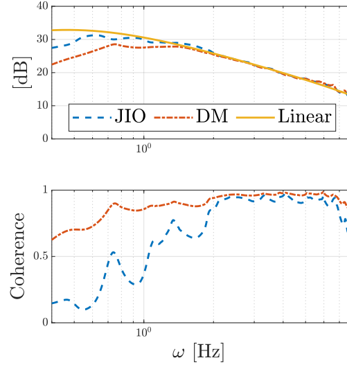
Fig. 9 Comparison of simulated frequency response with direct and JIO method in the presence of high-intensity disturbance.
