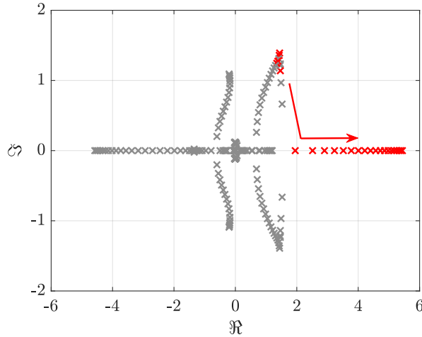
Fig. 2 Root loci of the bare-airframe dynamics with increasing horizontal airspeed.
