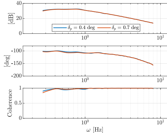
Fig. 6 Simulated roll rate p response to roll aligned input \delta_p with decreasing sweep amplitude A_0 .
