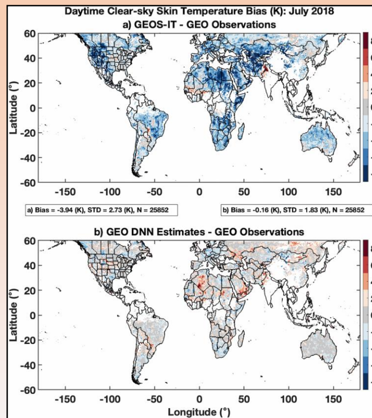
Previous DNN
