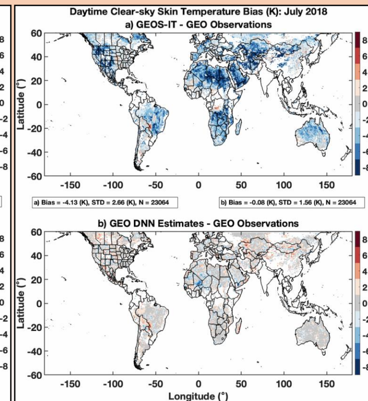
New DNN
