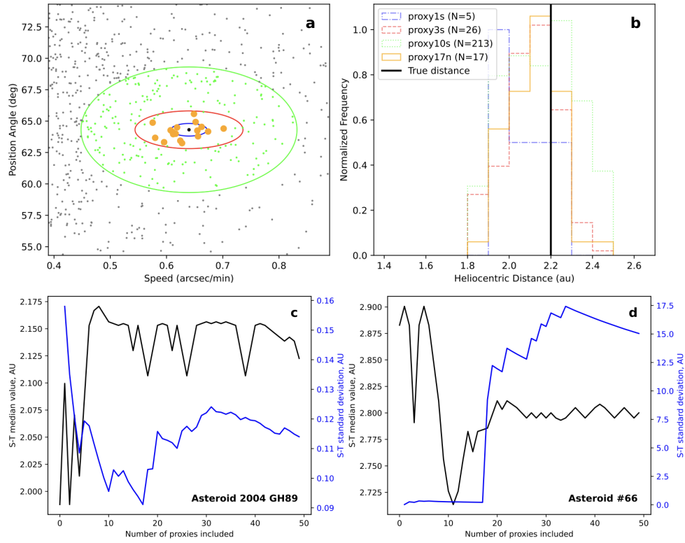
Extended Data Figure 2: Proof-of-concept application of population-based estimation of a distance to an asteroid a. Speed ( v ) and position angle (PA) of asteroid 2004 GH89 (black dot) compared to an ensemble of other known asteroids close to the field of view at the time of the observation (grey dots) together with proxy1s, proxy3s, and proxy10s ellipses (blue, red, green) used to select neighbors/proxies and the final 17 “proxy17n” proxies used (orange). b. Histogram of heliocentric distances (S-T) of from the different ensembles of proxies compared to the true value (black line) confirming that with an increasing number of proxies ( N ) the derived orbital configuration converges towards truth. c. Estimated heliocentric distance (black) and its uncertainty (blue) for asteroid 2004 GH89 as a function of N . For N \ll 10 , small number statistics can bias the derived distance and yield an artificially large associated uncertainty. Beyond N \sim 20 - 25 , more proxies present new/different orbital configurations resulting in sudden changes in the estimated value (otherwise converging) and thus a progressive inflation of the estimated uncertainty. d. Same as c. but for unknown asteroid #66 (likely NEO) with a limited number of close proxies leading to its 19 th and 20 th closest proxies to be clear outliers (TNOs) resulting in a sudden jump of its derived uncertainty.
