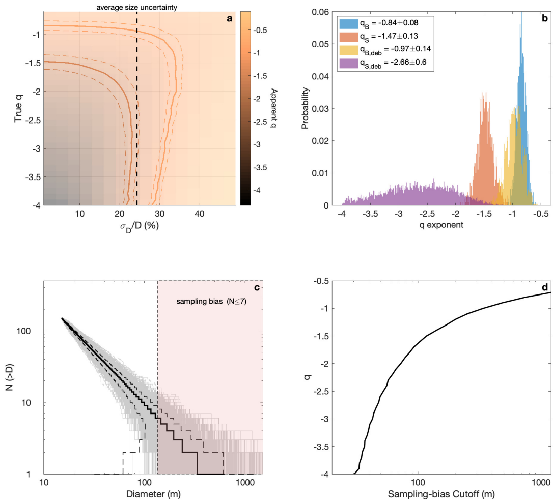
Extended Data Figure 6: Information content and sensitivity analysis of a size-frequency
