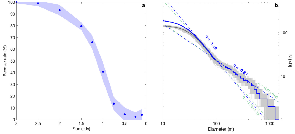
Extended Data Figure 1: Completeness test and recovery rate. a. Fraction of recovered synthetic asteroids as a function of their flux based on injection-recovery tests to assess the completeness of our search and correct the derived size-frequency distribution. The shaded area represent the 1-\sigma deviation from the reported rates seen across a range of injections. The derived cutoff is 0.5 \mu\text{Jy} with a observation bias starting at \sim 1.5 \mu\text{Jy} (i.e., at the 20- to 40-m size regime). b. Ensemble of cumulative size-frequency distributions (SFDs) built from 1,000 perturbed asteroid diameters in order to propagate the size uncertainties onto the SFD estimate (median in grey) via the Monte Carlo method 52 together with the SFD debiased for brightness-dependent recovery rate (blue).
