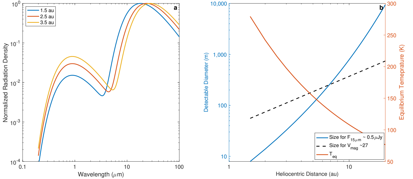
Figure 2: JWST’s far-infrared window into the main-belt asteroid population. a. Radiation Density (Jy) normalized to the peak emission for 0.1-albedo asteroids with an heliocentric distance of 1.5 (blue), 2.5 (red), and 3.5 au (yellow) showcasing the favorable infrared-to-visible flux ratio. b. Minimum size of an asteroid detectable for a 0.5 \mu\text{Jy} detection threshold at 15 \mu\text{m} compared to state-of-the-art capabilities in the visible—dashed line represents the radius detection threshold at V_{\text{mag}} \sim 27 (ref. 6 ). With a 0.5 \mu\text{Jy} detection threshold (Extended Data Figure 1), JWST can outperform searches in the visible up to 10 au, and by up to two orders of magnitude in size in the main belt.
