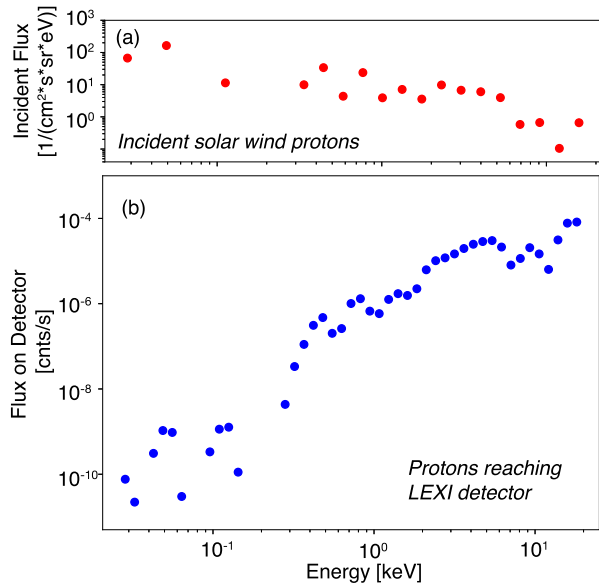
Fig. 7 Charged particles at LEXI. (a) Proton flux measured by THEMIS at the moon in the solar wind. The flux is from a look direction corresponding to LEXI's science pointing, 60^\circ - 120^\circ from the Earth-sun line. (b) Modeled solar wind protons reaching the LEXI detector after passing through the sweeping magnets and blocking filter. Total incident proton counts is modeled to be less than 0.5 \text{ s}^{-1} for nominal solar wind conditions
