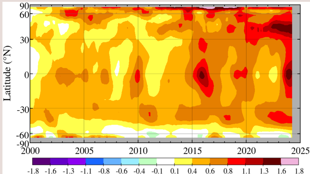
Figure 10. Zonal-mean Sea Surface Temperature anomaly ( ^{\circ}\text{C} ). **
