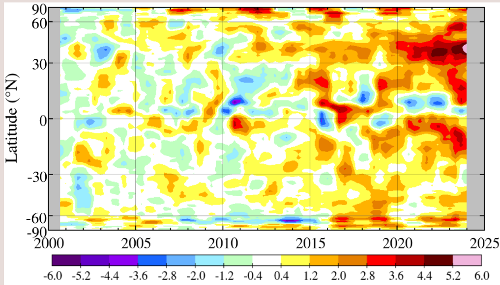
Figure 9. Zonal-mean Absorbed Solar Radiation anomaly ( \text{W/m}^2 ). **
