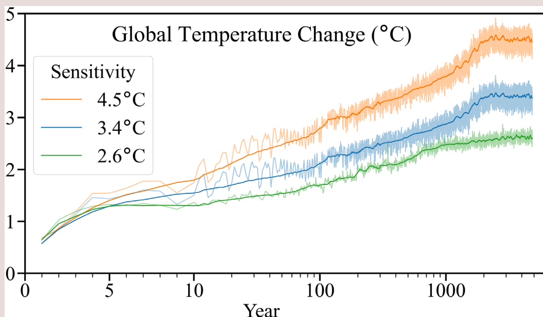
Figure 14. Global Temperature Response to 2 \times \text{CO}_2 . **
