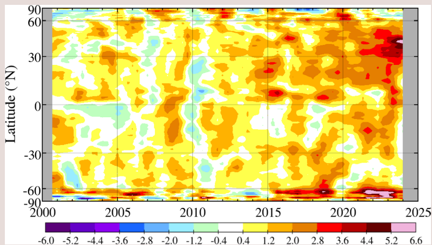
Figure 12. Zonal-mean Earth energy balance over ocean ( \text{W/m}^2 ).**
