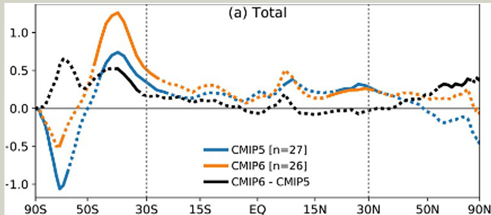
Figure S4a. Shortwave low cloud feedbacks ( \text{W/m}^2 per ^{\circ}\text{C} ).**
