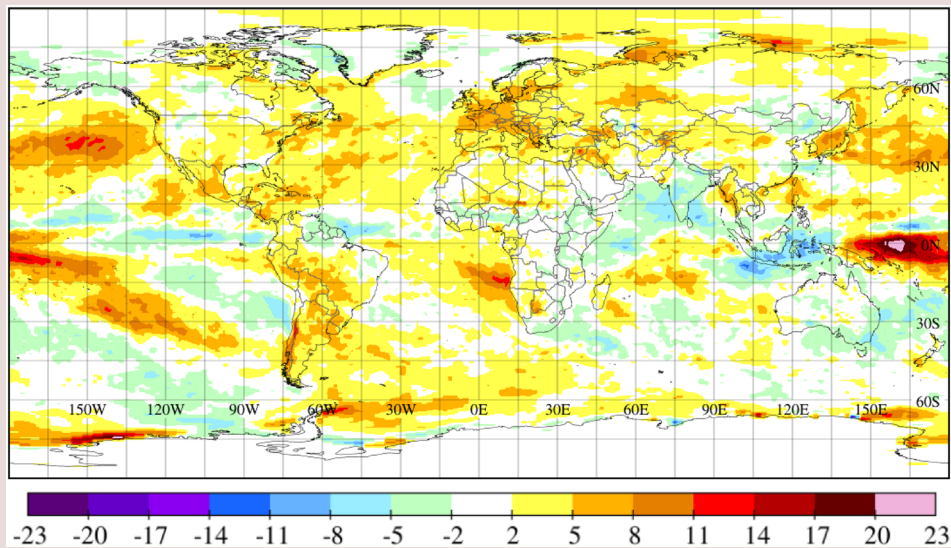
Figure 8. Absorbed Solar Radiation anomaly ( \text{W/m}^2 ) in 2020-23.**
