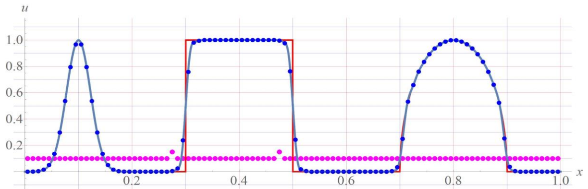
(c) DG3 solution with limiting and \sigma = 0.125 after 800 time steps (distance travelled: 1 period)
