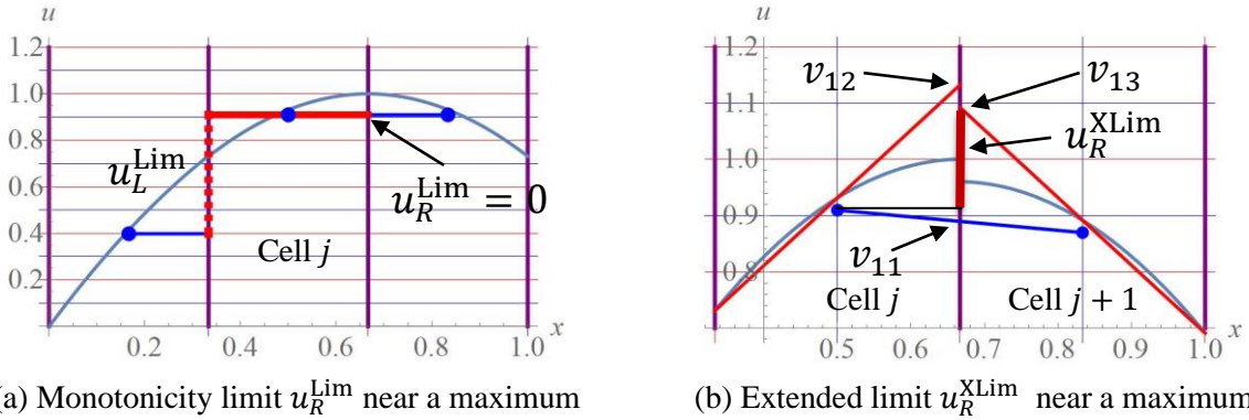
Fig. 5.2: (a) u_R^{\text{Lim}} reduces to 0, and limiting causes a loss of accuracy; (b) near a smooth maximum with a nonzero curvature, the extended limit u_R^{\text{XLim}} provides ample room so limiting has no effect.
