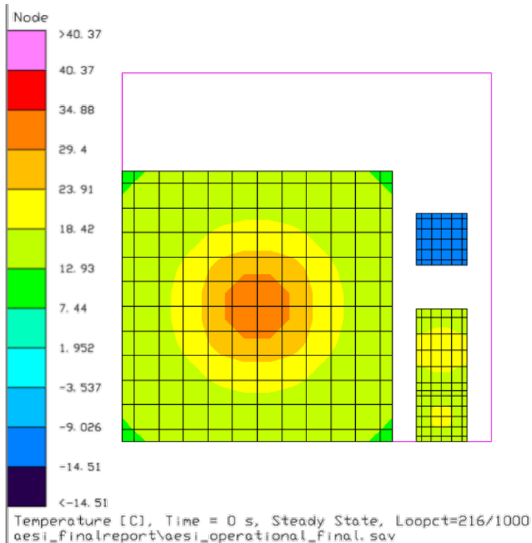
Figure 3.29 AeSI Operational Mode steady-state radiator temperature map. (top) Hub and (bottom) Cart. The temperature scale is in degrees Celsius. See Figures 3.3.3-1 and 3.3.3-2 for labels indicating the components served by each of the radiators.
