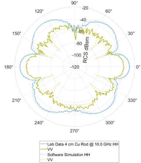
Figure 9. Comparison of Test 16, a copper rod, between the laboratory measurements and CEM simulation at 10 GHz. There is good agreement between the laboratory measurements and the CEM simulations where the laboratory measurements have high signal-to-noise.
