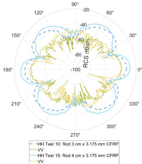
Figure 6. Comparison of two CFRP rods, Test 10 and Test 15, at 10 GHz. The two rods have the same radius, but the Test 15 rod is longer. At 0 degrees and 180 degrees, the RCS of the longer rod is higher in both the HH and VV polarizations.
