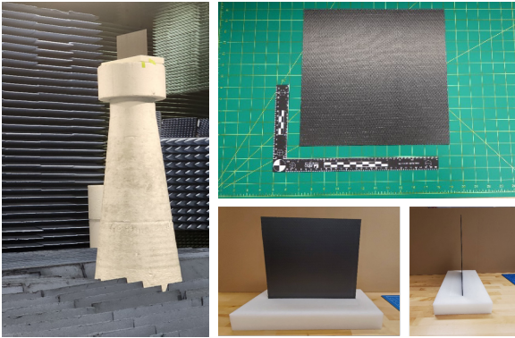
Figure 3. Top right: example of one of the calibration targets, a CFRP square plate. Bottom right: two views of the same target in a custom-made low-loss foam sample holder. Left: target and holder placed on rotating foam positioner pedestal in the OSU-ESL radar range.
