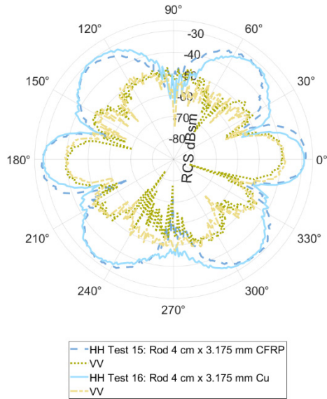
Figure 8. Comparison of Test 15, CFRP rod, and Test 16, copper rod, at 10 GHz. These two rods have the exact same dimensions. The two materials show a similar azimuthally dependent RCS, with some differences in the HH polarization.
