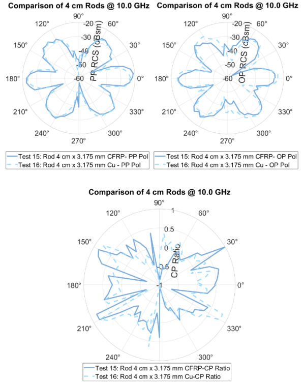
Figure 11. Comparison of circular polarization properties for Test 15, a CFRP rod, and Test 16, a copper rod, at 10 GHz. These two rods have the exact same dimensions. Top left shows the PP polarization, top right shows the OP polarization, and the bottom shows the CP ratio. The two materials show a similar azimuthally dependent RCS in both PP and OP.
