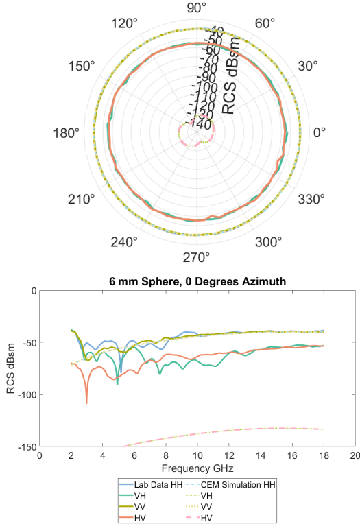
Figure 4. Azimuthal RCS of Test 3, a 6 mm sphere, at 15 GHz (top) and frequency dependant RCS of the same at 0 degrees azimuth (bottom). Lab data for each polarization are denoted by the solid lines, while CEM simulations are shown as dashed lines.
