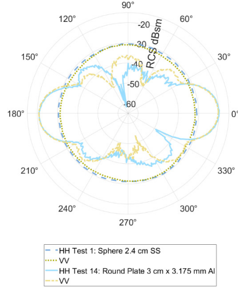
Figure 5. Comparison of Test 1, the 2.4 cm sphere, and Test 14, the 3 cm diameter round plate, at 10 GHz. Both objects have a similar L_c , 24 mm for the sphere versus 22.2 mm for the plate. This figure demonstrates the very different azimuthally dependent monostatic RCS between the spherical versus non-spherical object.
