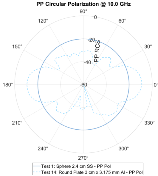
Figure 12. Comparison of the PP RCS (dBsm) for Test 1, a stainless steel sphere, and Test 14, a round aluminum plate, at 10 GHz. These objects have L_c = 24 mm and L_c = 22.2 mm, respectively.
