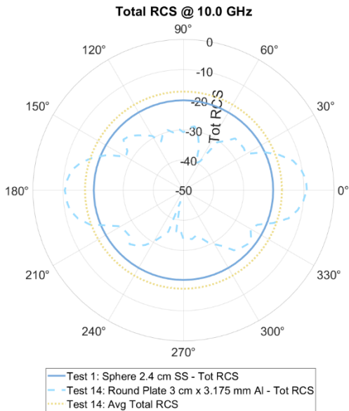
Figure 13. Comparison of the total RCS (dBsm) for Test 1, a stainless steel sphere, and Test 14, a round aluminum plate, at 10 GHz. These objects have L_c = 24 mm and L_c = 22.2 mm, respectively. Also shown is the azimuthally averaged total RCS for Test 14.
