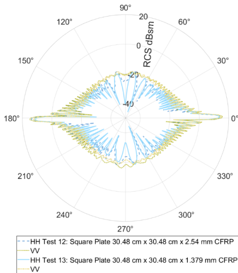
Figure 7. Comparison of two CFRP plates, Test 12, CFRP plate with a unidirectional weave and Test 13, CFRP plate with a quasi-unidirectional weave, both at 10 GHz. The two plates are square with 30.48 cm sides, and the square face of the plates were perpendicular to the incoming beam at 0 degrees azimuth.
