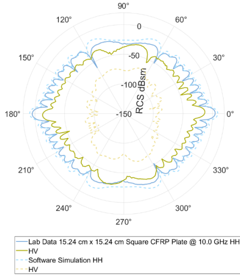
Figure 10. Comparison of Test 9, a CFRP plate, between the laboratory measurements and CEM simulation of a perfect conductor at 10 GHz. There is good agreement between the laboratory measurements and the CEM simulations for the HH polarization, although the lab data has a slightly smaller RCS at all azimuth angles than the simulated data. There is substantial disagreement for the HV polarization, as the perfectly conducting simulation does not capture the polarizing properties of the CFRP.
