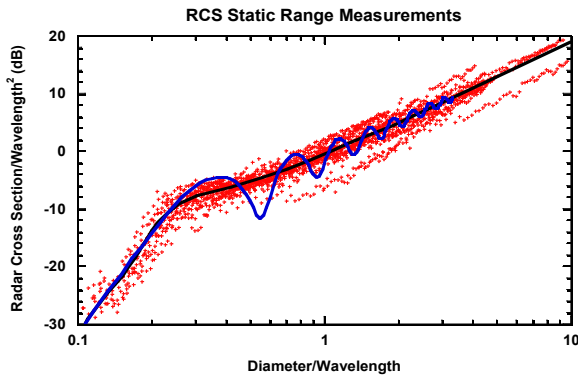
Figure 1. Results of RCS-to-size measurements on 39 representative debris objects (red +). The oscillating blue curve is the RCS for a spherical conductor while the smooth black curve represents the NASA SEM and is the polynomial fit to the data.
