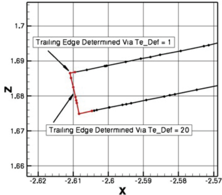
Figure B4: Sliced section corresponding to Fig. B3; zoomed in to the trailing edge region.
