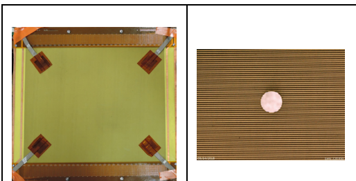
Figure 8. SDM test article (left) and a 1 mm diameter damage hole (HITF18172, 2018).
