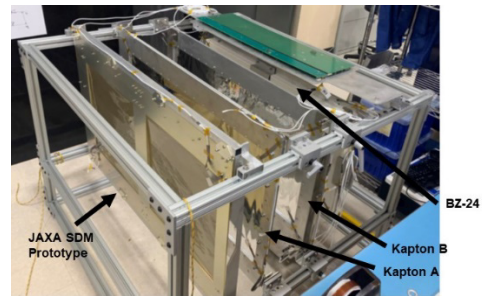
Figure 9. MACS prototype unit with 4 layers.
