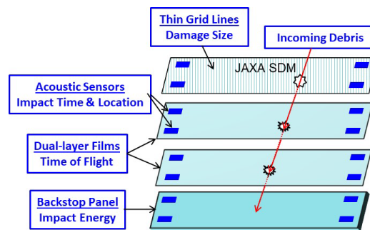
Figure 2. MACS Detection Principles.
