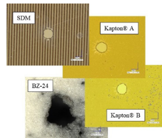
Figure 10. Impact features on the 4 layers of the MACS prototype unit (HITF23124, MACS148, 2023).
