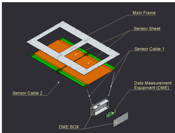
Figure 5. Illustration of the MACS SDM.
