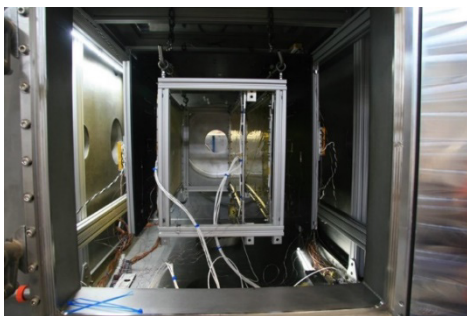
Figure 11. Test setup of the MACS Kapton ® layers and the BZ-24 foam panel inside a thermal vacuum chamber.
