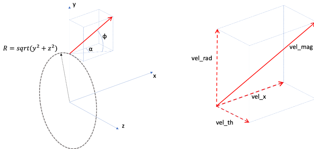
Figure 9.18: Radial cloud coordinate system.
