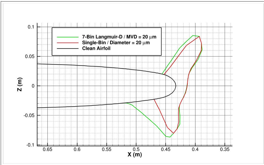
Figure 8.10: Single-Bin 20 \mu\text{m} diameter versus 7-Bin MVD = 20 \mu\text{m} Langmuir-D Ice Shape Comparison at Y = 0.75 \text{ m} .
