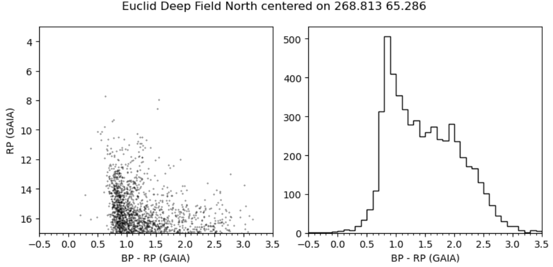
Figure 6: Color-magnitude diagram of sources in Gaia magnitudes with the RP and BP filters (left) and the color distribution of sources (right) for the EDFN wavelength calibration field.
