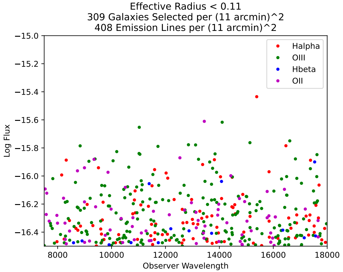
Figure 13: After limiting galaxies to \sim 1 pixel in radius, there are at least \sim 100 sources per detector with line fluxes brighter than a few times 10^{-17} \text{ ergs/cm}^2/\text{s} and that the emission lines are well distributed over the prism wavelength range. The figure shows (11 \text{ arcmin})^2 or about 2 detectors worth of area.
