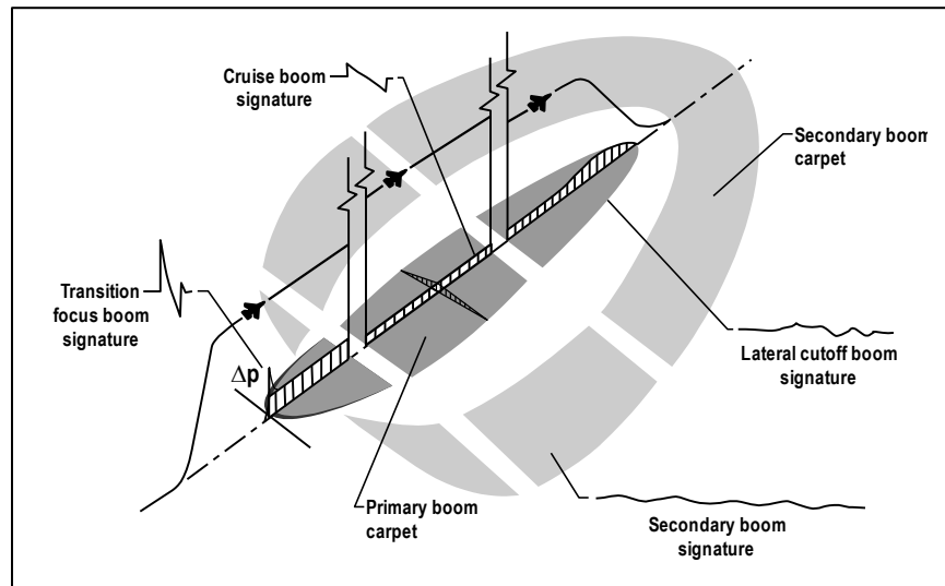
Figure B-71 Sonic boom carpet regions. 33
