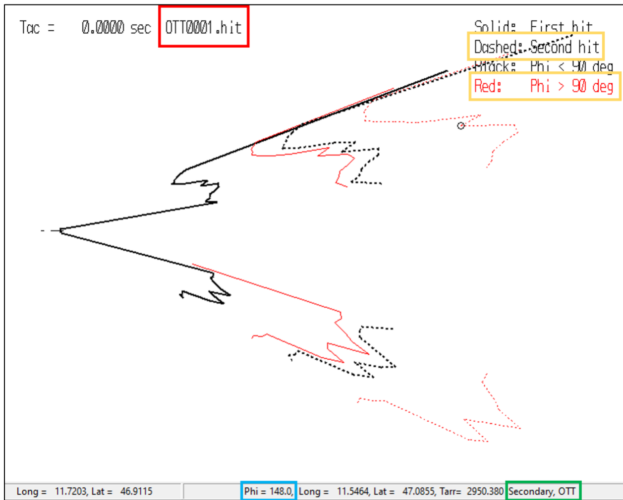
Figure B-75 OTT case POTTI visualization of the primary and secondary sonic boom footprint from the first trajectory point.
