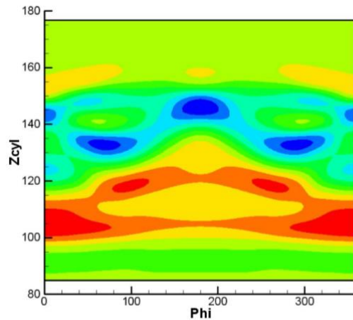
Figure 3-18 Example cylinder.plt file, unwrapped flat.
