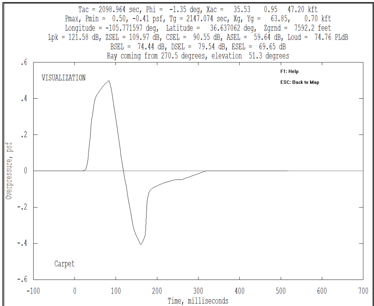
Figure B-8 Visualization case, signature view.
