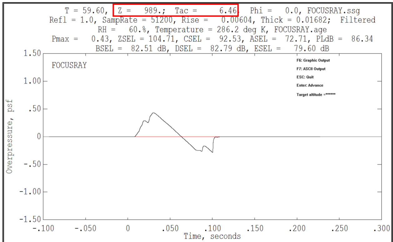
Figure B-68 PCBurg focus delta ray propagation termination at Burgers-LNTE interface altitude and Tac = TADVANCE.
