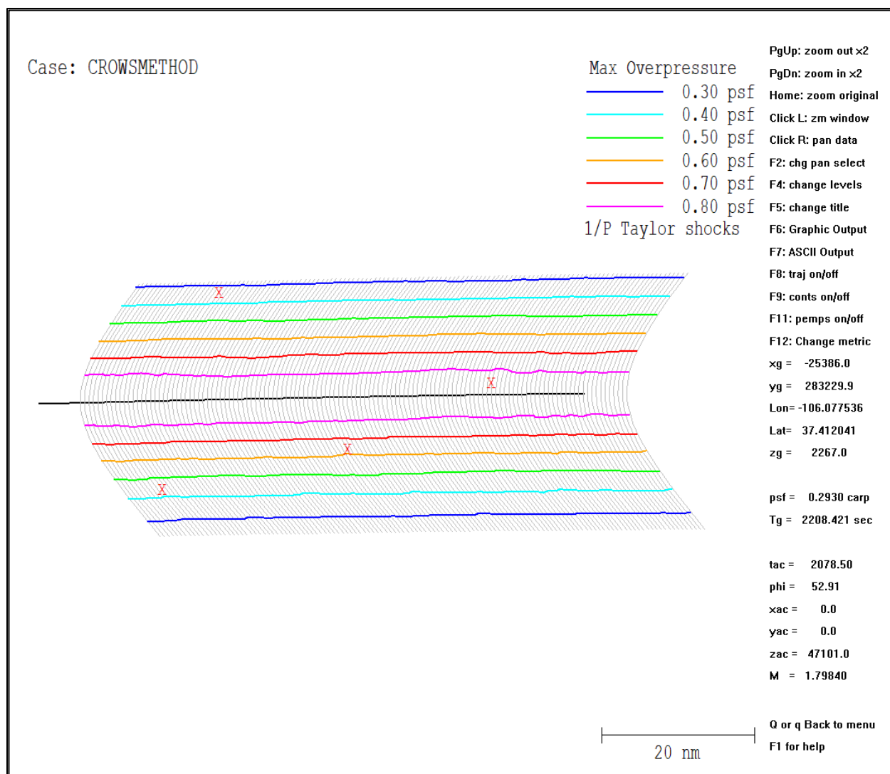
Figure B-39 Crow's method case WCON footprint with marked locations of interest from script file.
