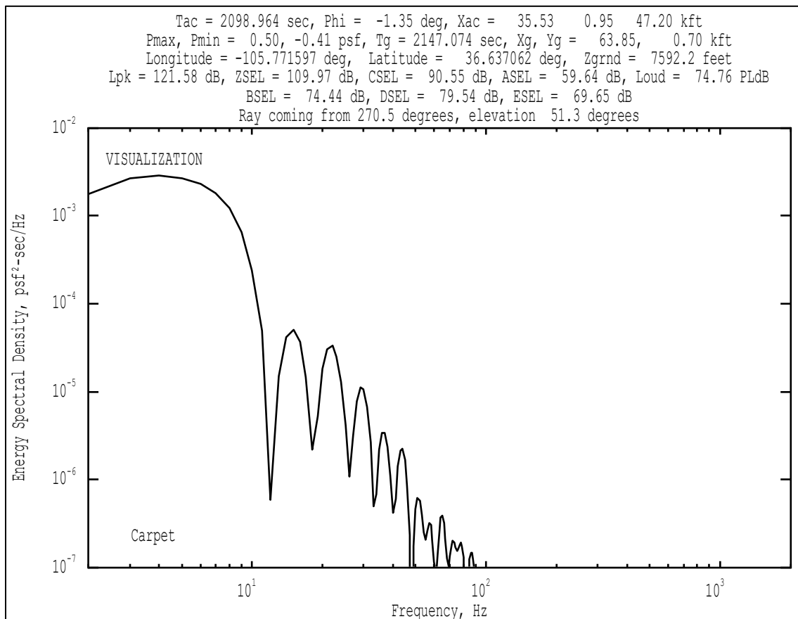
Figure B-10 Visualization case, spectrum display.
