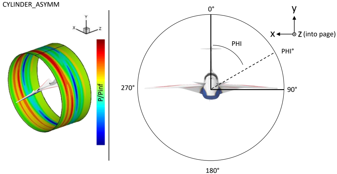
Figure 3-19 CYLINDER_ASYMM coordinate axis definition.
