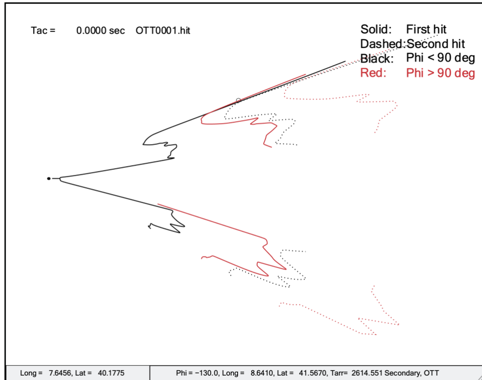
Figure 5-7 POTTI isopemp display.
