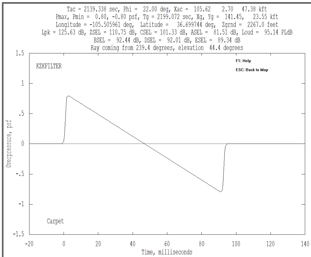
Figure B-32 KZK Filter case WCON signature view example – pre-FIR Filter.
