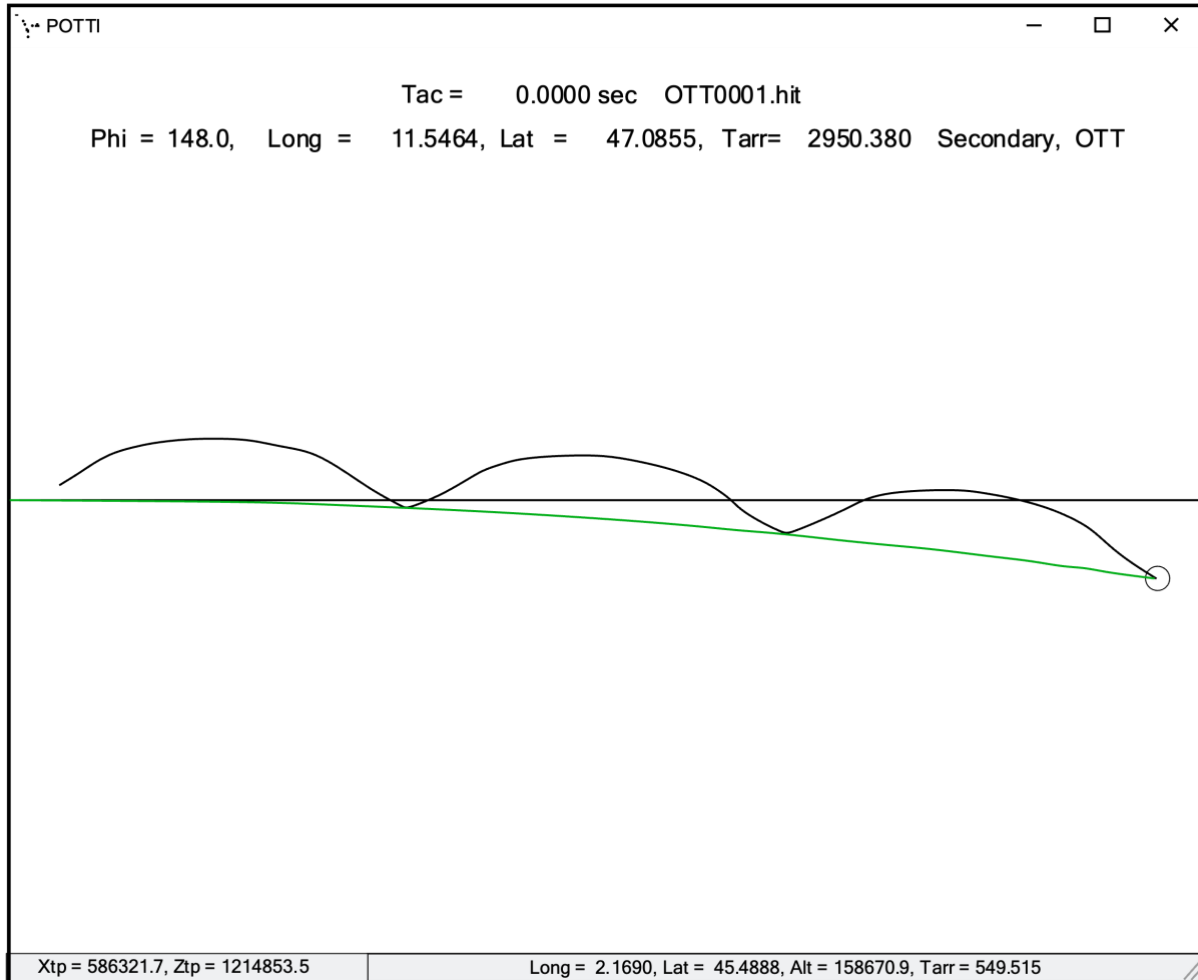
Figure B-76 OTT case POTTI visualization of secondary sonic boom ray bounces from the first trajectory point.
