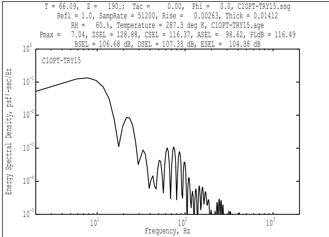
Figure 4-4 Energy spectral density of the Burgers solution at the ground.
