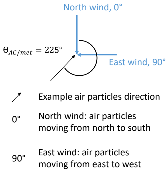
Figure 3-6 Wind angle conventions.
