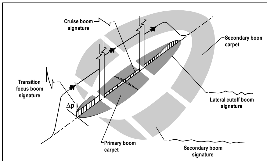
Figure 5-4 Primary and secondary boom carpets. 27
