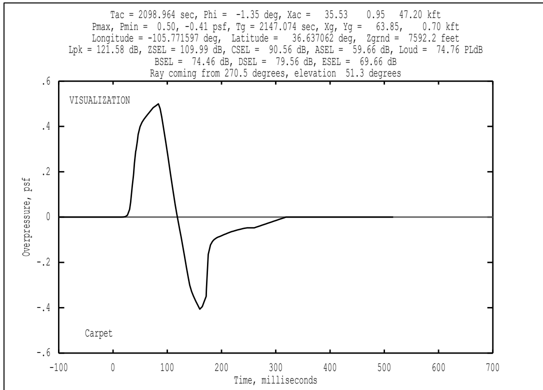
Figure 4-12 Example WCON signature display.
