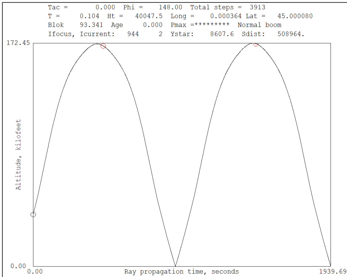
Figure B-78 OTT case OTTER ray path plot.
