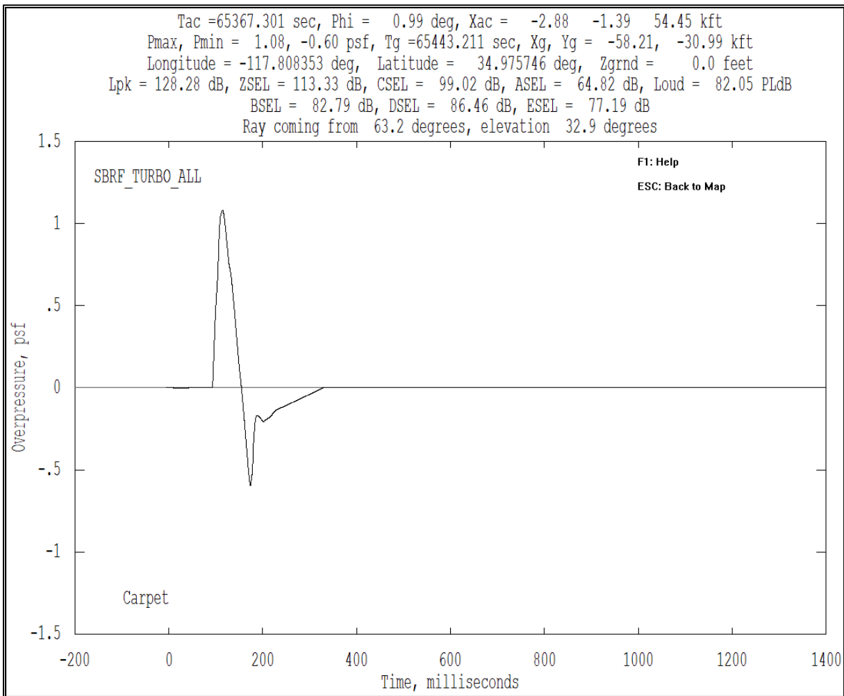
Figure B-50 Turbo case WCON turbulized signature view example.
