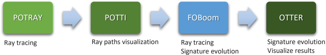
Figure B-72 Over-the-Top/Secondary sonic boom workflow.
