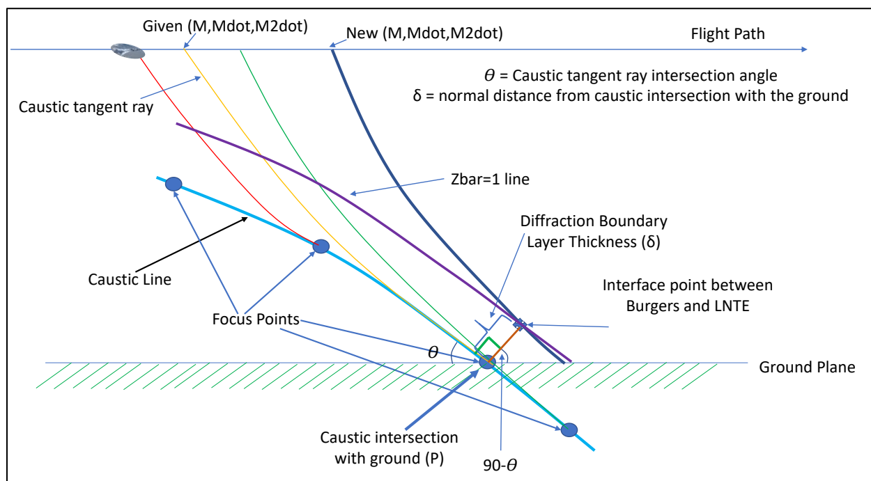
Figure 5-1 Focus delta ray geometry. 24
