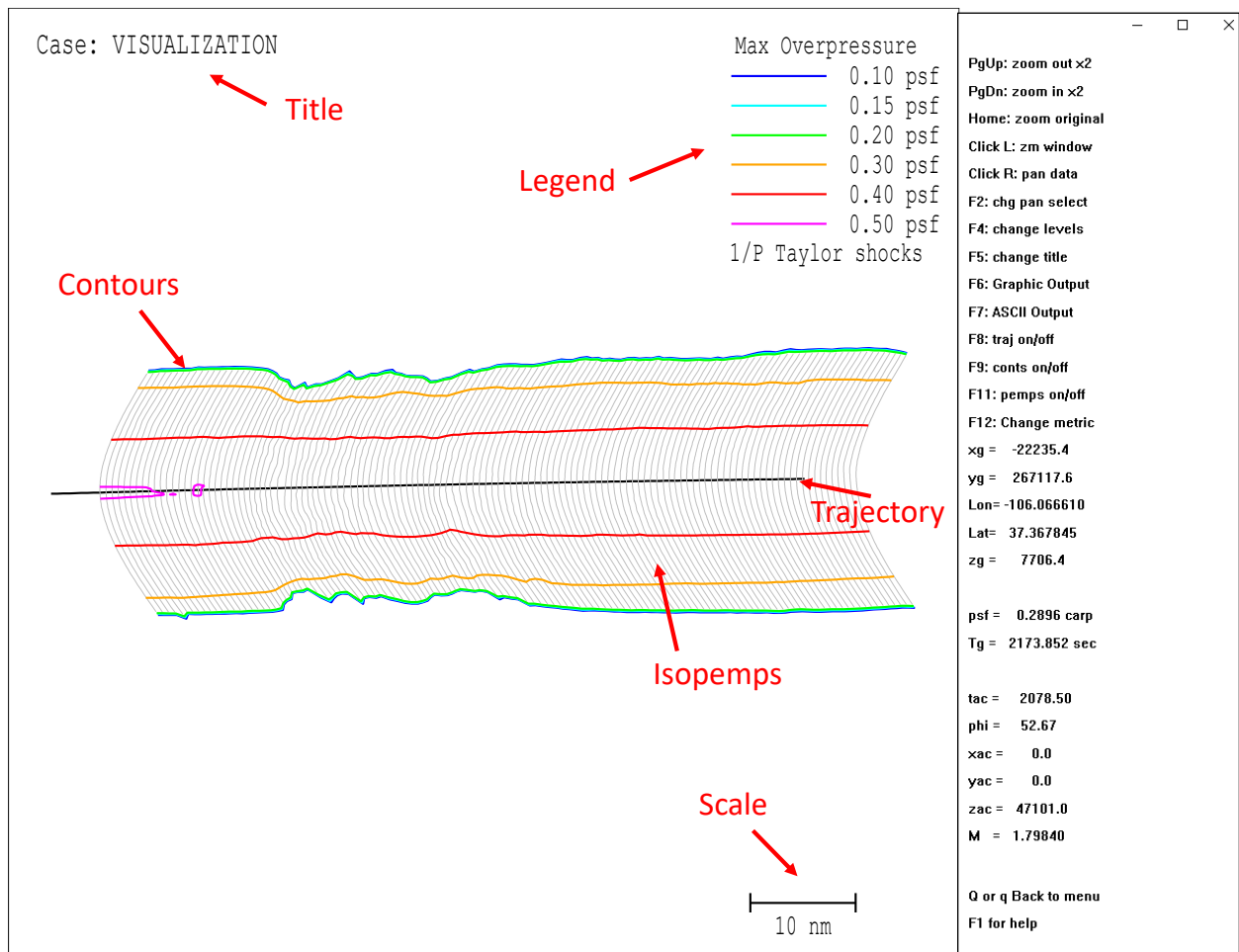
Figure 4-10 WCON footprint main display.
