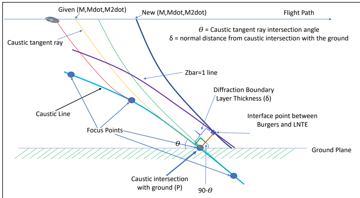
Figure B-55 Focus delta ray geometry. 32
