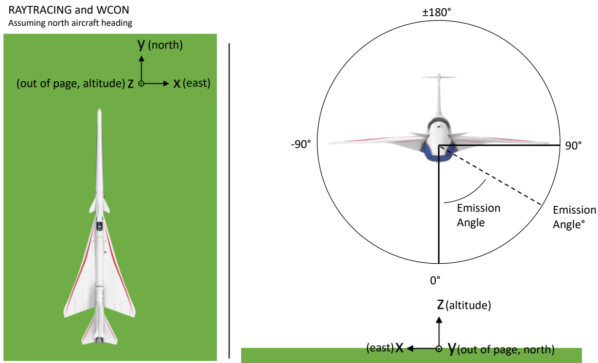
Figure 3-11 RAYTRACING coordinate axis definition.
