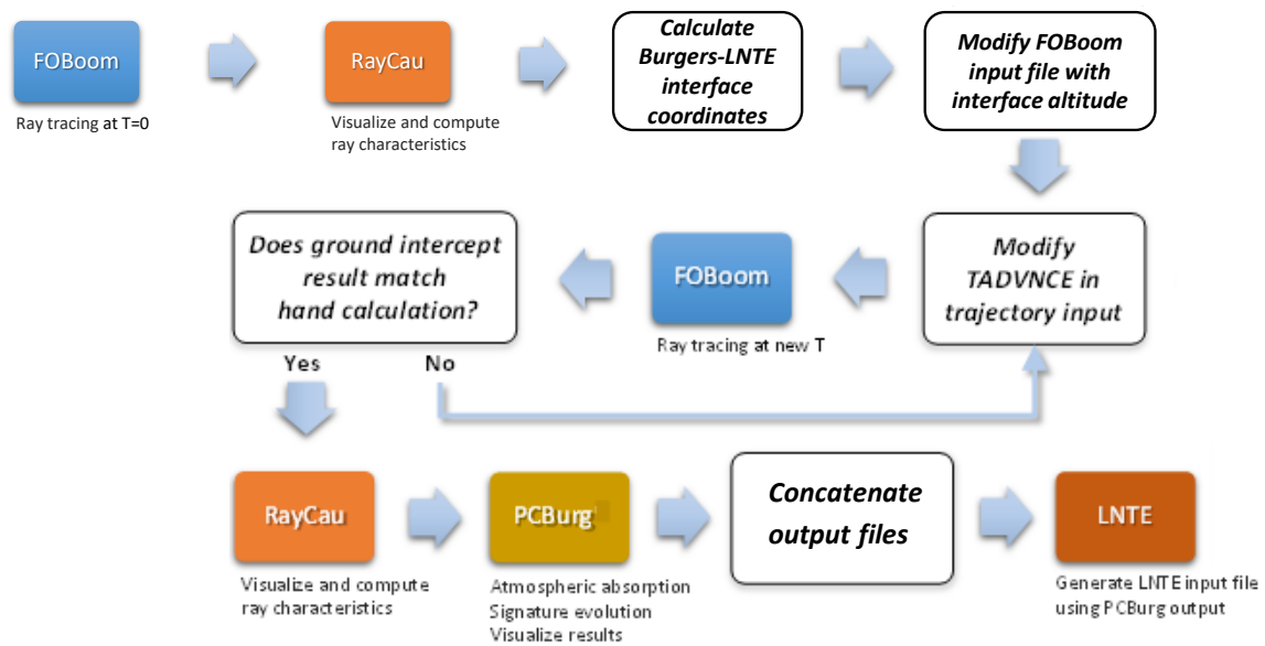
Figure B-56 Focus delta ray solution workflow.
