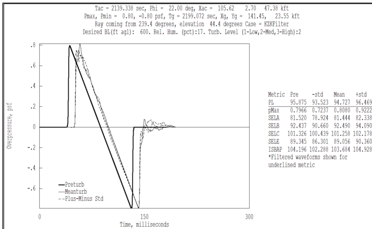
Figure B-34 FiltView interface with turbulized signatures and statistical loudness metrics.
