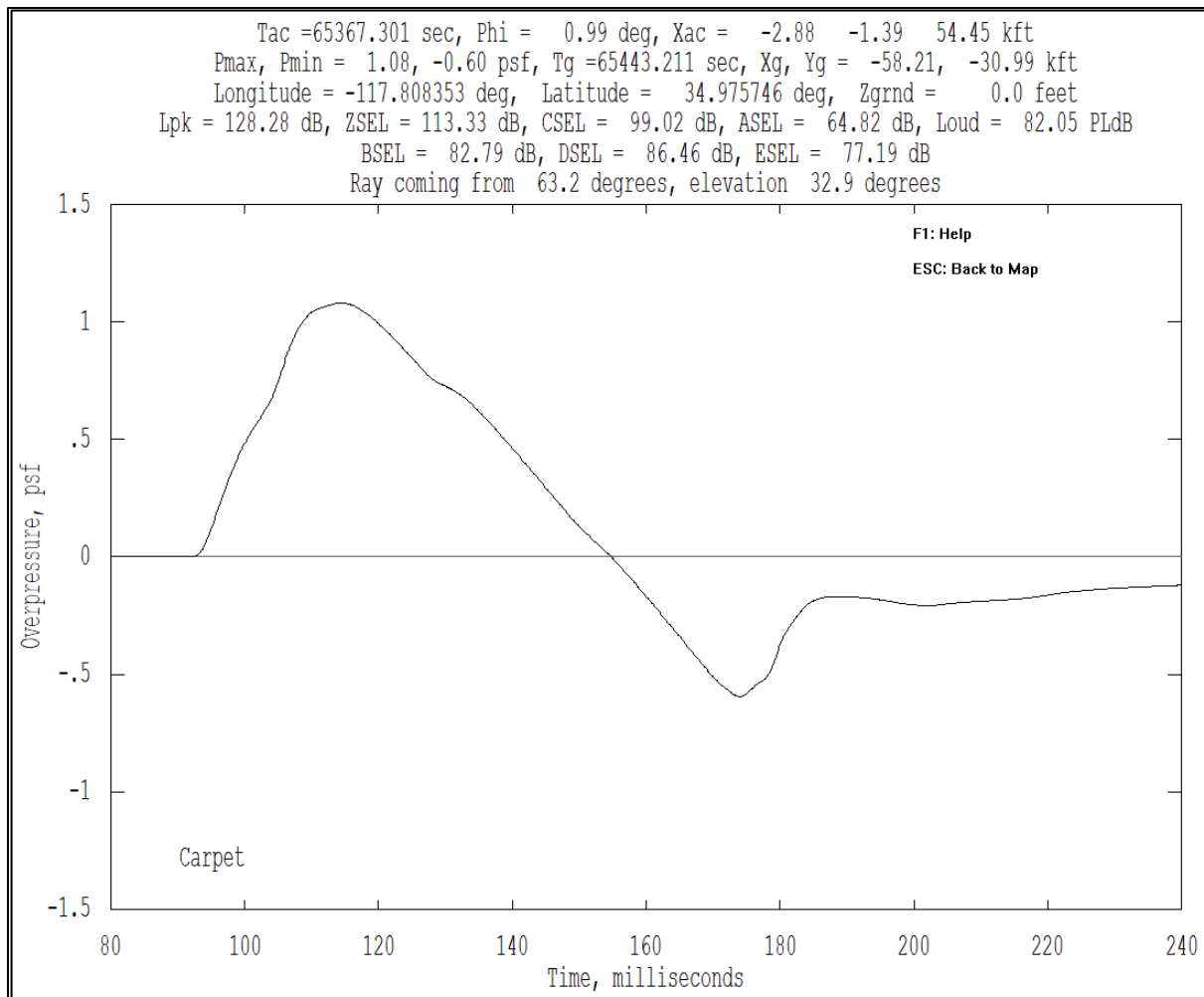
Figure B-51 Turbo case WCON signature view example – time axis zoom in to view turbulized signature.
