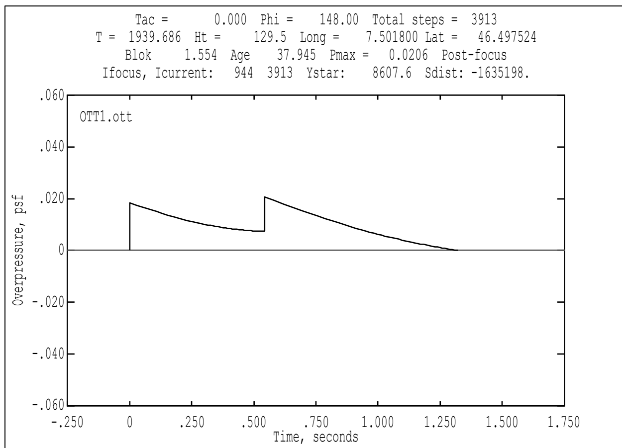
Figure B-81 OTT case OTTER signature view at second bounce point (Over-The-Top Ground Signature).
