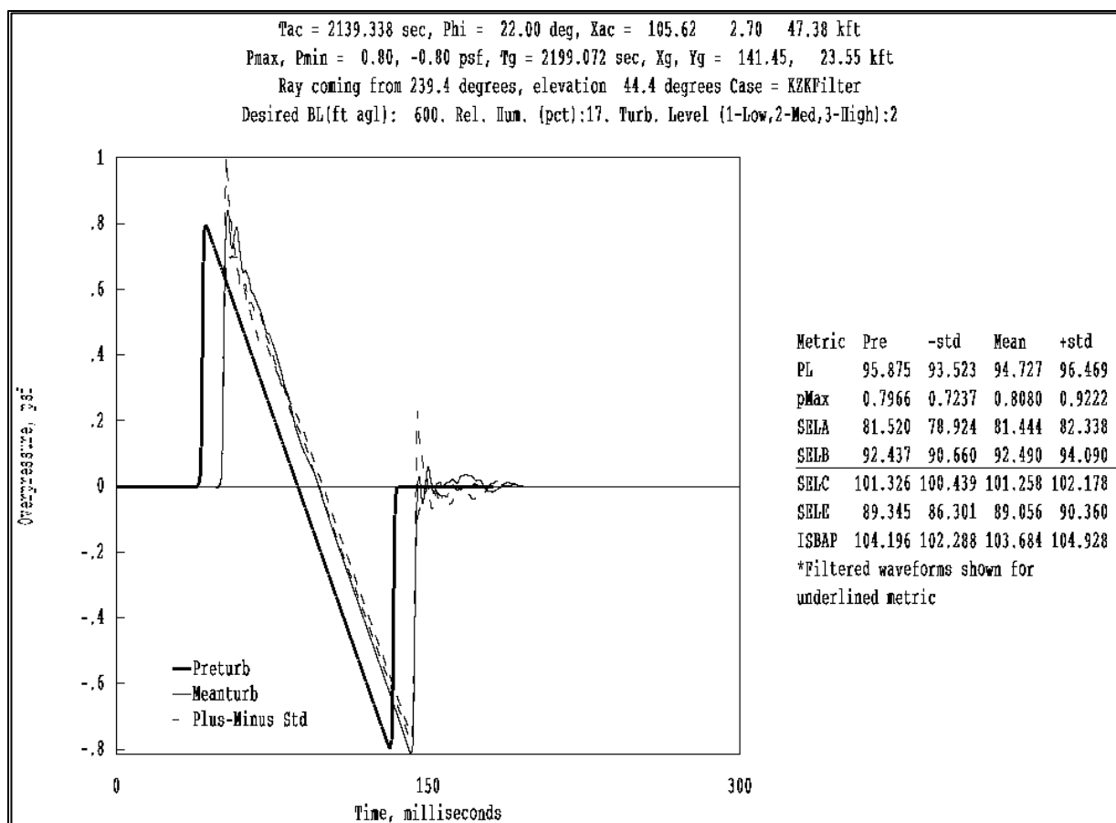
Figure B-35 FiltView interface showing the SELB turbulized waveforms.
