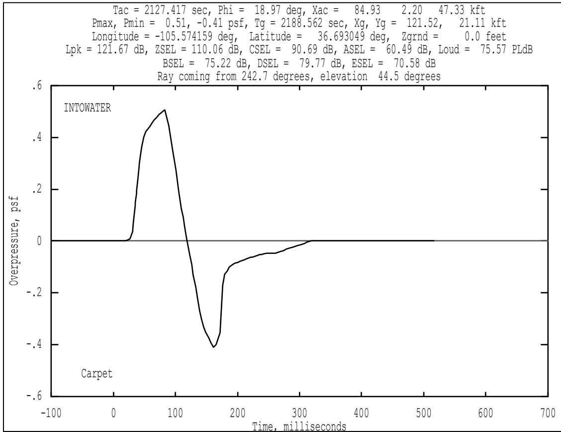
Figure B-23 Example WCON signature view – at water surface.
