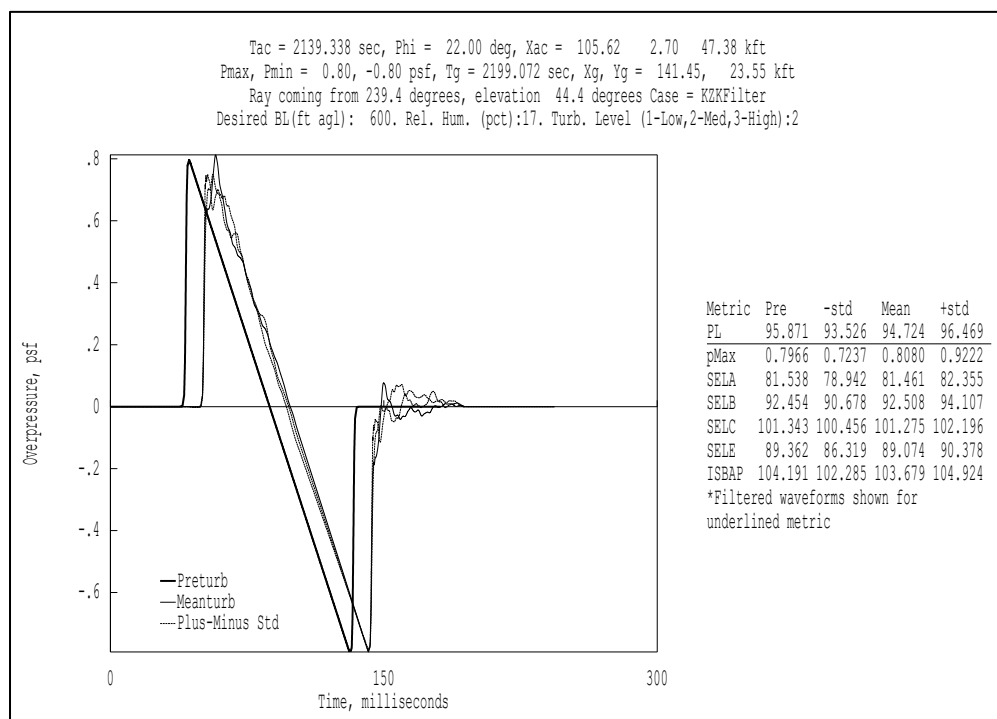
Figure 4-13 Example FiltView display.
