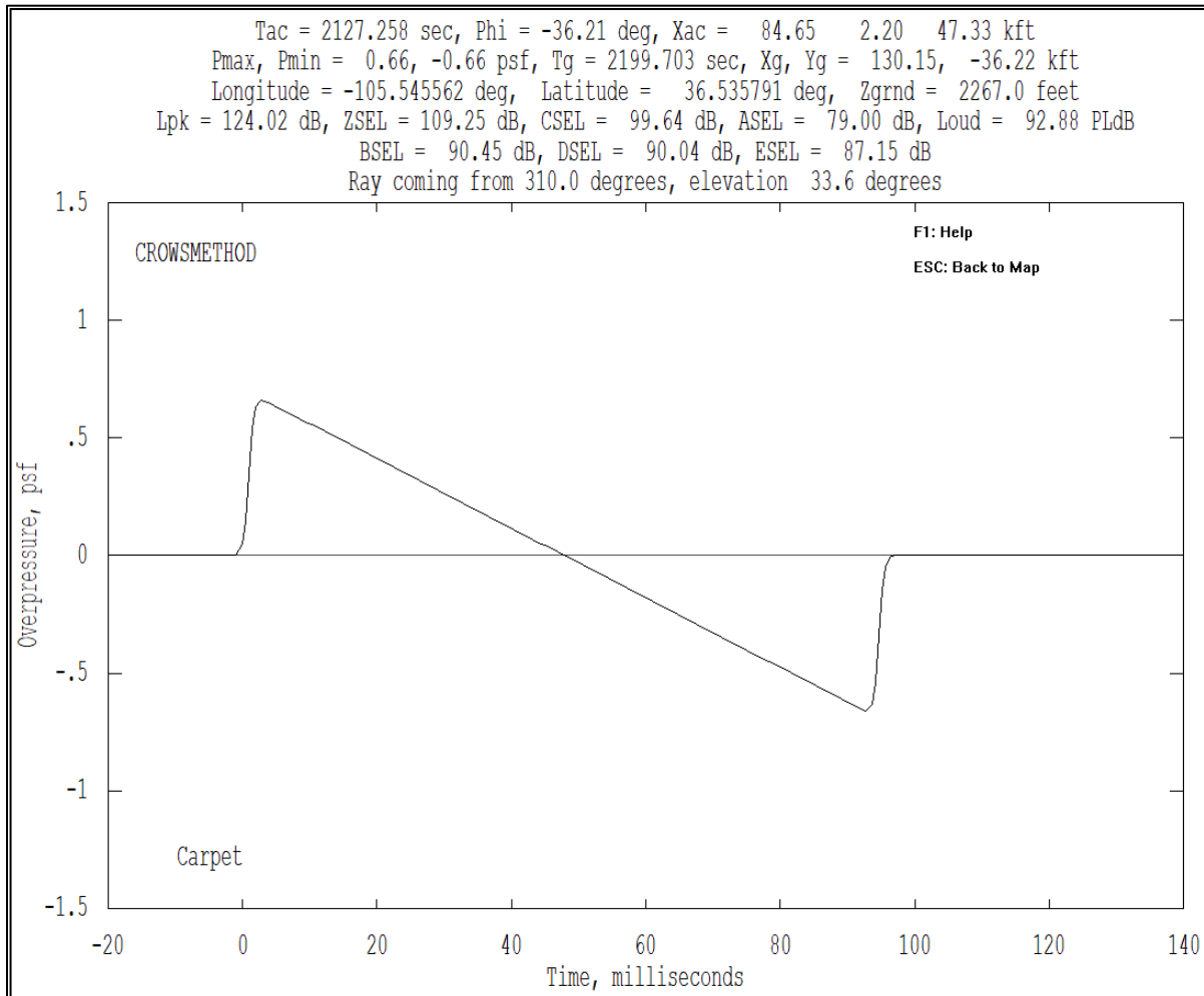
Figure B-41 Crow's method case WCON signature view example – pre-Crow's method envelope.
