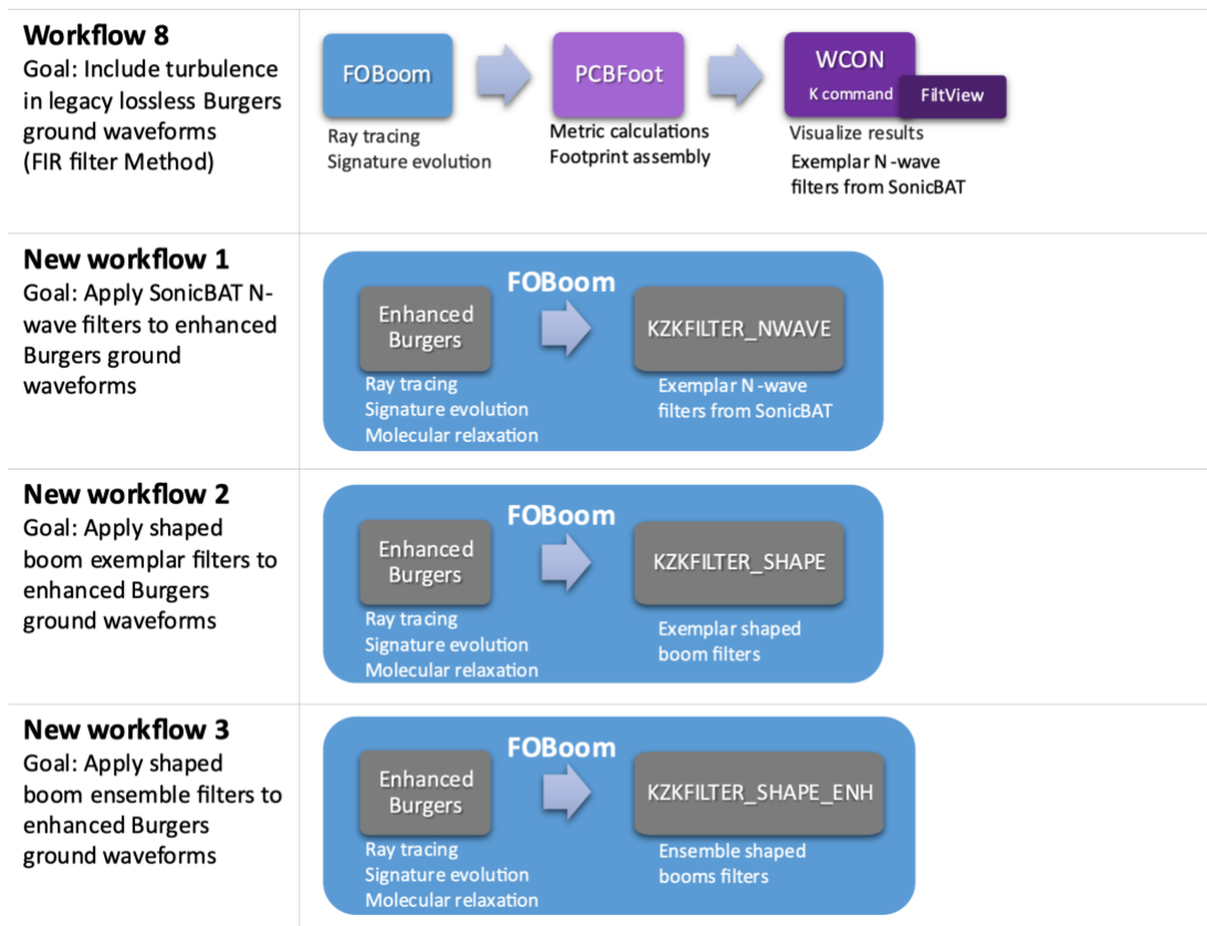
Figure 2-6 Turbulence KZK filter workflows.
