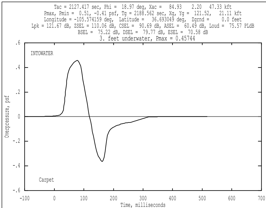
Figure B-24 Example WCON signature view – 3 ft underwater.
