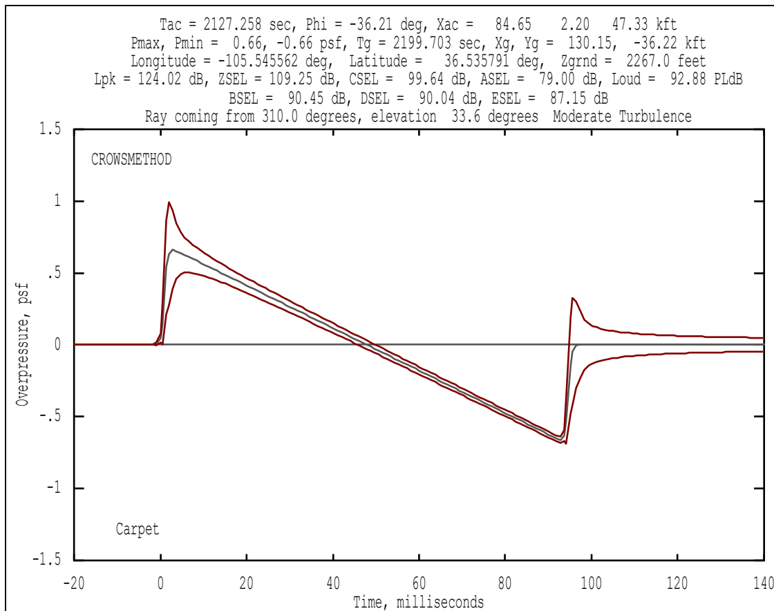
Figure B-42 Crow's filter envelope overlaid on WCON signature view.
