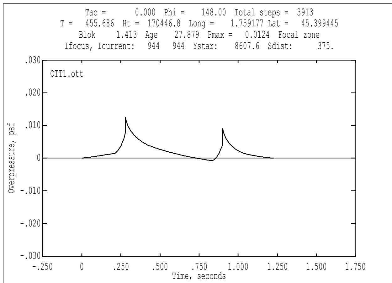
Figure B-79 OTT case OTTER signature view at first focus point.
