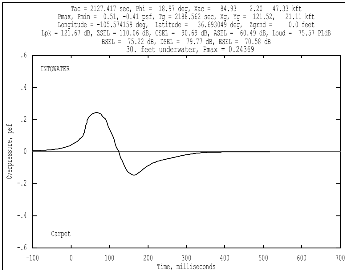
Figure B-25 Example WCON signature view – 30 ft underwater.
