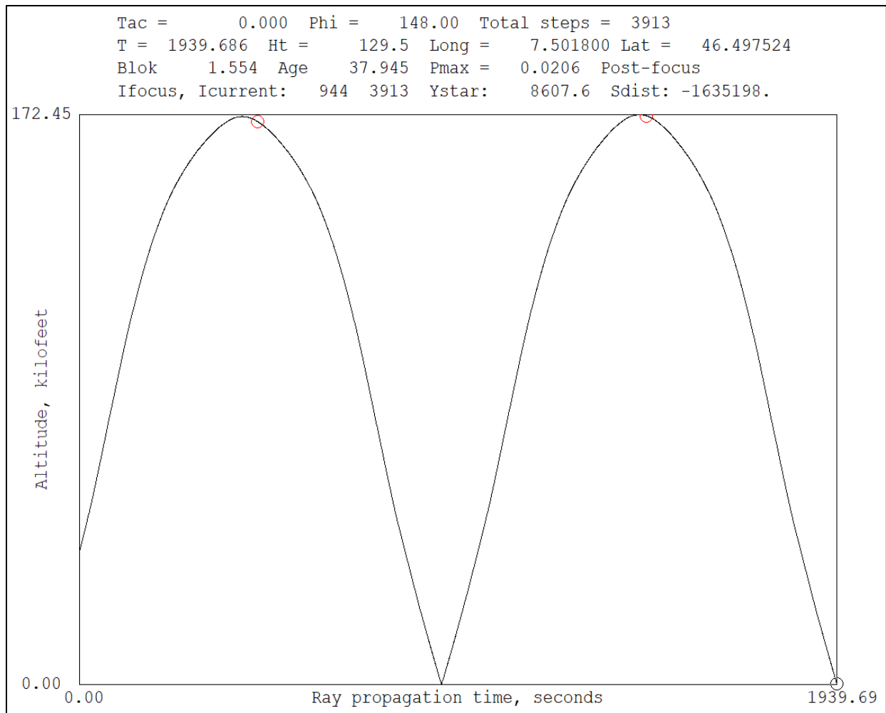
Figure B-80 OTT case OTTER ray path plot with cursor on second bounce (secondary sonic boom).
