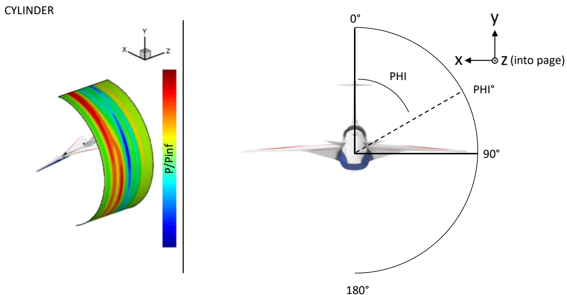
Figure 3-15 CYLINDER coordinate axis definition.
