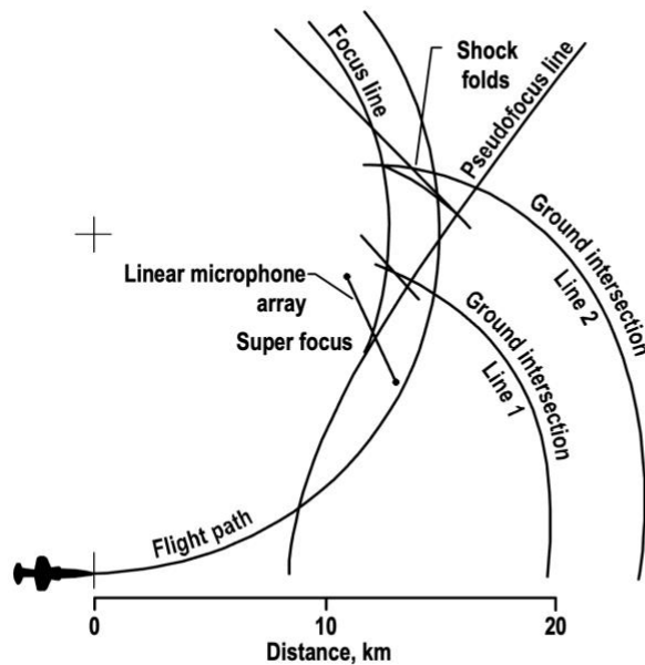
Figure 3-39: Shock Wave Footprint on the Ground in a Turn Entry Maneuver (Source: NASA-SP-622 [7]).
