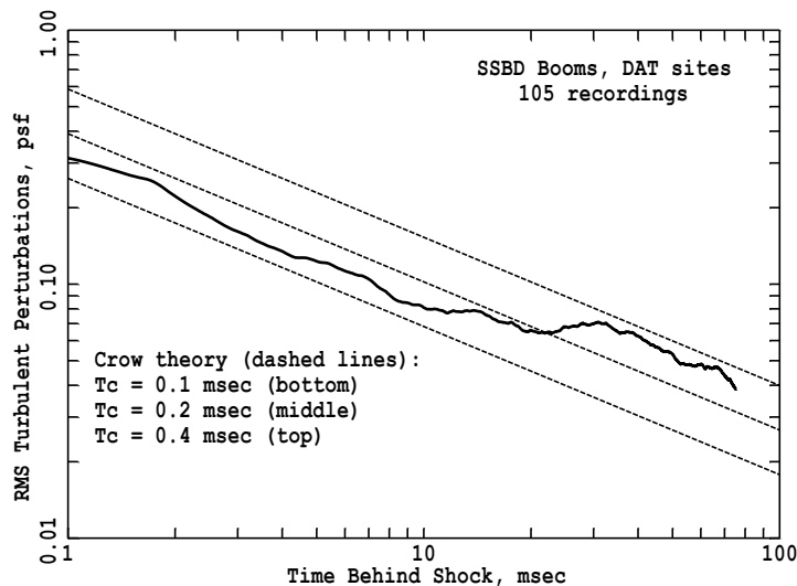
Figure 3-28: RMS Values of SSBD Rear Shock Spiky Fine Structure (Source: Plotkin, Maglieri, Sullivan [43], reprinted with permission).
