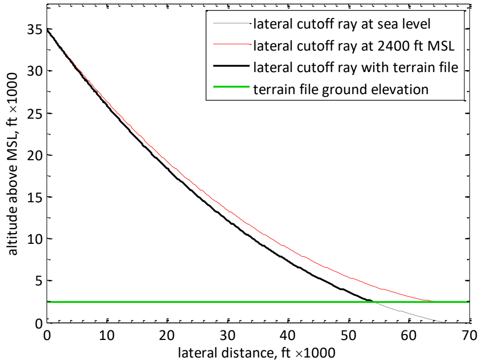
Figure 4-12: Ray Paths at Lateral Cutoff as Determined by FOBoom LEGACY Internal Algorithm.
