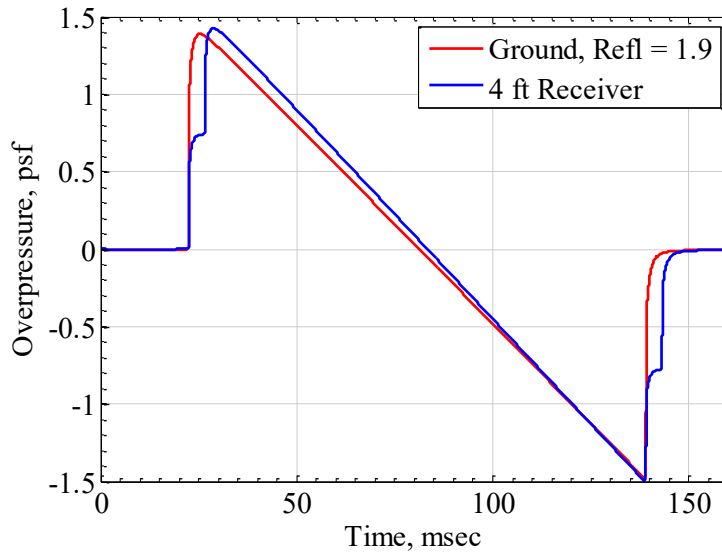
Figure 3-47: Comparison of Ground Waveform Modeling using Simple Reflection Factor = 1.9 and Waveform at Receiver Elevated 4 ft above Ground.
