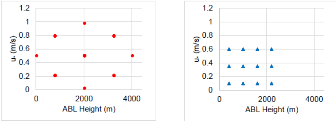
Figure 3-31 Example comparison of u_* and ABL Height design factor points, with space-filling central composite design of the shaped filters on the left and the full-factorial design of the N-wave filters on the right.
