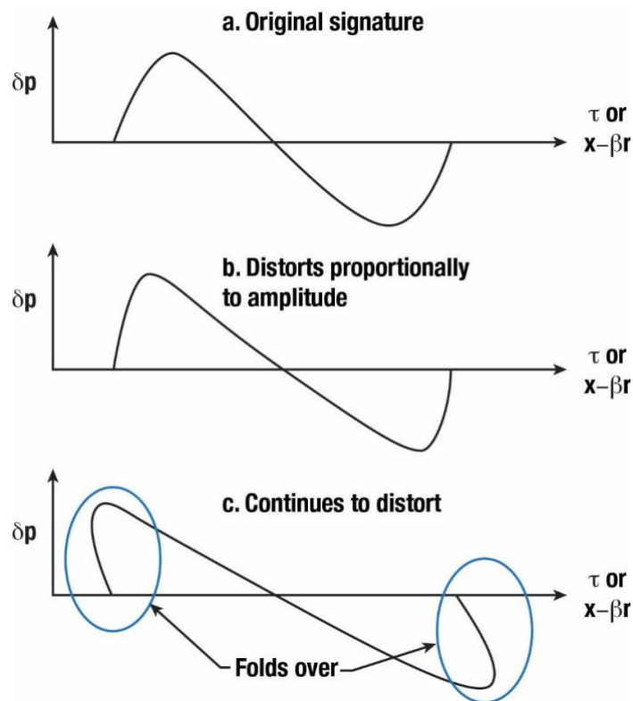
Figure 3-22: Evolution and Steepening of Sonic Boom Signatures (Source: NASA-SP-622 [7]).
