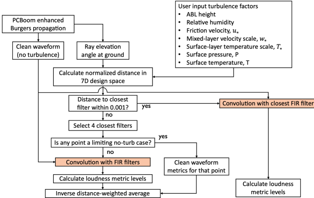
Figure 4-8: Flowchart illustrating the PCBoom process implementing regular and enhanced shaped boom filters.
