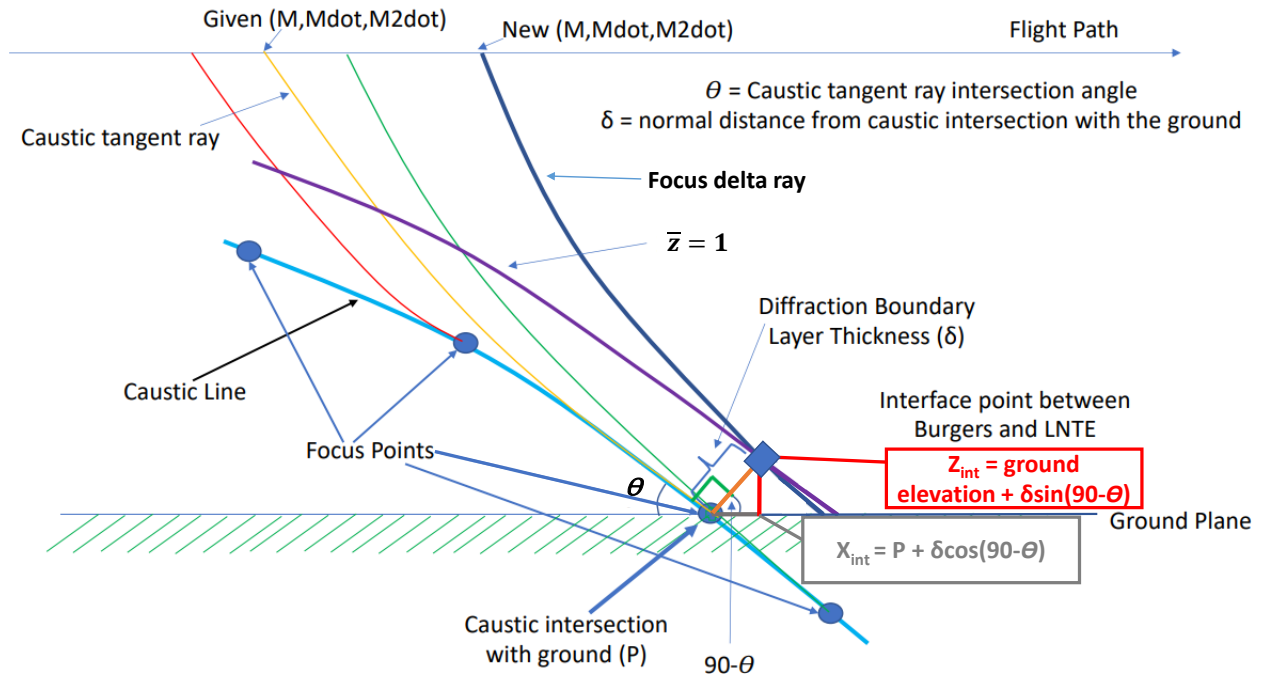
Figure 6-4: Geometric Interface between Ray Tracing and LNTE (Source: Adapted from Rallabhandi [112]).
