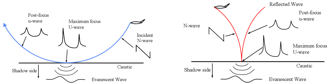
Figure 3-43: Focus at a Cutoff Caustic. Atmosphere fixed frame (left) and wave fixed frame (right) (Source: Plotkin, Page, and Haering [5]; reprinted with permission).
