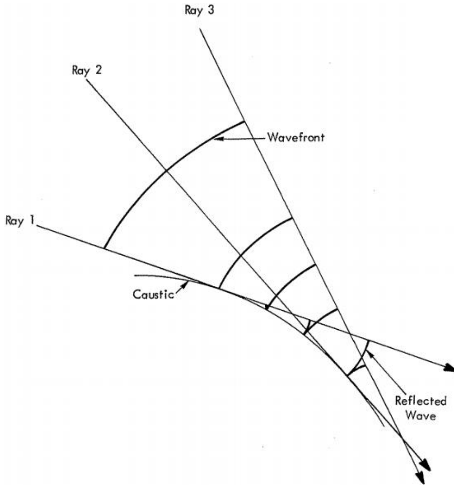
Figure 3-34: Ray Geometry and Wavefront Folding (Reflection) at a Caustic (Source: Plotkin and Cantril, "Prediction of Sonic Boom at a Focus," [2]; reprinted by permission of the American Institute of Aeronautics and Astronautics, Inc.).
