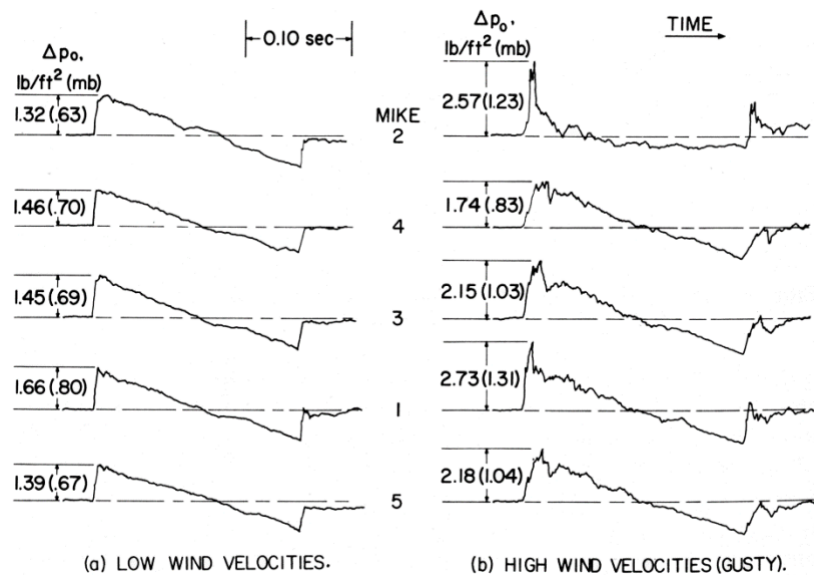
Figure 3-25: Sonic Booms Measured Under Calm and Turbulent Conditions (Source: NASA TN D-3655 [46]).
