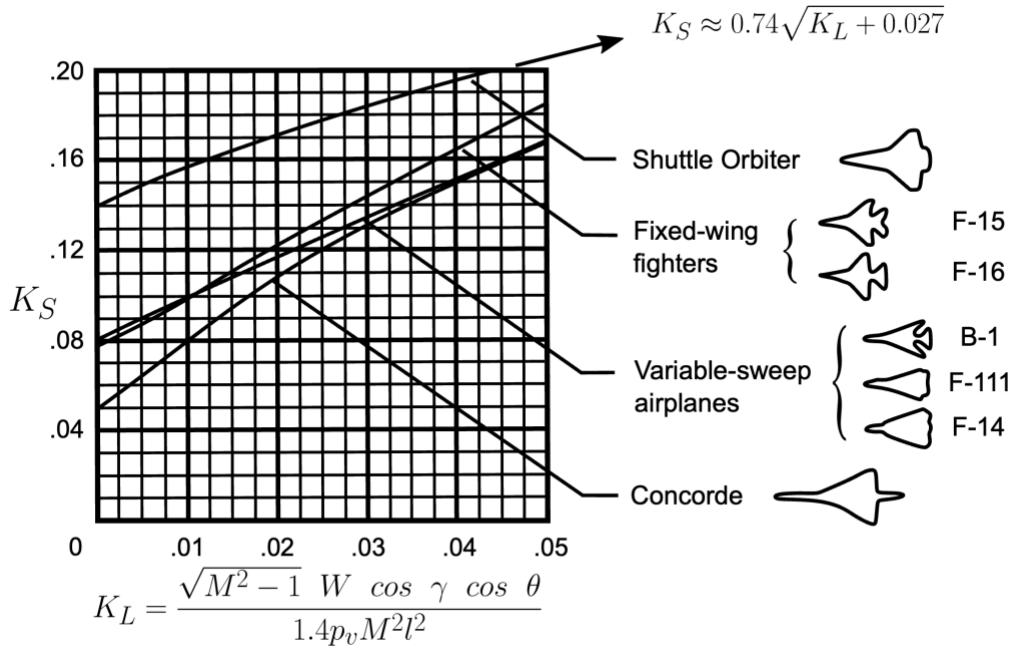
Figure 4-9: Carlson Representative Aircraft Shape Factors ( K_S ) as a function of Lift Parameter ( K_L ) (Source: NASA TP 1122. Carlson [9]).
