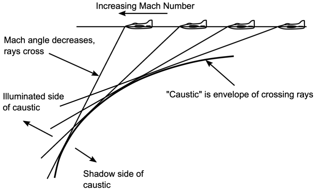
Figure 3-36: Caustic Due to Acceleration (Source: NASA-CR-218871 [69]).
