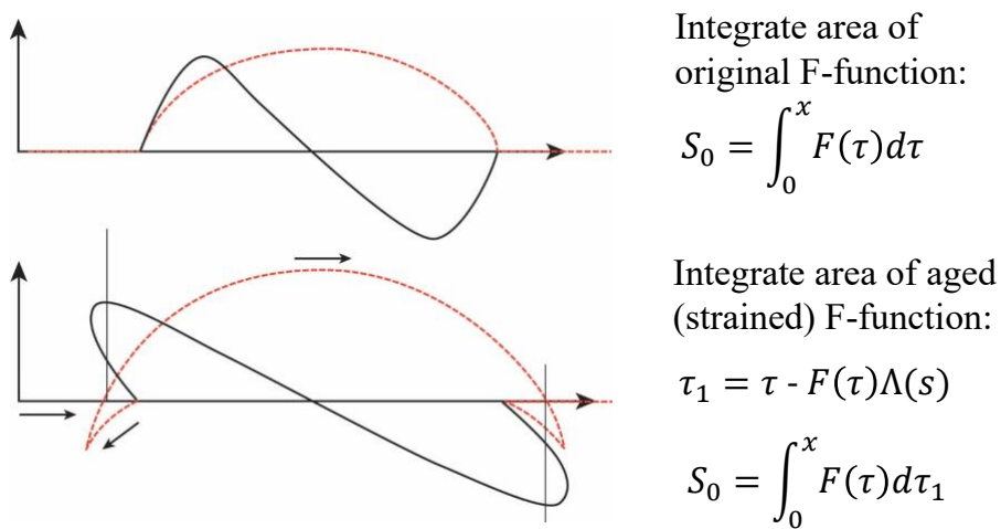
Figure 3-23: Middleton–Carlson Aging Method (Source: NASA-SP-622 [7]).
