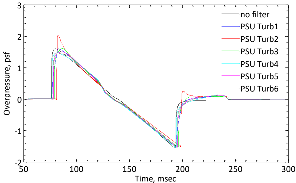
Figure 3-30: Modeled F-18 Ground Signature with Turbulence Filters Applied.
