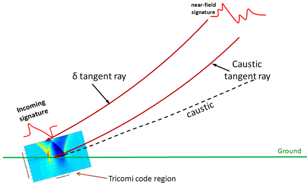
Figure 6-3: Rays, Caustic, and Focal zone (Source: NASA-CR-218871 [69]).
