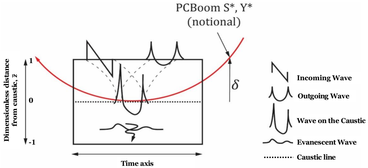
Figure 6-2: Focal Zone as Defined by the Tricomi Solution Region, with Tangent Ray Shown (Source: Adapted from Auger and Coulouvrat [98] and Salamone [111], with permissions, and NASA-CR-218871 [69]).
