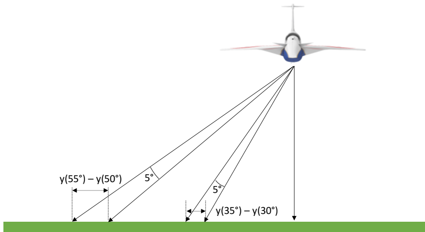
Figure 4-11: Differences in Lateral Ground Intersection Points for Pairs of Rays Separated by 5^\circ .
