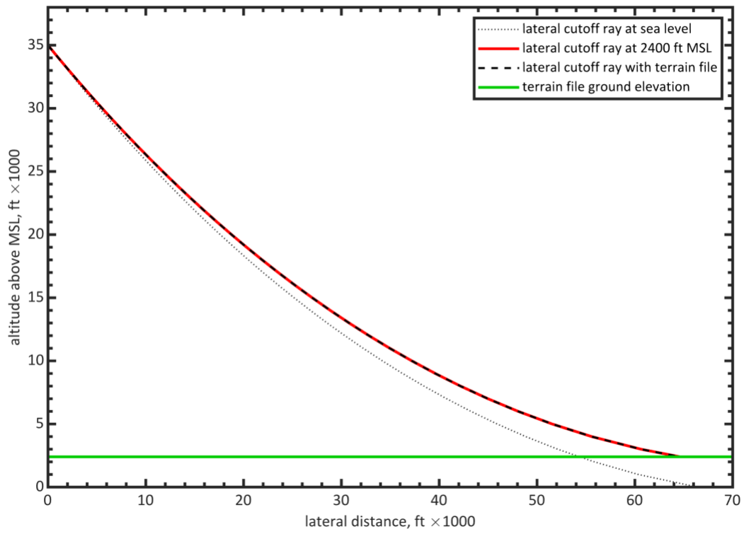
Figure 4-13: Ray Paths at Lateral Cutoff as Determined by FOBoom Schulten Internal Algorithm.
