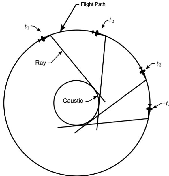
Figure 3-33: Caustic Geometry for a Steady Turn in a Uniform Atmosphere (Source: Plotkin and Cantril, "Prediction of Sonic Boom at a Focus," [2]; reprinted by permission of the American Institute of Aeronautics and Astronautics, Inc.).
