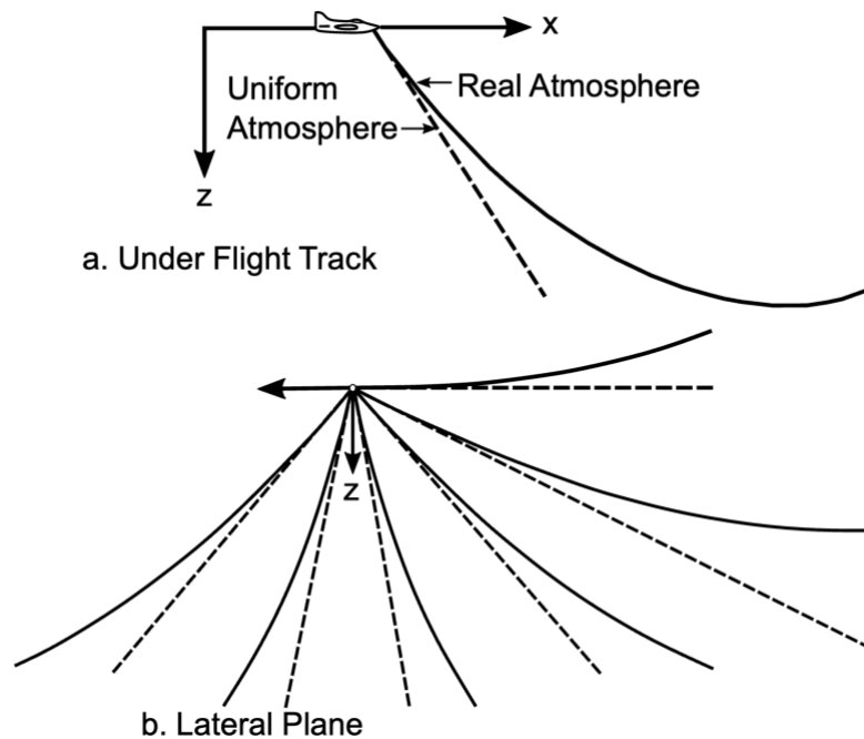
Figure 3-35 Ray Curvature in a Real Atmosphere. (Source: Plotkin [12], reprinted with permission).
