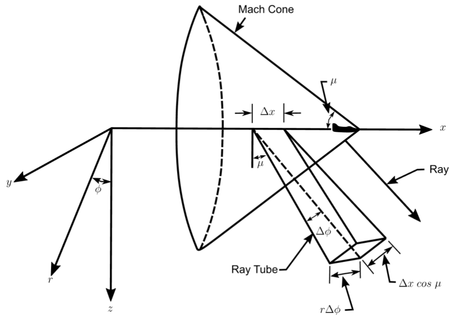
Figure 3-32: Mach Cone, Ray, and Ray Tube for Steady Level Supersonic Flight in a Uniform Atmosphere.
