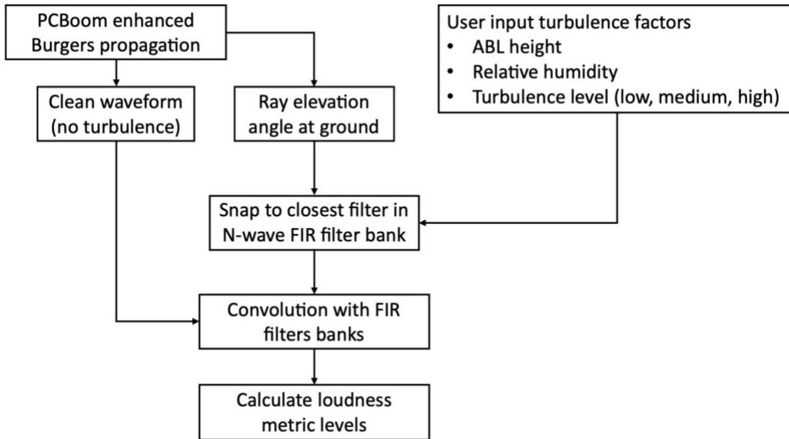
Figure 4-7: Flowchart illustrating the PCBoom process implementing N-wave filters.
