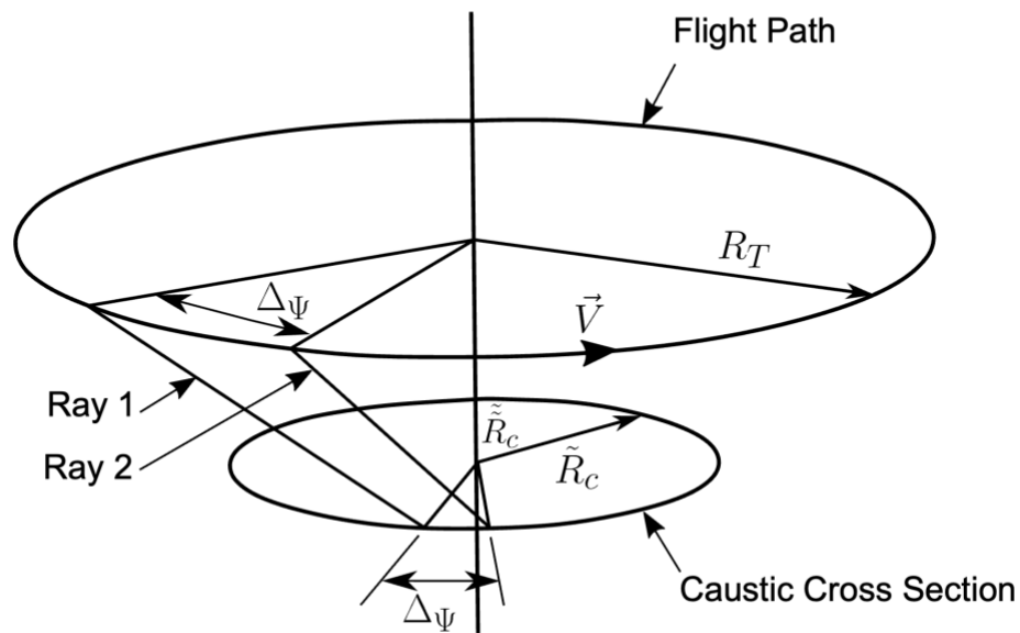
Figure 3-40: Two Successive Rays at Fixed Azimuth in a Steady Turn.
