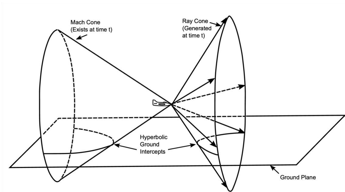
Figure 3-5: Wave and Ray Viewpoints for Steady Flight (Source: Plotkin [12], reprinted with permission).
