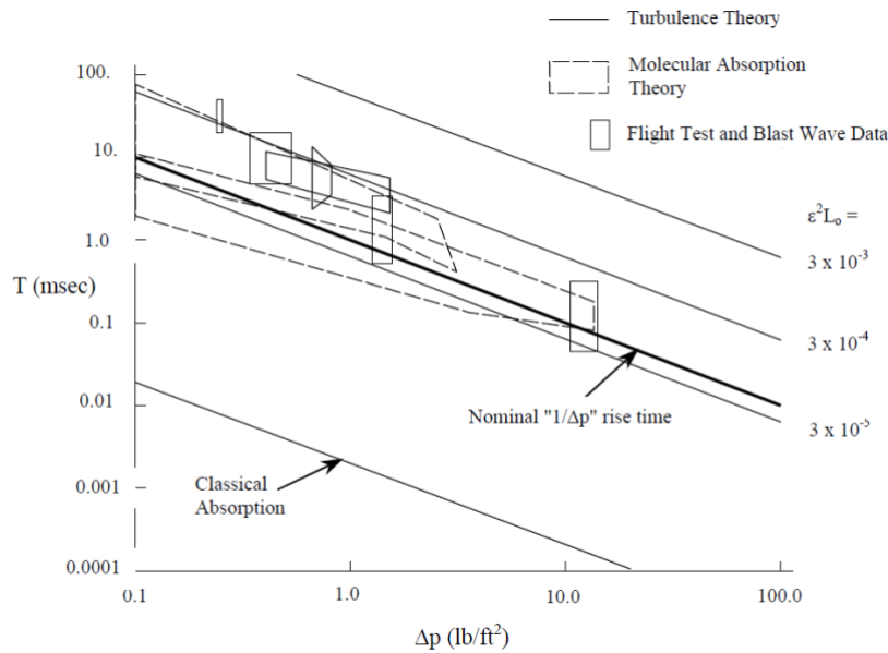
Figure 3-24: Shock Wave Rise Time, Theories, and Applied Model (Source: Adapted from Plotkin [12], reprinted with permission).
