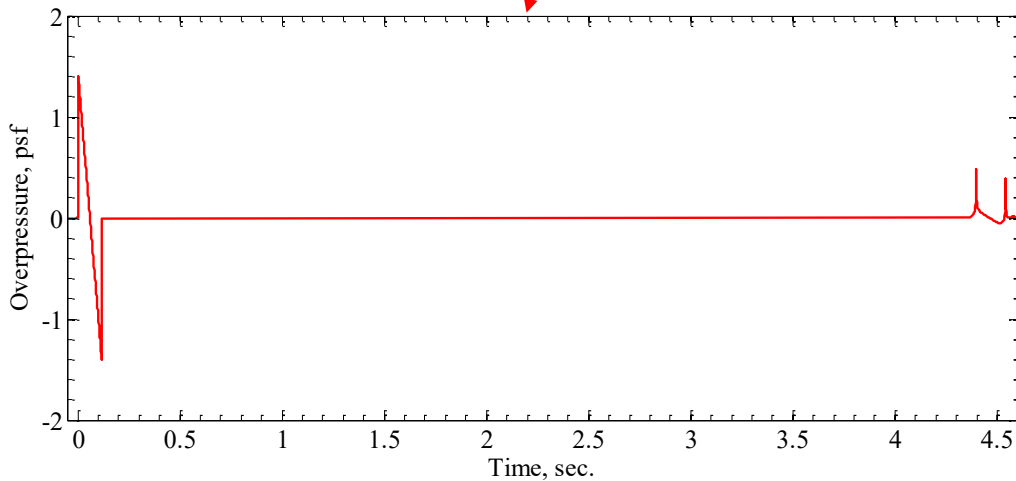
Figure 3-48: Sonic Boom Carpet for Maneuvering Flight (top) and Combined Ground Signature Showing Contributions from Two Ground Booms (bottom).
