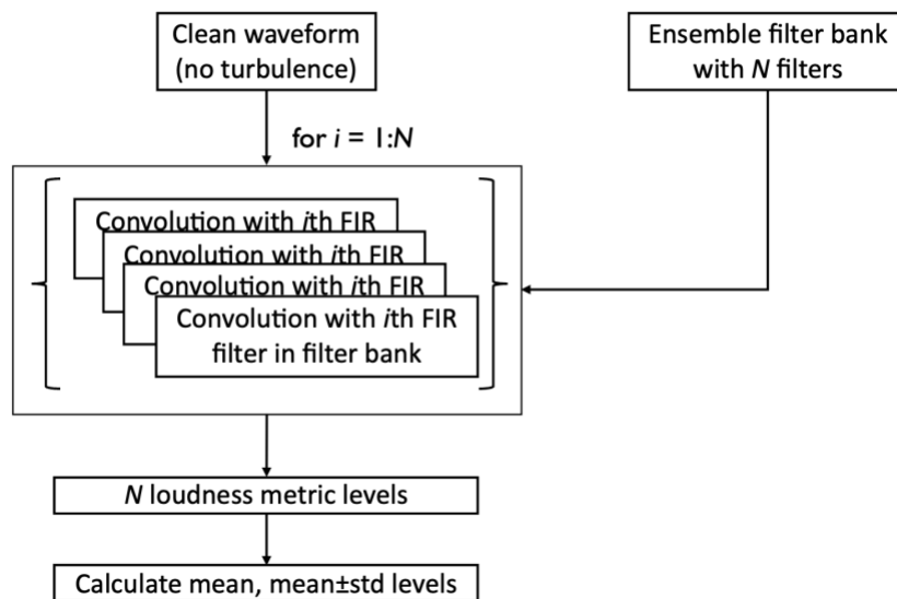
Figure 4-6: Enhanced filter convolution process.
