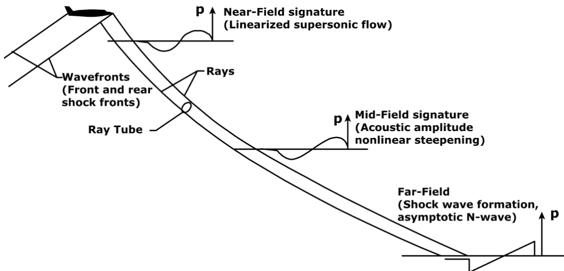
Figure 3-12: Schematic of Sonic Boom Propagation (Source: NASA-SP-622 [7]).
