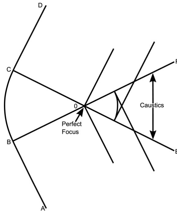
Figure 3-38: Perfect Focus of a Hypothetical Wavefront (Source: Plotkin and Cantril, "Prediction of Sonic Boom at a Focus," [2]; reprinted by permission of the American Institute of Aeronautics and Astronautics, Inc.).
