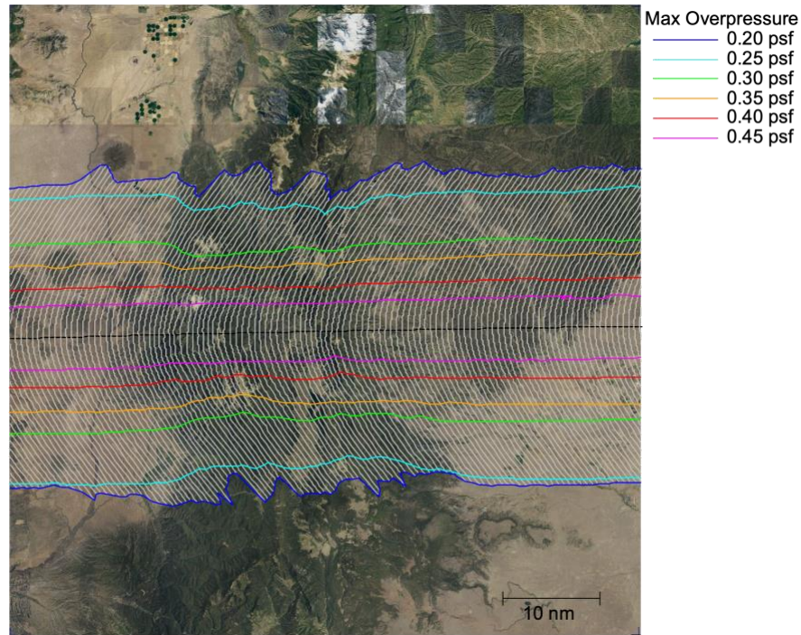
Figure 3-45: Example of Sonic Boom Propagation over Mountainous Terrain (See also Rachami et al. [74]).
