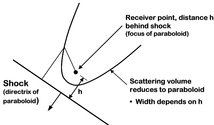
Figure 3-27: Scattering Volume for Thin Shock: Paraboloid of Dependence (Source: Plotkin, Maglieri, and Sullivan [43], reprinted with permission).
