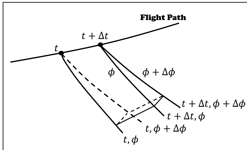
Figure 4-10: Ray Tube Outlined by Four Corner Rays \Delta t and \Delta\phi apart (Source: Plotkin [12]; reprinted with permission).
