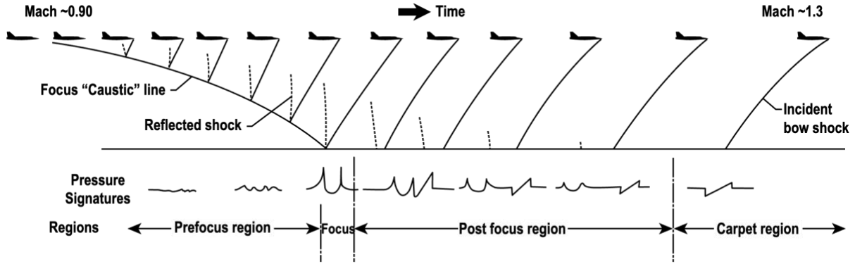
Figure 3-44: Pressure signatures along ground track for aircraft in transition flight (Source: NASA-SP-622 [7]).
