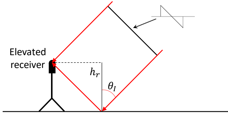
Figure 3-46: Plane Wave Ground Model Geometry.
