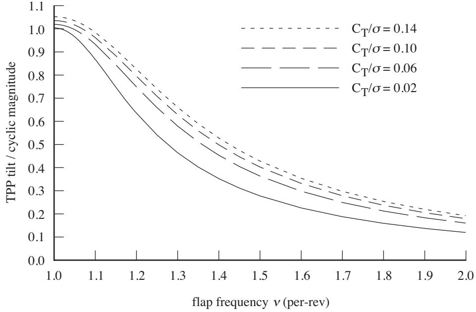
Figure 12-3a. Tip-path plane tilt with cyclic pitch.
