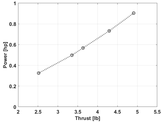
Figure 23. Orb rotor - power vs. thrust at forward speed of 32.8 ft/s.
