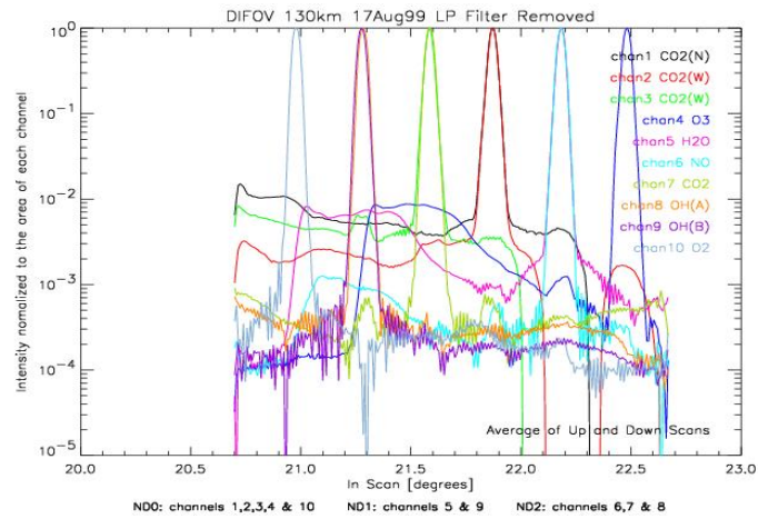
Figure 2. SABER In-Scan IFOV
