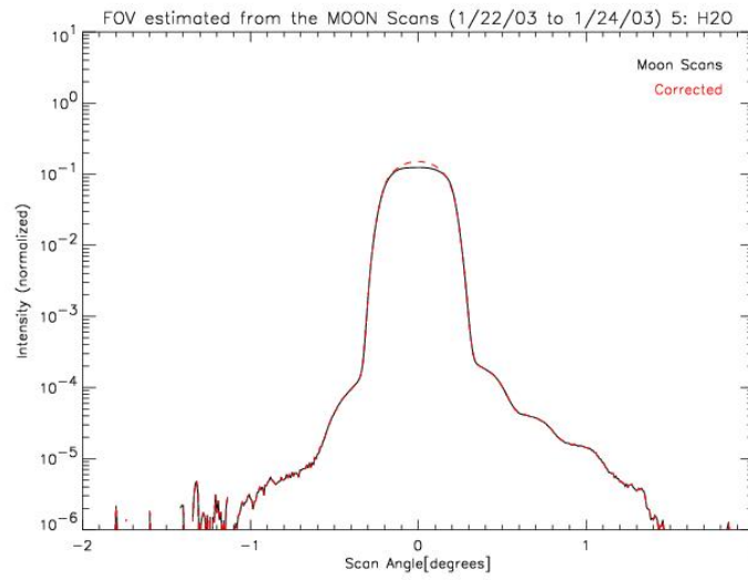
Figure 5. Channel Saturation in Lunar Observation
