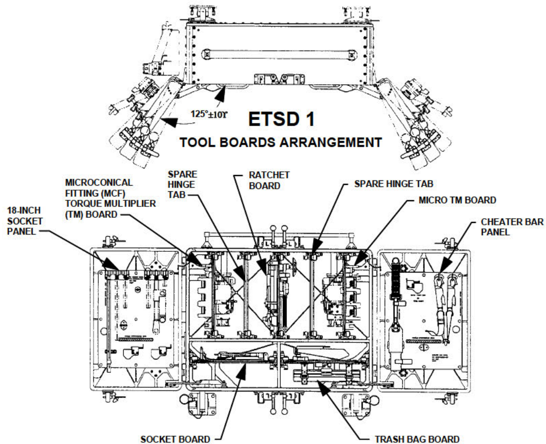
Figure 11-17. Tool box
