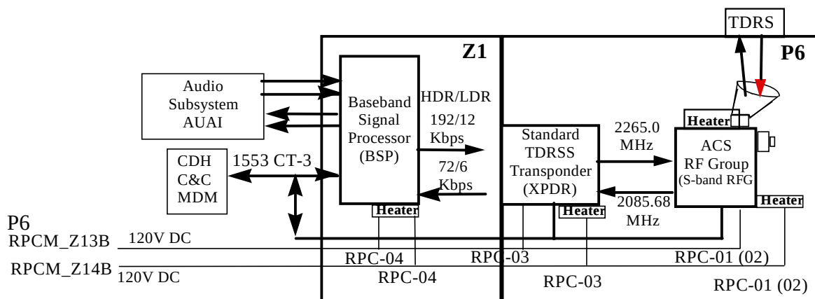
Figure 4-6. S-band overview
