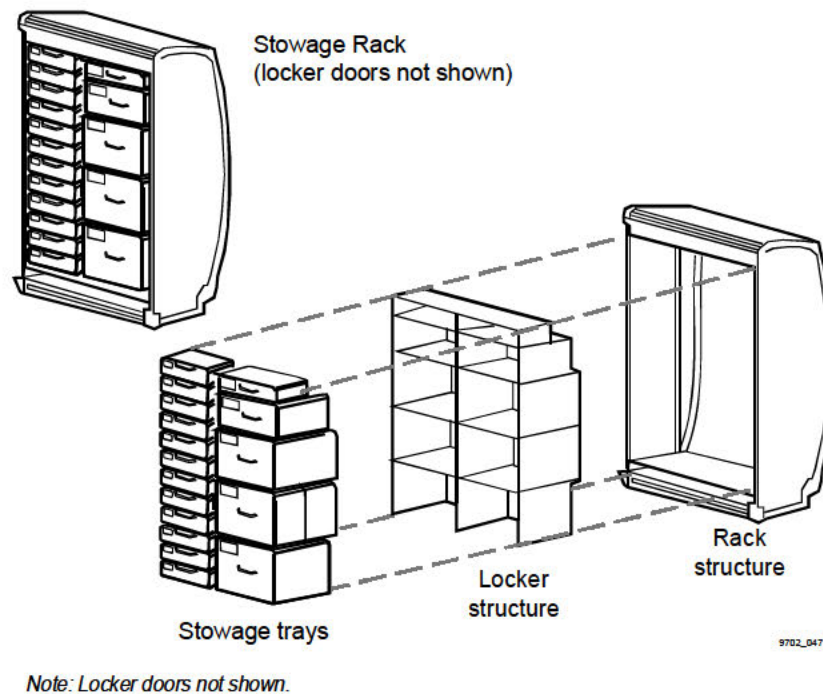
Figure 13-14. Stowage rack
