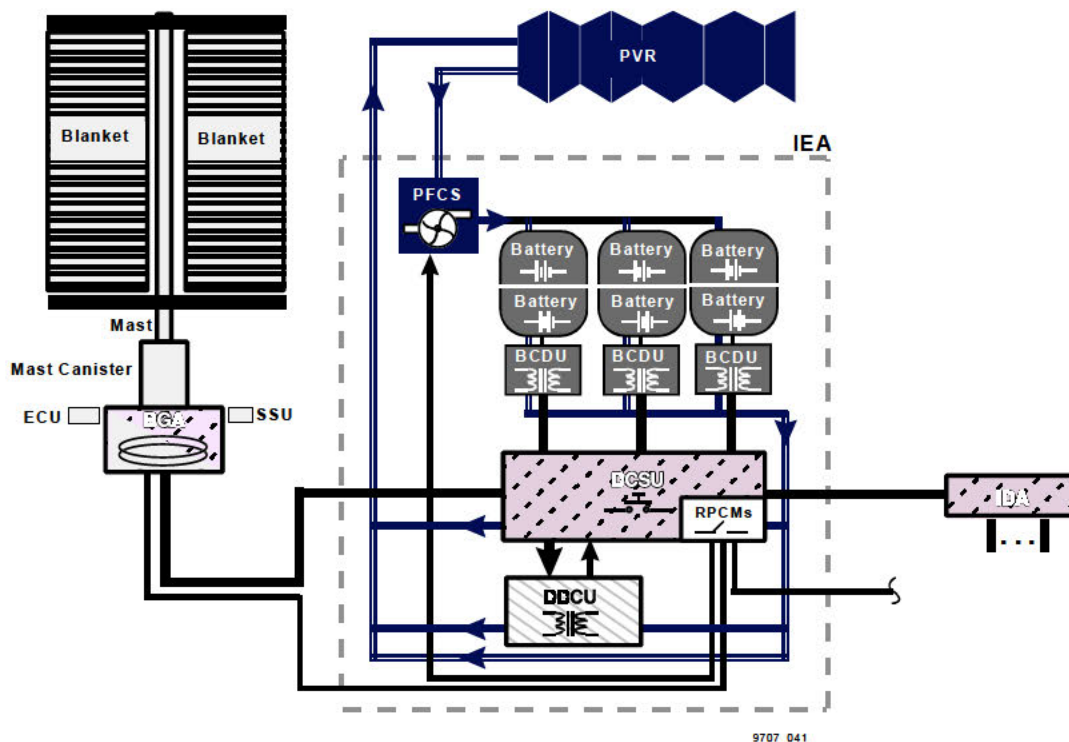
Figure 3-5. USOS EPS power channel
