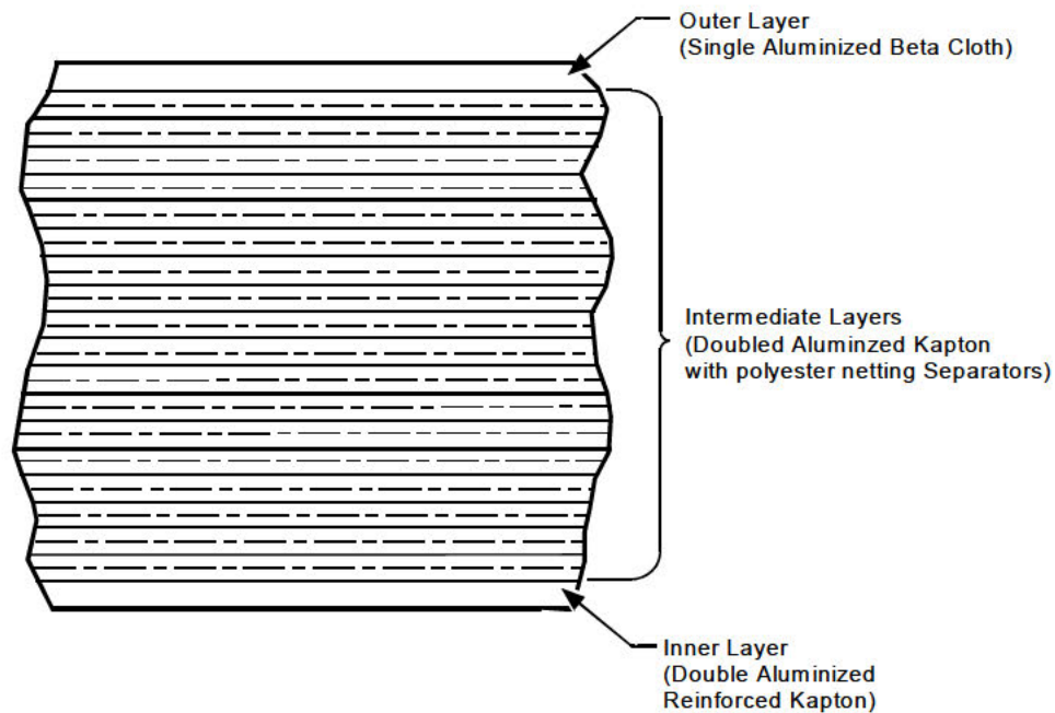
Figure 5-2. MLI design
