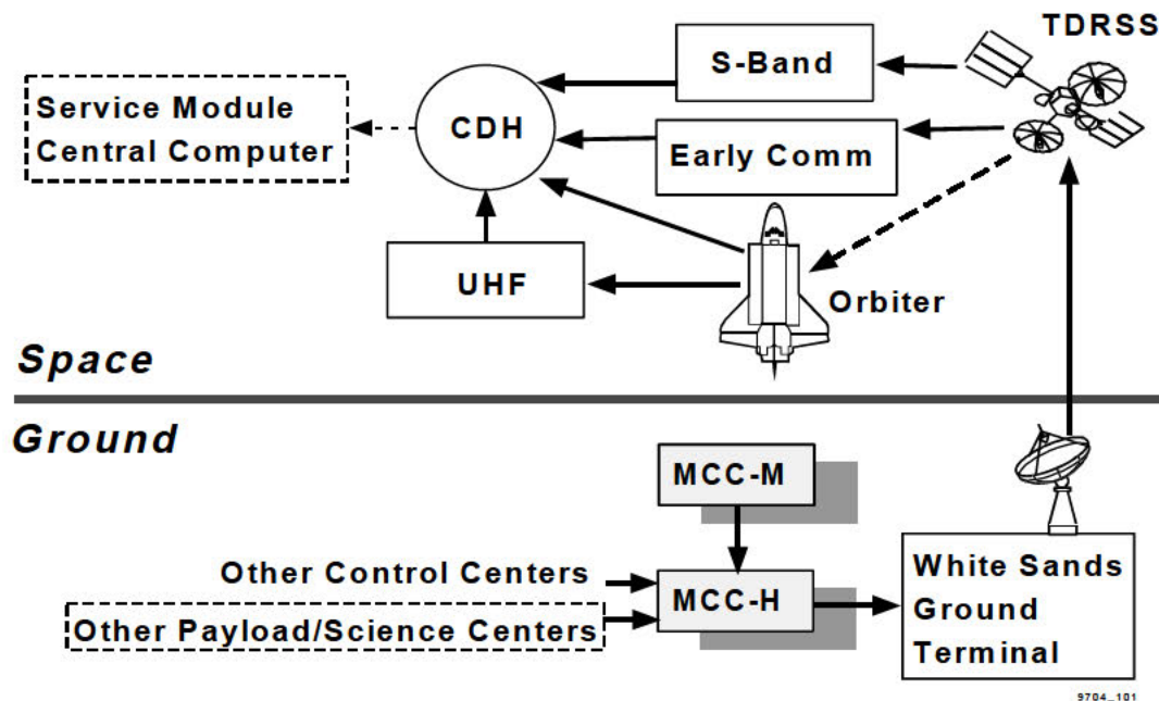
Figure 4-2. USOS command paths
