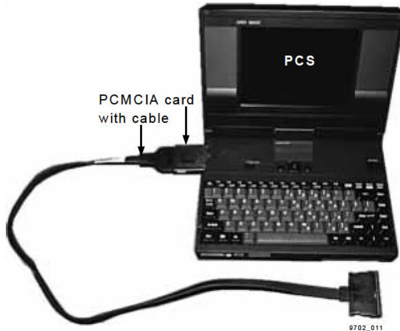
Figure 12-4. Logic analyzer
