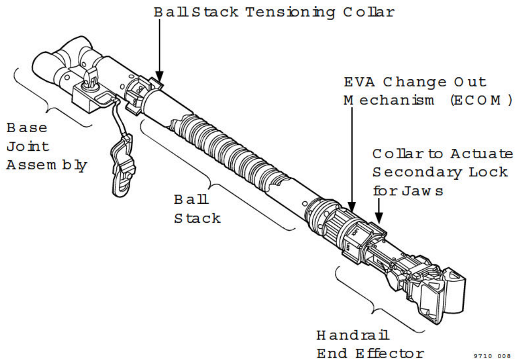
Figure 11-9. Multi-Use Tether
