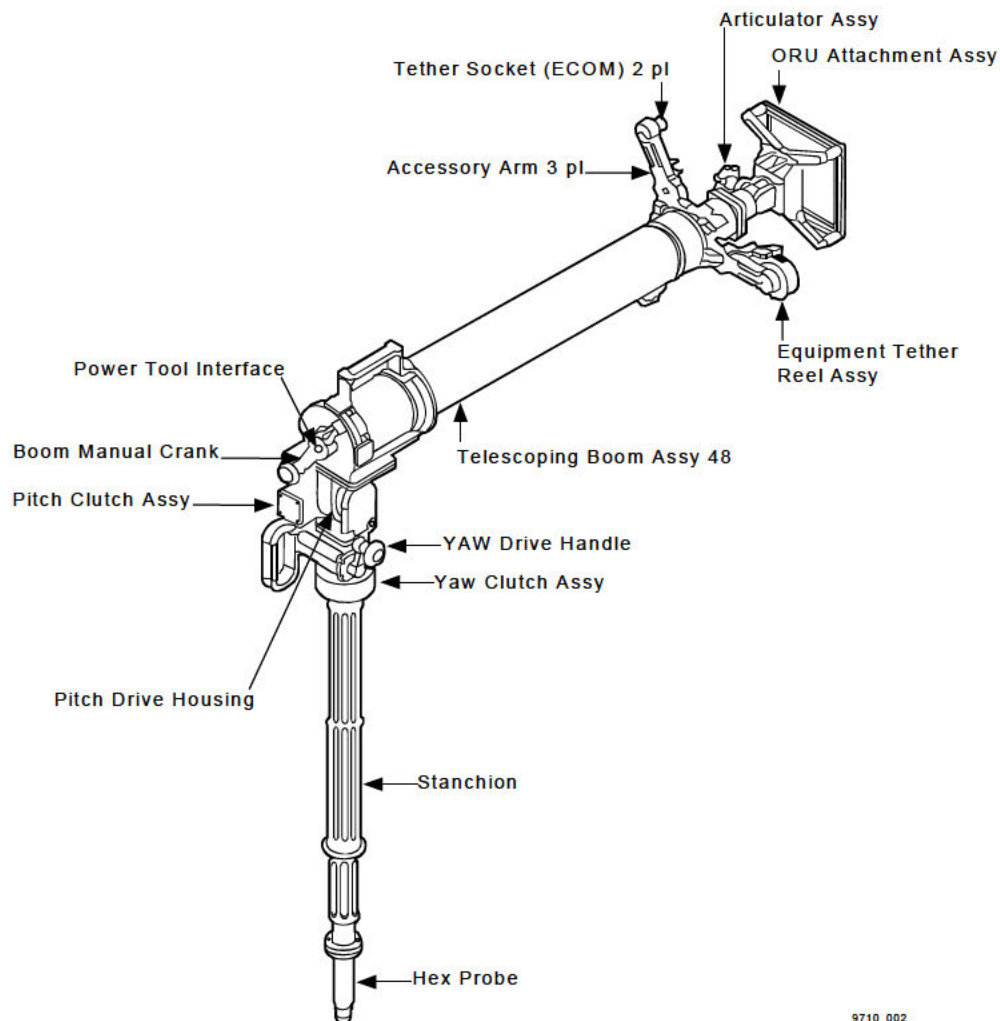
Figure 11-15. ORU transfer device (Crane)
