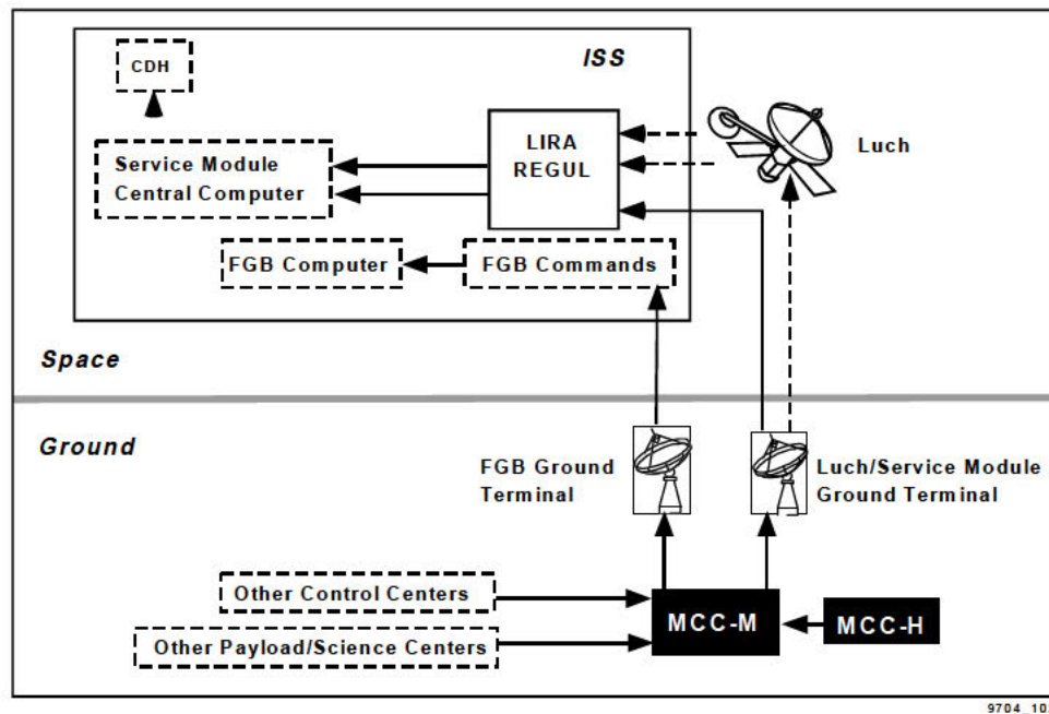
Figure 4-3. Russian Segment command path
