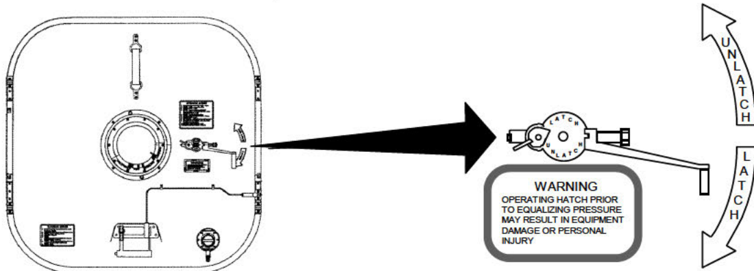
Figure 13-17. Hatch decal
