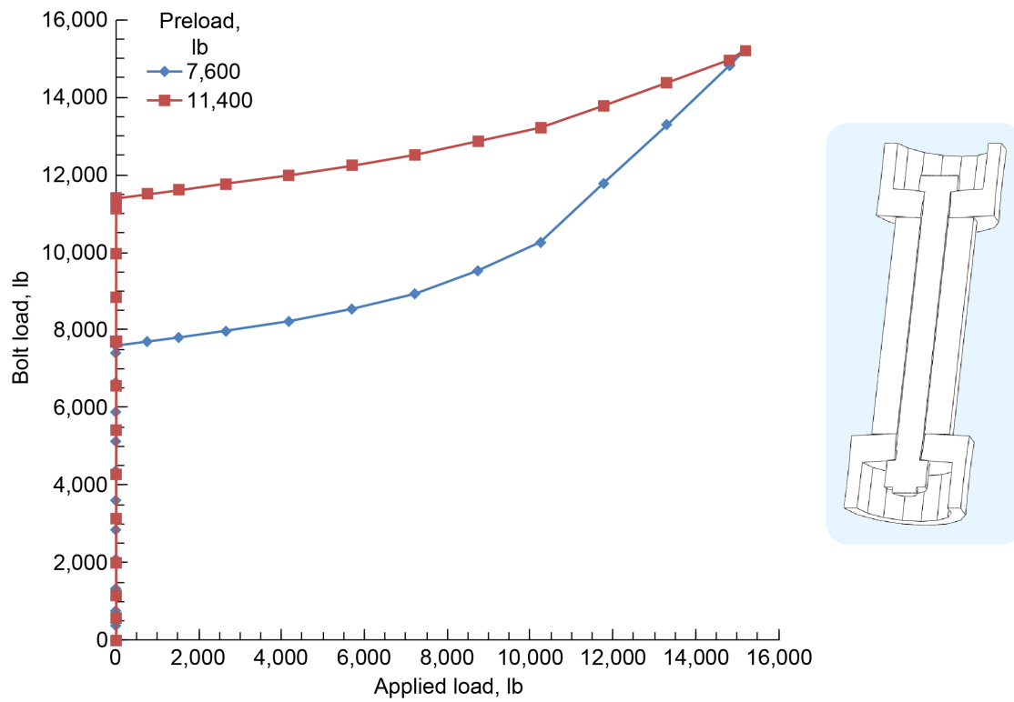
Figure G.5.—Bolt-load trajectories for PBJ as function of preload variation.
