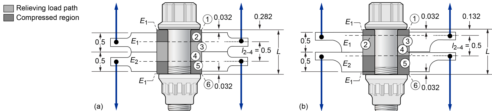
Figure 15.—Comparison of GLIF and SBLIF for PBJ, using cylindrical compression zone. Through-hole diameter is 0.25 in., bolt head and nut contact area diameter is 0.375 in., and moduli E_1 = 29 \times 10^6 psi, and E_2 = 10 \times 10^6 psi. (a) Relieving load path is centered within clamped members. (b) Relieving load path is offset closer to bolt head.
