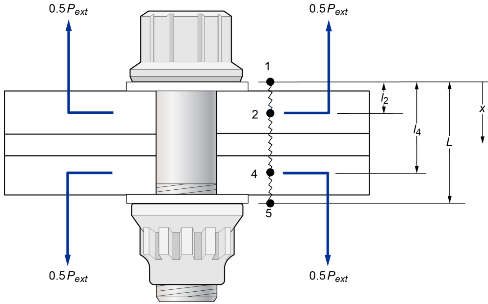
Figure 13.—Loading planes located at points 2 and 4. Points 1, 2, 4, and 5 correspond to those of Figure 8.
