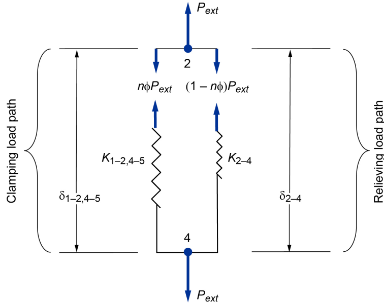
Figure J.5.—Stiffness representation of PBJ, indicating displacement and load being reacted by clamping and relieving load paths after preload.
