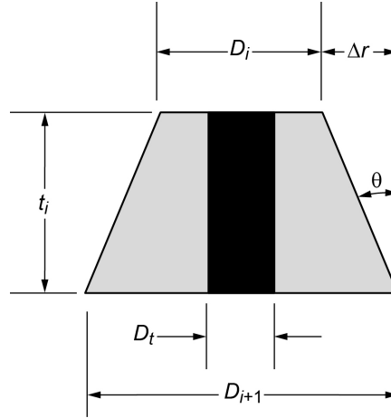
Figure C.3.—PBJ frustum element, i .
