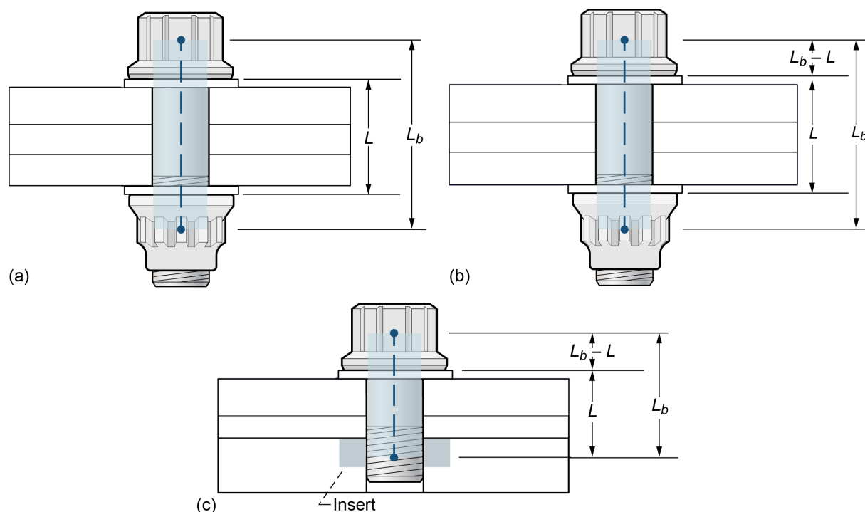
Figure E.2.—PBJ showing effective length of bolt L_b and thickness of clamped members L . (a) Bolt head and nut (internal threaded component) are not included as part of clamped members. (b) Part of nut (internal threaded component) is included as part of clamped members. (c) Part of insert (internal threaded component) is included as part of clamped members.
