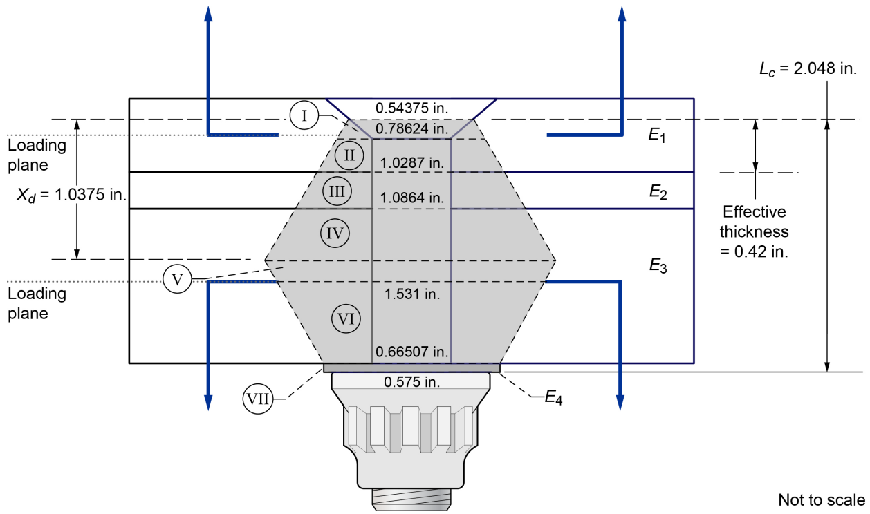
Figure C.2.—PBJ frustum stiffness elements I to VII arranged in series to form compression zone of thickness L_c with maximum diameter located at X_d .
