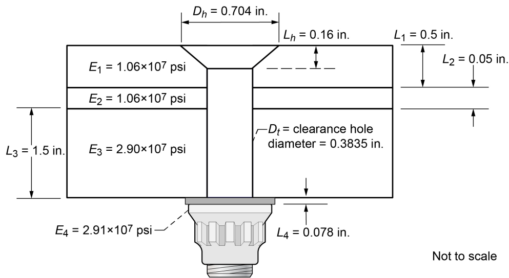
Figure C.1.—PBJ detail.
