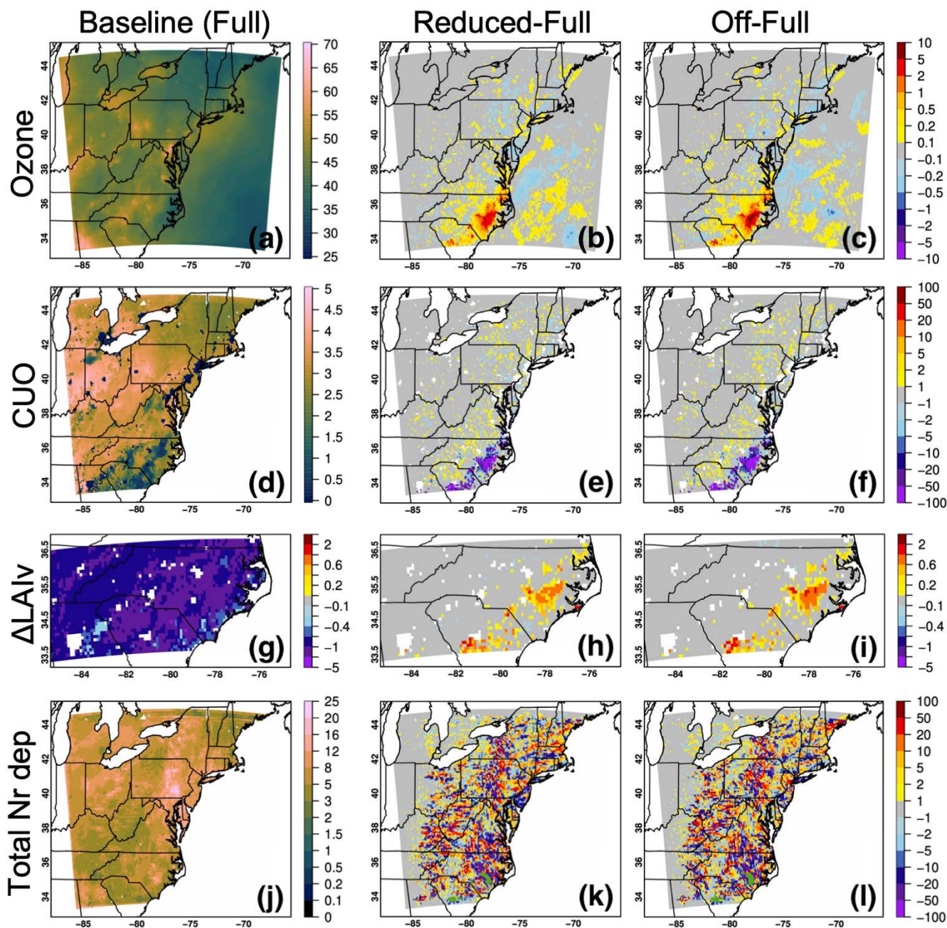
Figure 15: (a) Daytime surface O_3 concentration (ppbv, with the RMSE relative to AQS data of \sim 5.6 ppbv); (d) period-cumulated O_3 stomatal uptake ( \text{mmol m}^{-2} ); (g) O_3 impacts on leaf biomass (%) over irrigated areas in/around the Carolinas; and (h) total Nr deposition overland ( \text{kgN ha}^{-1} \text{a}^{-1} ) from the baseline simulation during 21–30 June 2022, and (b;c;e;f;h;i;k;l) their sensitivities to adjustments in irrigation schemes. Sensitivity results are in ppbv for surface O_3 concentration, and in % for all other plots. Green areas in (k;l) marked the grids where Student's t -tests comparing Nr deposition from the baseline and sensitivity simulations gave smaller-than-0.05 p values.
