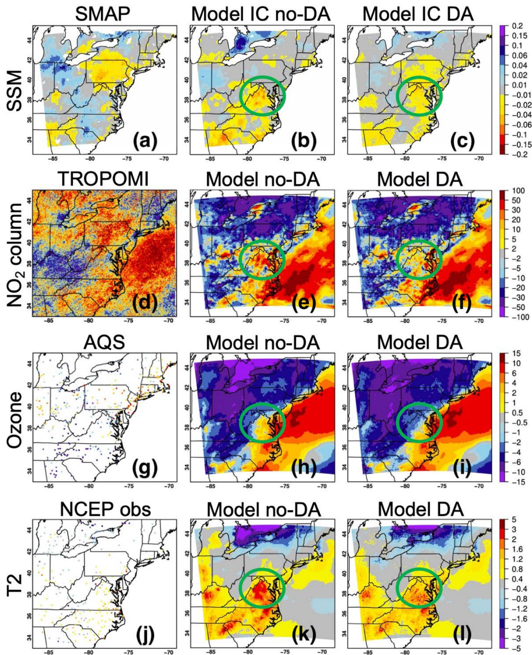
1310 Figure 14: July 2022-July 2018 monthly differences in (a–c) SSM ( \text{m}^3 \text{m}^{-3} ) indicated by bias-corrected SMAP, free-running and SMAP-constrained WRF-Chem initial conditions (ICs); (d–f) early afternoon NO 2 columns (%) based on TROPOMI, free-running and SMAP-constrained WRF-Chem results; (g–i) daytime surface O 3 concentrations (ppbv) based on AQS observations, free-running and SMAP-constrained WRF-Chem results; and (j–l) daytime surface air temperature (K) based on the National Centers for Environmental Prediction (NCEP) Surface Observational Weather Data product, free-running and SMAP-constrained WRF-Chem results. Green circles highlight areas in/around Virginia where improvements in WRF-Chem land ICs notably improved the weather, NO 2 and O 3 fields. Additional information on the SMAP data assimilation (DA) impacts is included in Fig. S18.
