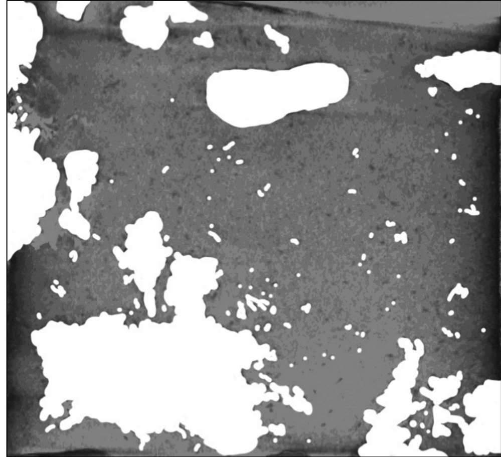
Main Core cross-section CT image with white masks applied to macro-pore locations used to calculate the pore area of each cross-section increment.
